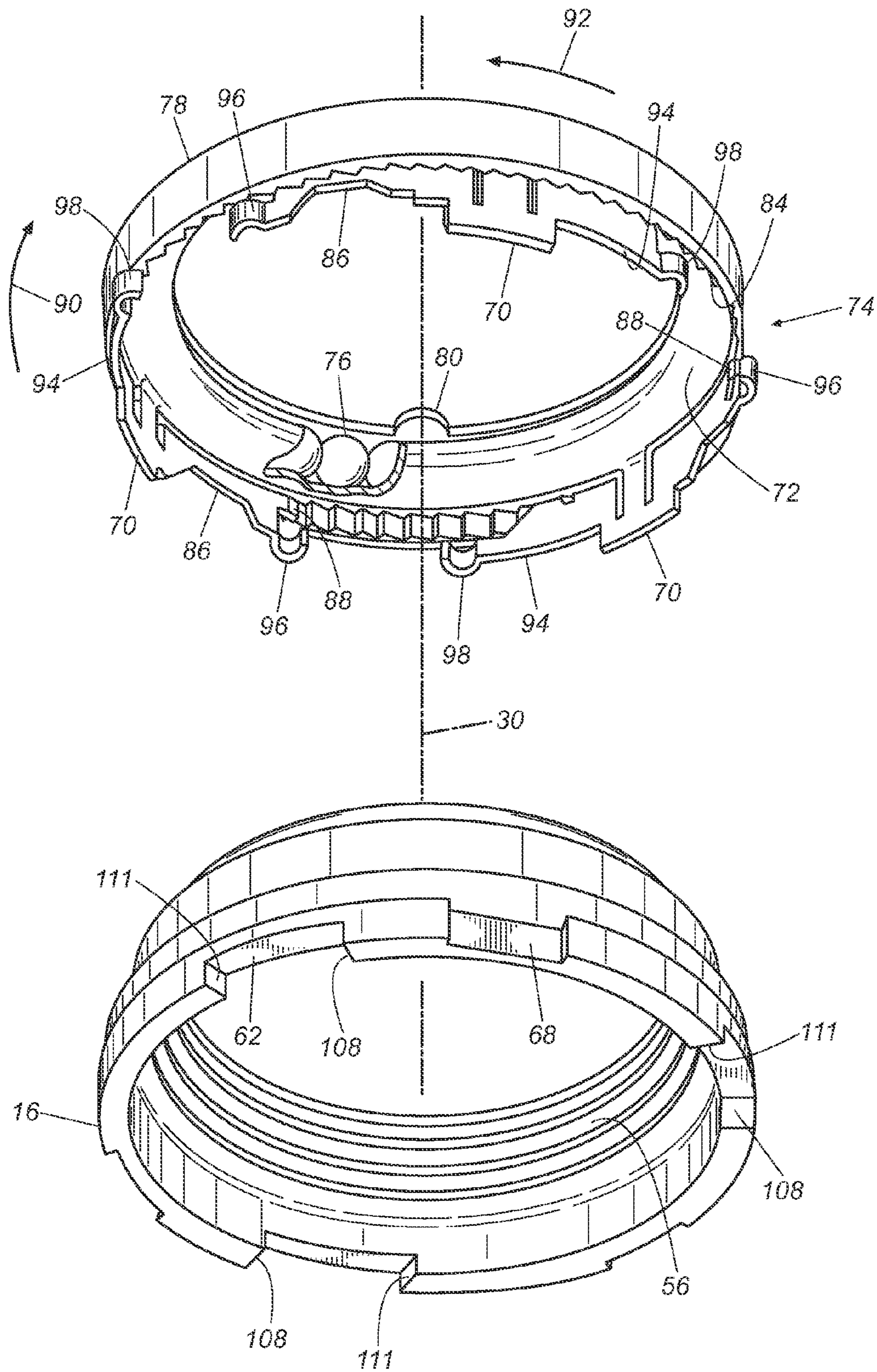
Fig. 3 (Prior Art)
