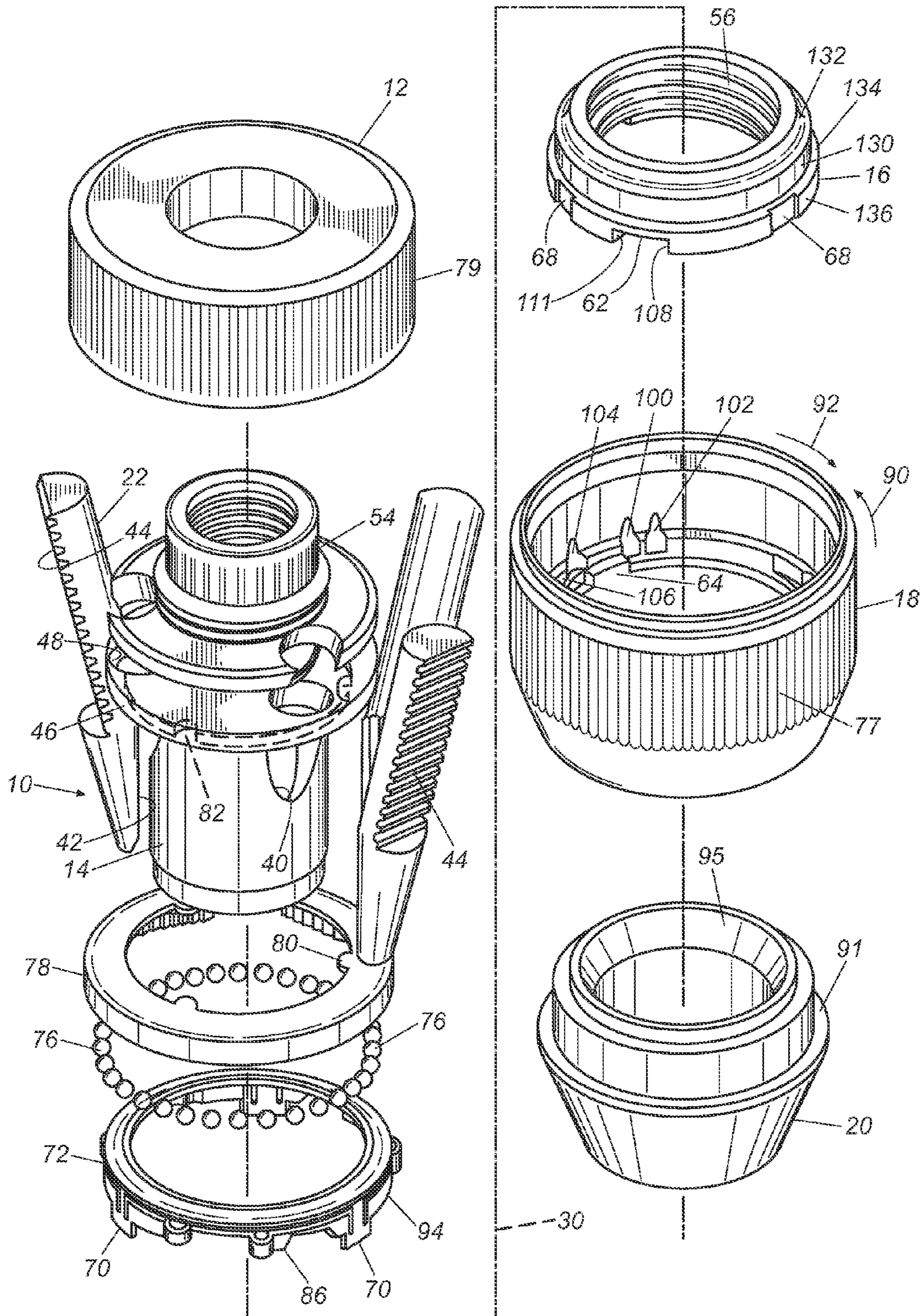
Fig. 2 (Prior Art)
