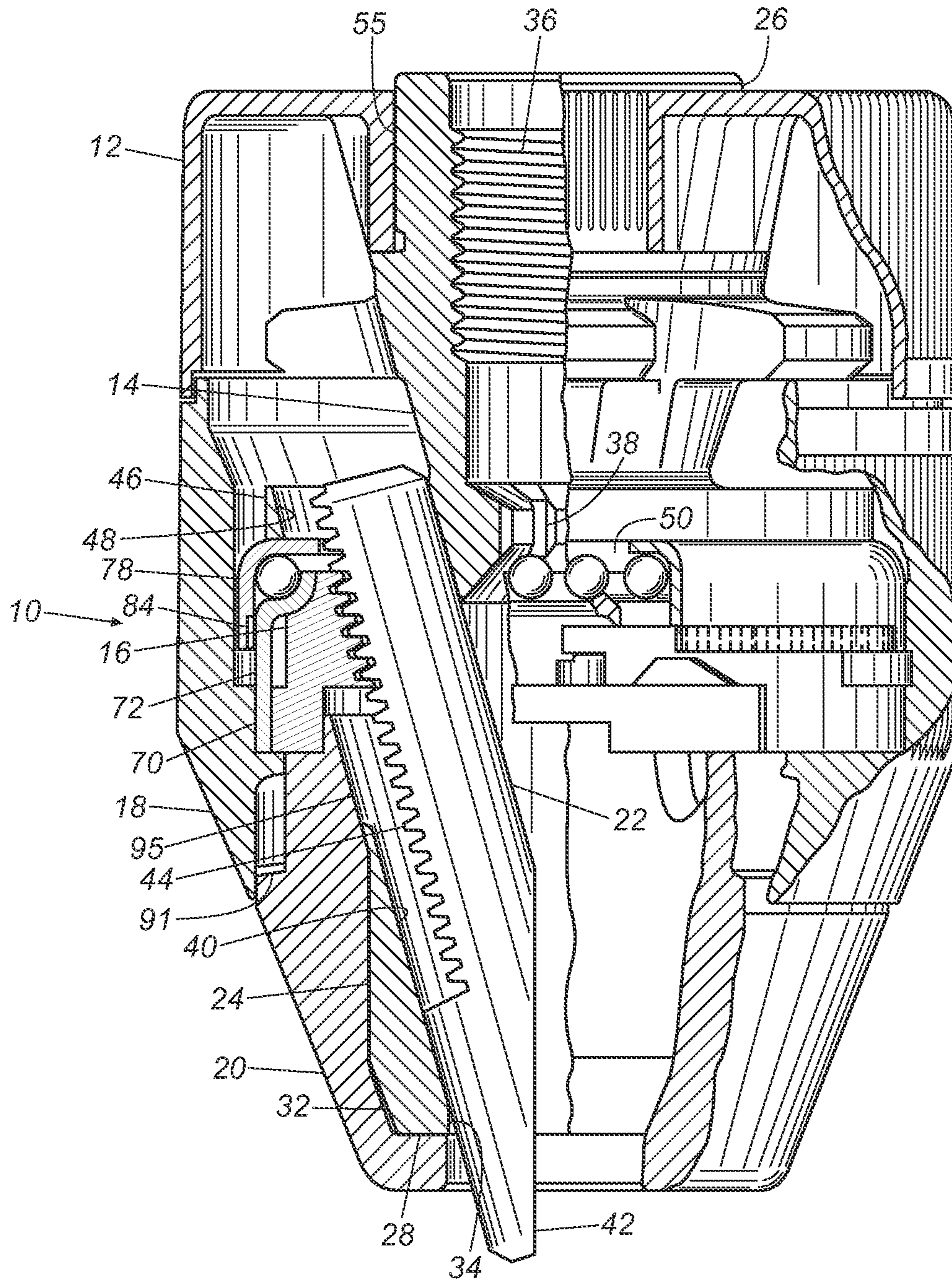
Fig. 1 (Prior Art)
