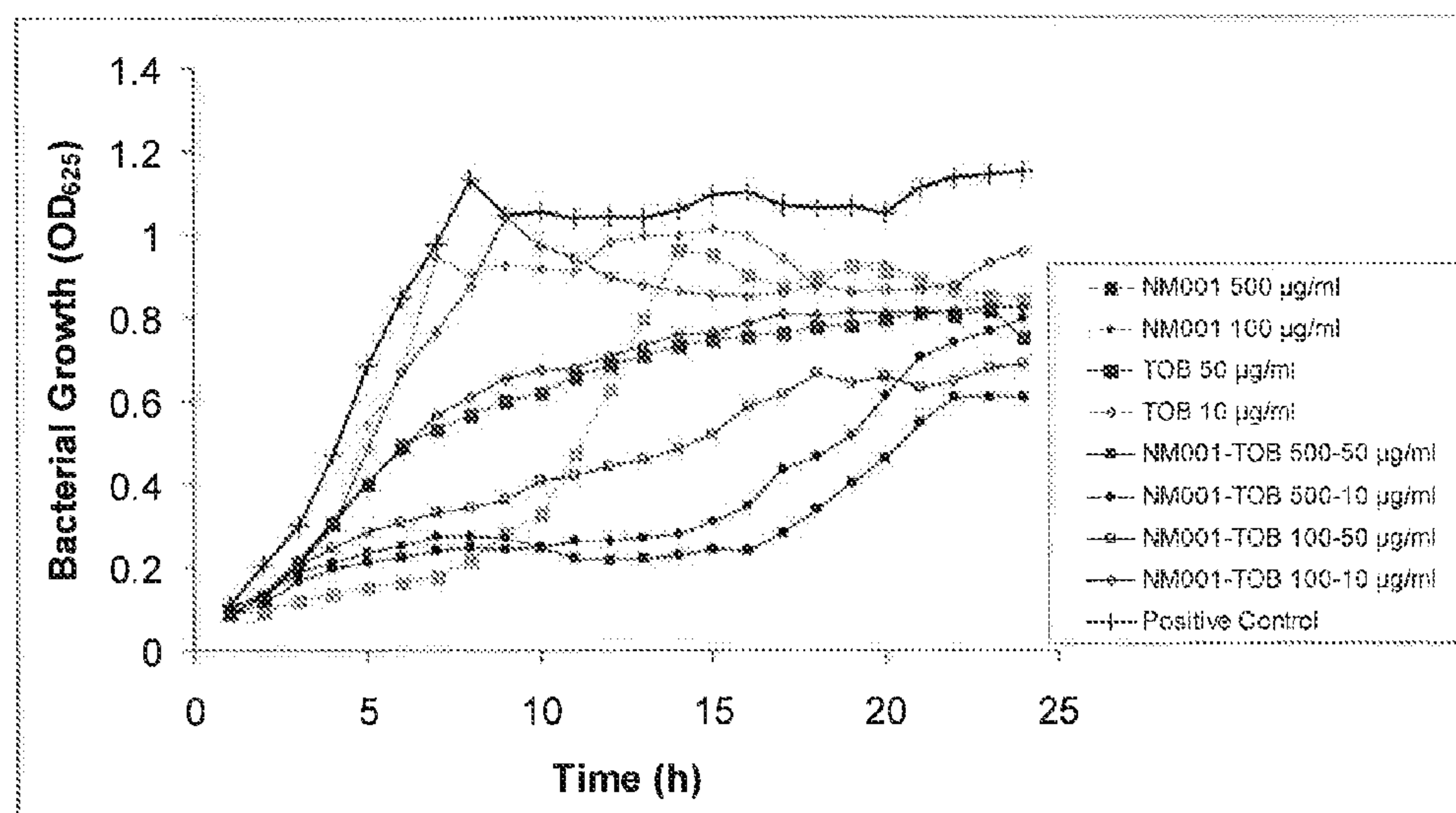
FIG. 5 Post-Antimicrobial Effect of Cysteamine (NM001) in Combination with Tobramycin (TOB) versus P. aeruginosa PAO1 biofilms
