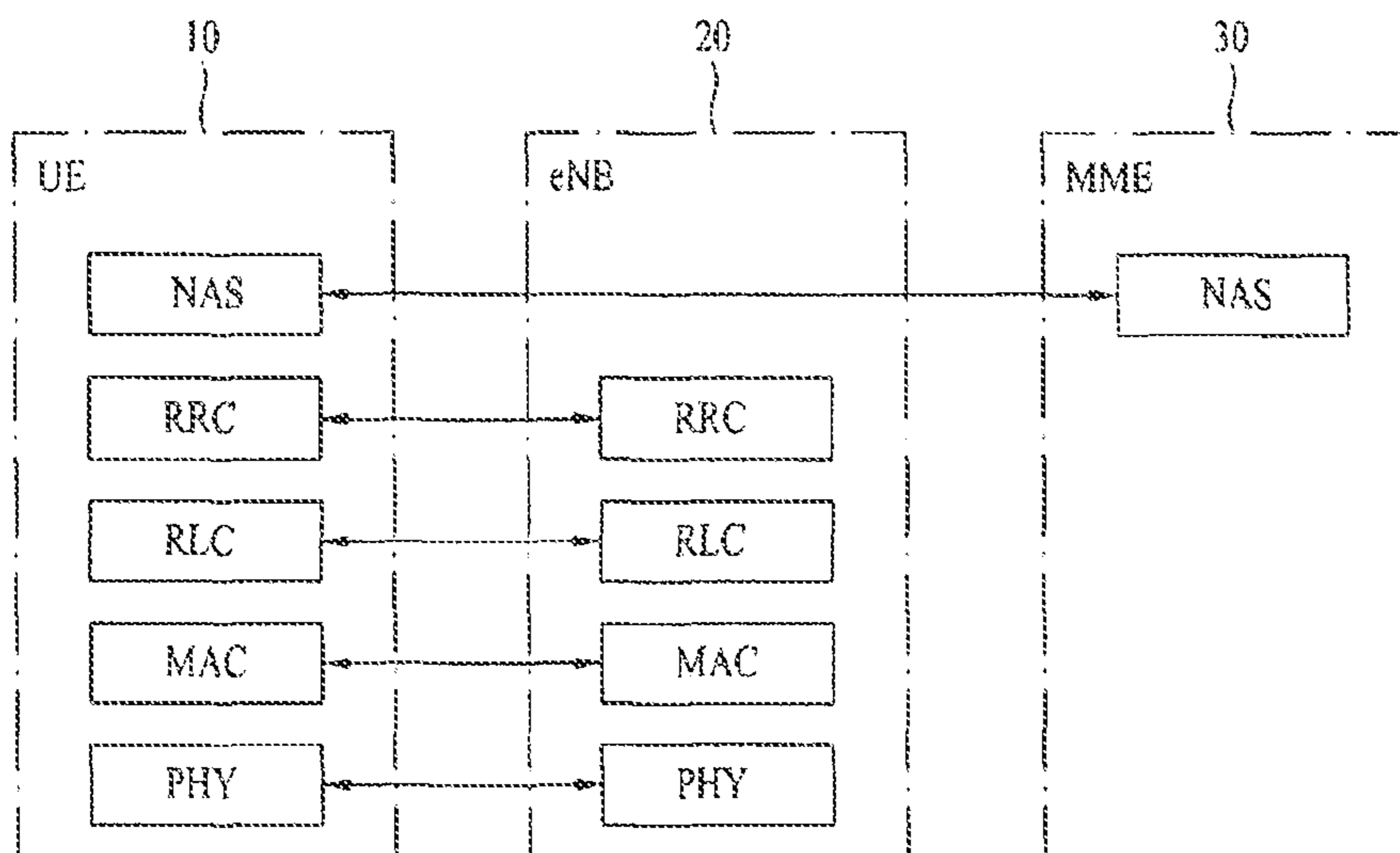
FIG. 2C (PRIOR ART)
