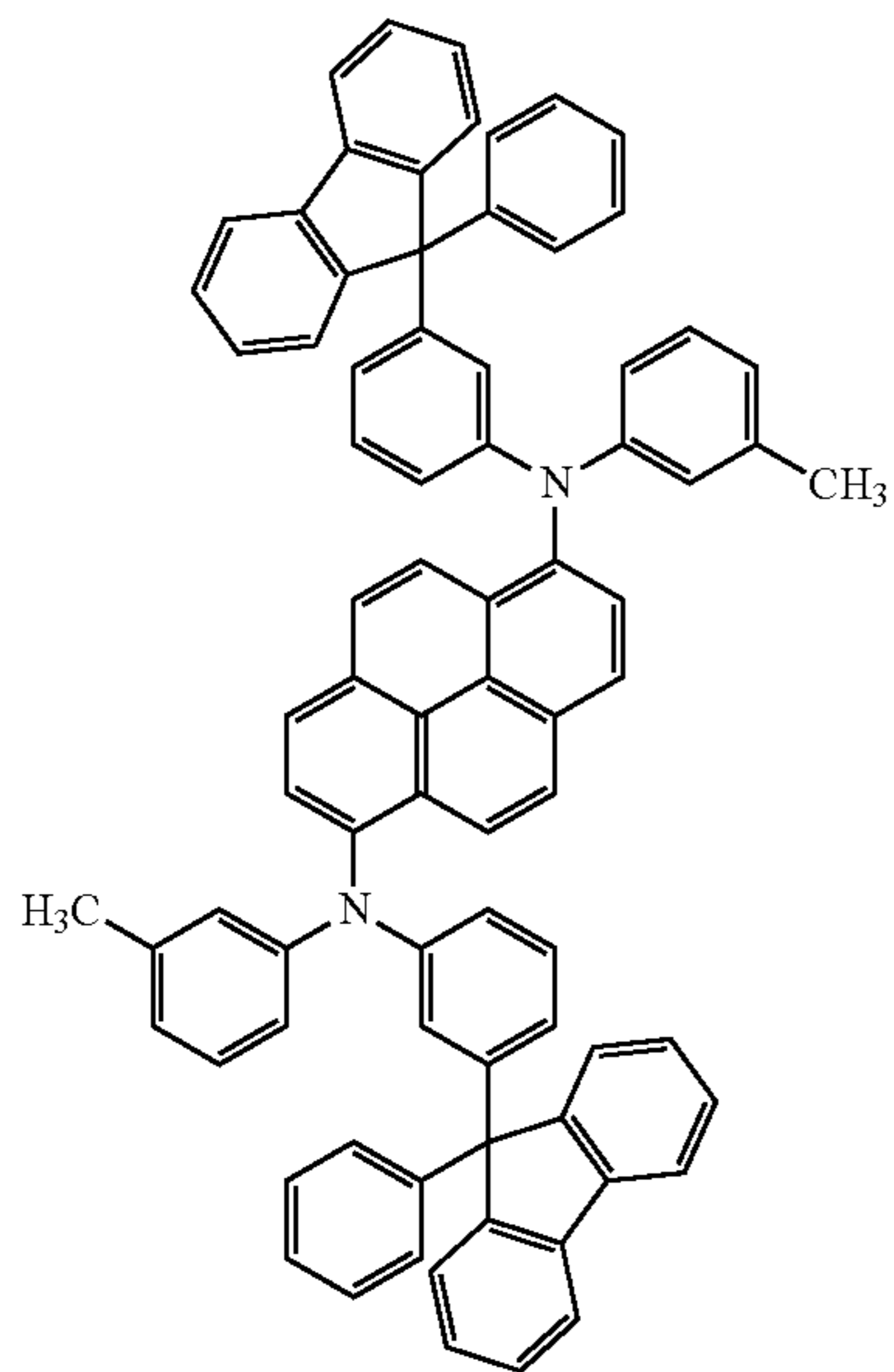
1,6mMemFLAPrn
