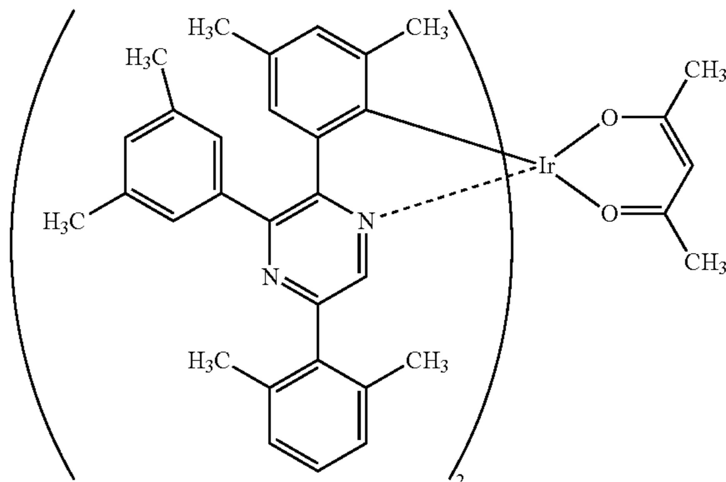
[Ir(dmdppr-dmp) 2 (acac)]
