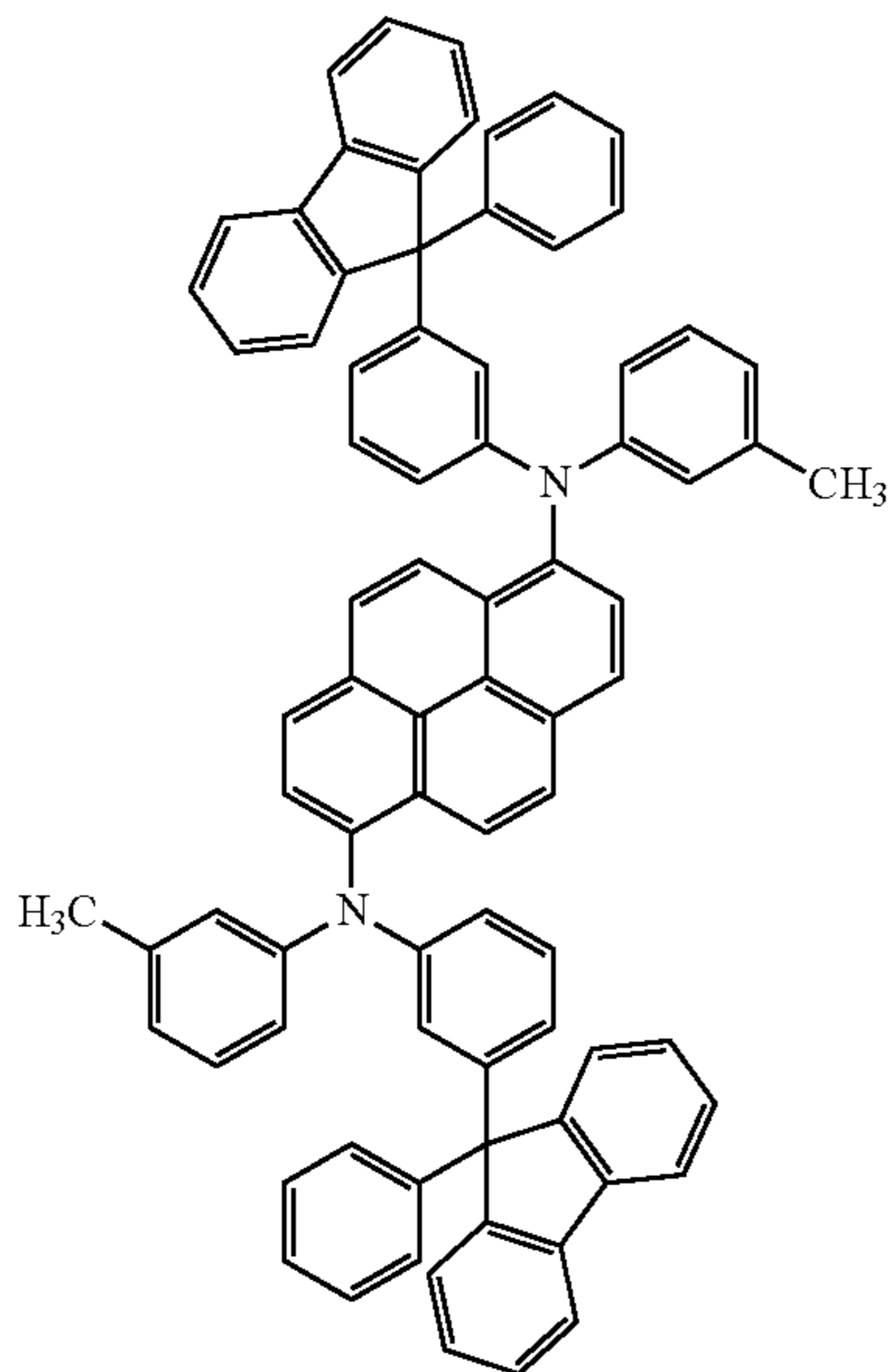
1,6mMemFLAPrn
