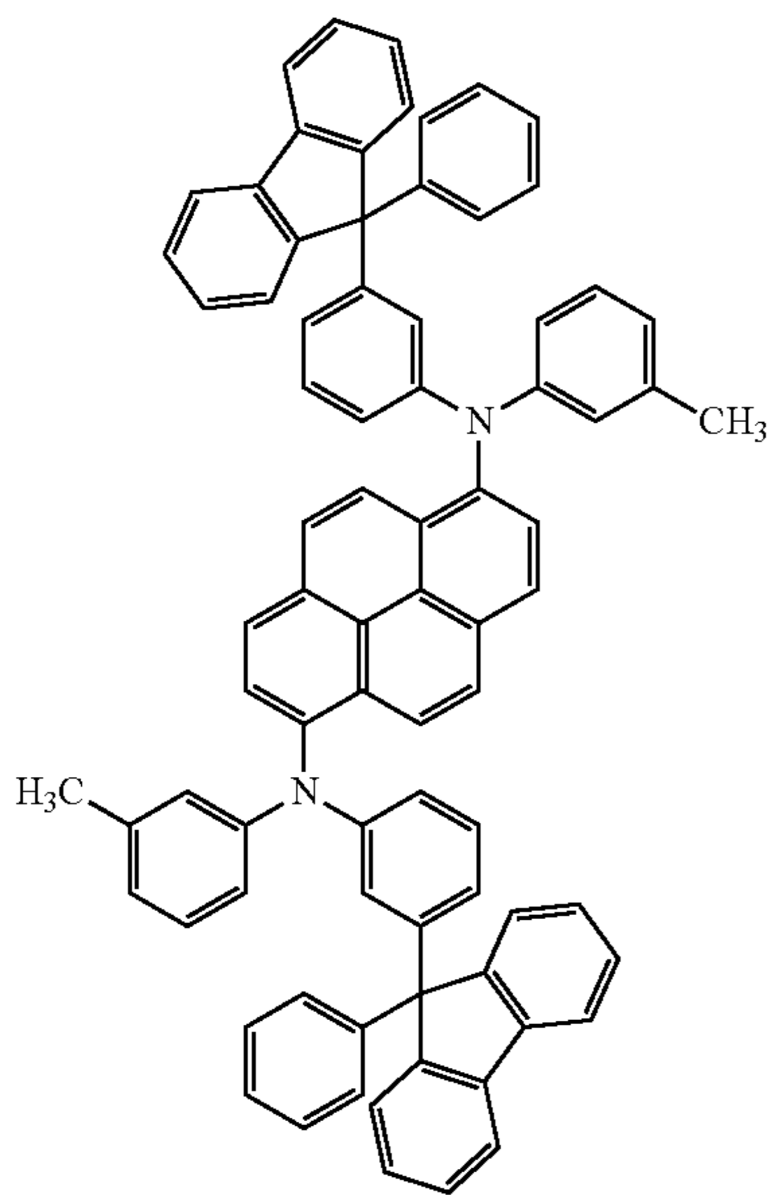
1,6mMemFLAPm
