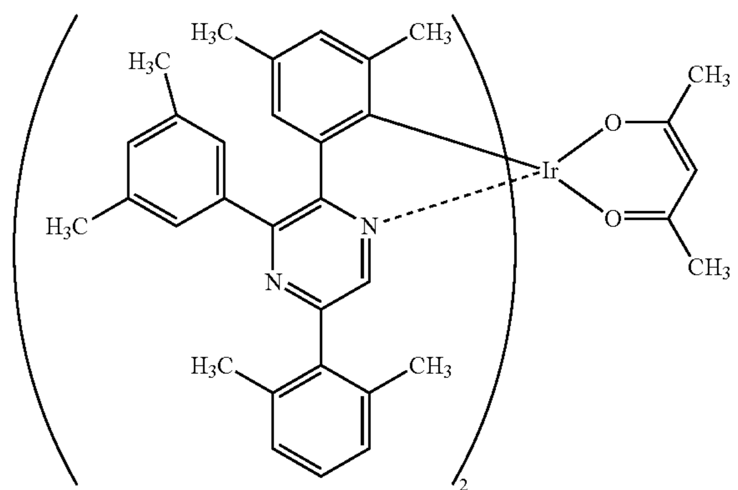
[Ir(dmdppr-dmp) 2 (acac)]
