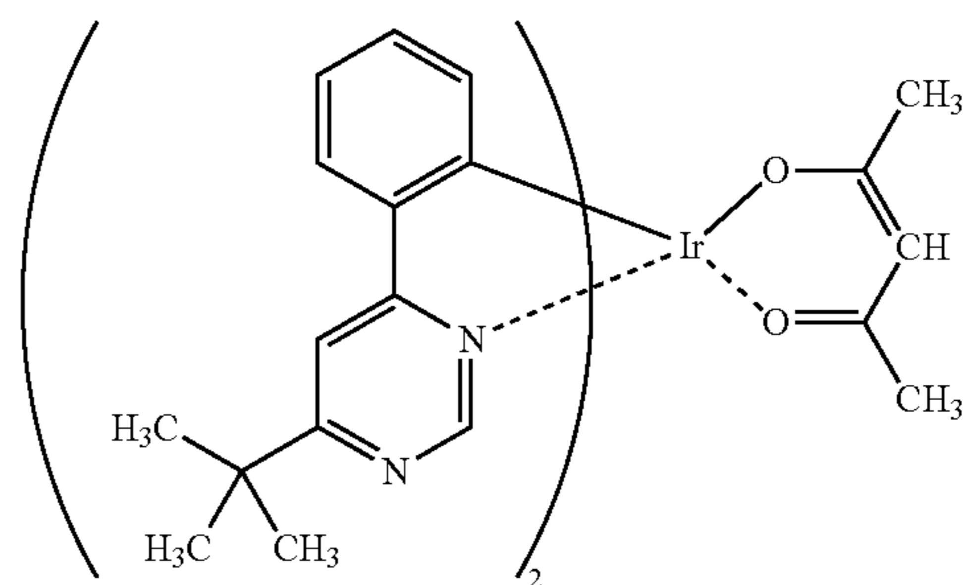
[Ir(tBuppm) 2 (acac)]
