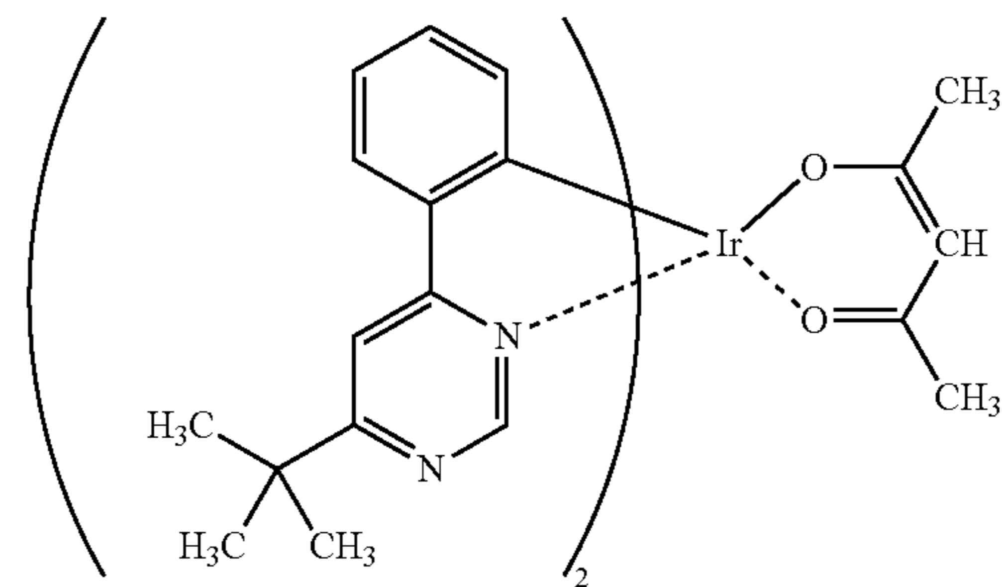
[Ir(tBuppm) 2 (acac)]
