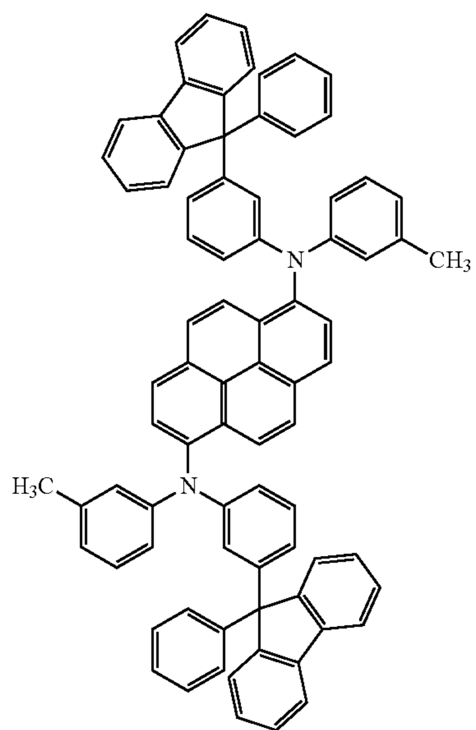
1,6mMemFLAPm
