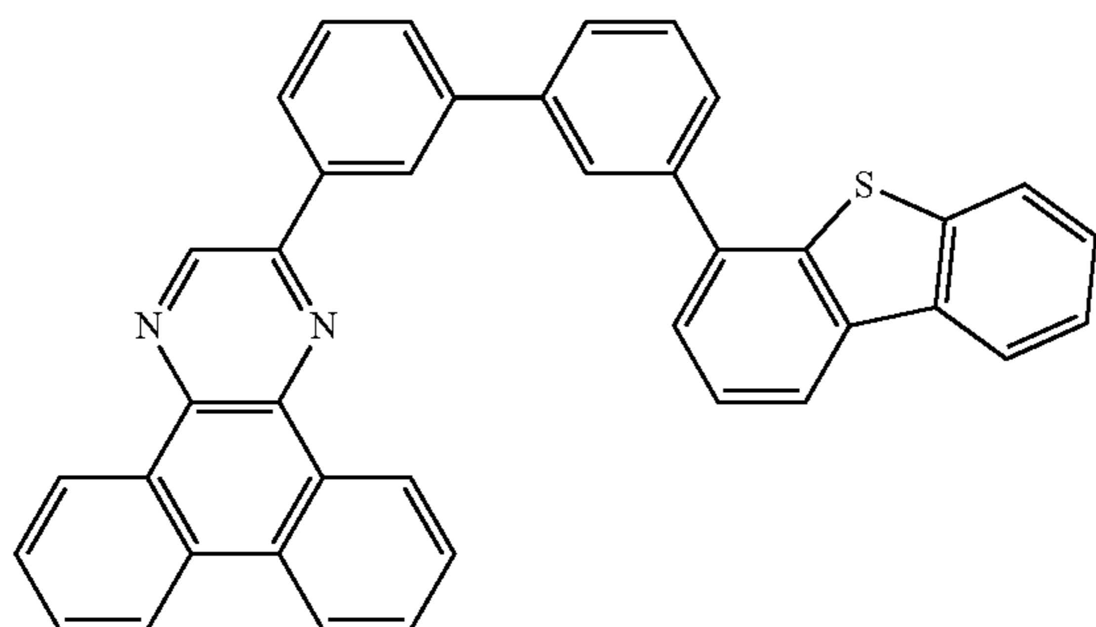
2mDBTBPDBq-II
