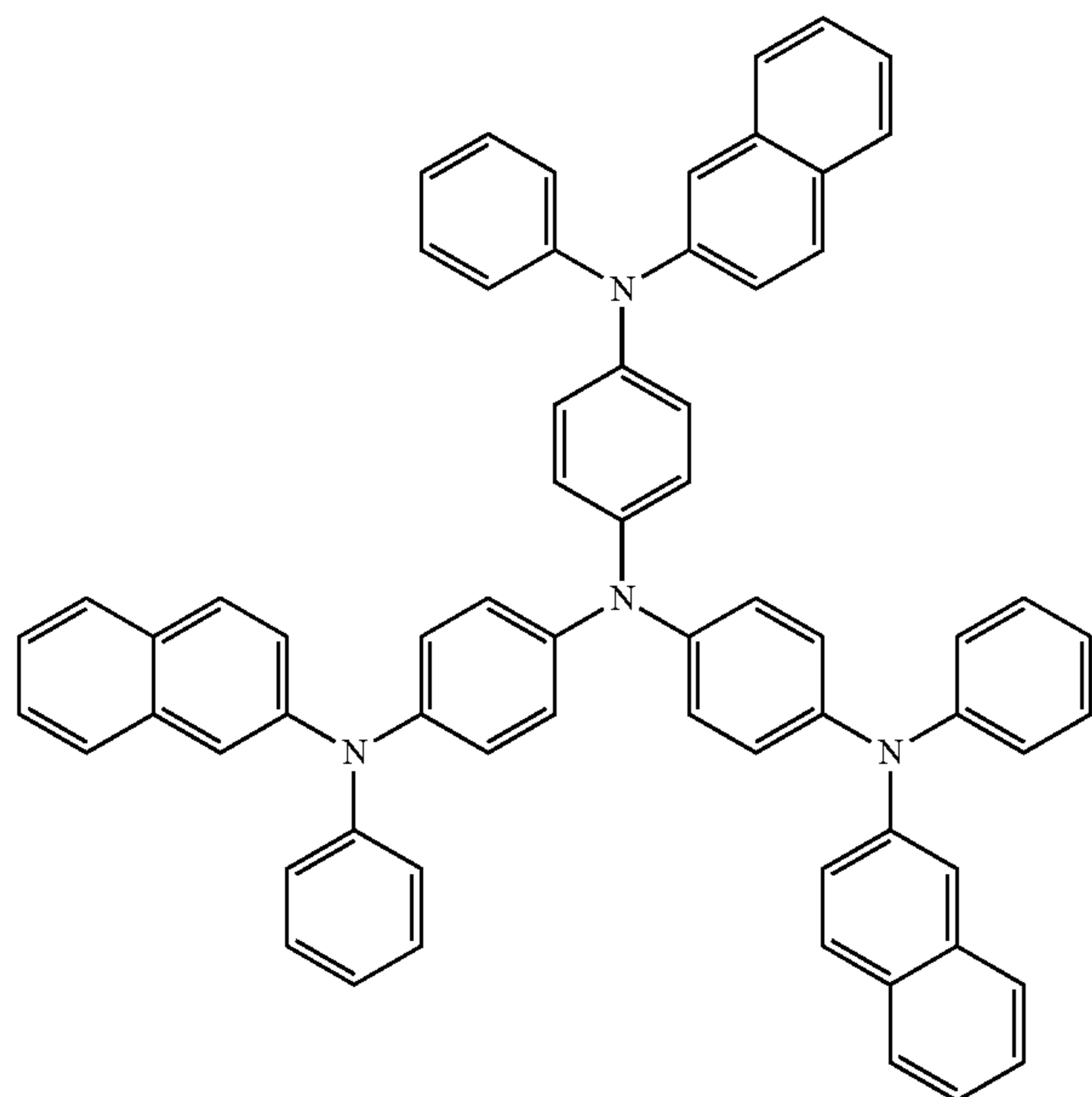
2-TNATA
