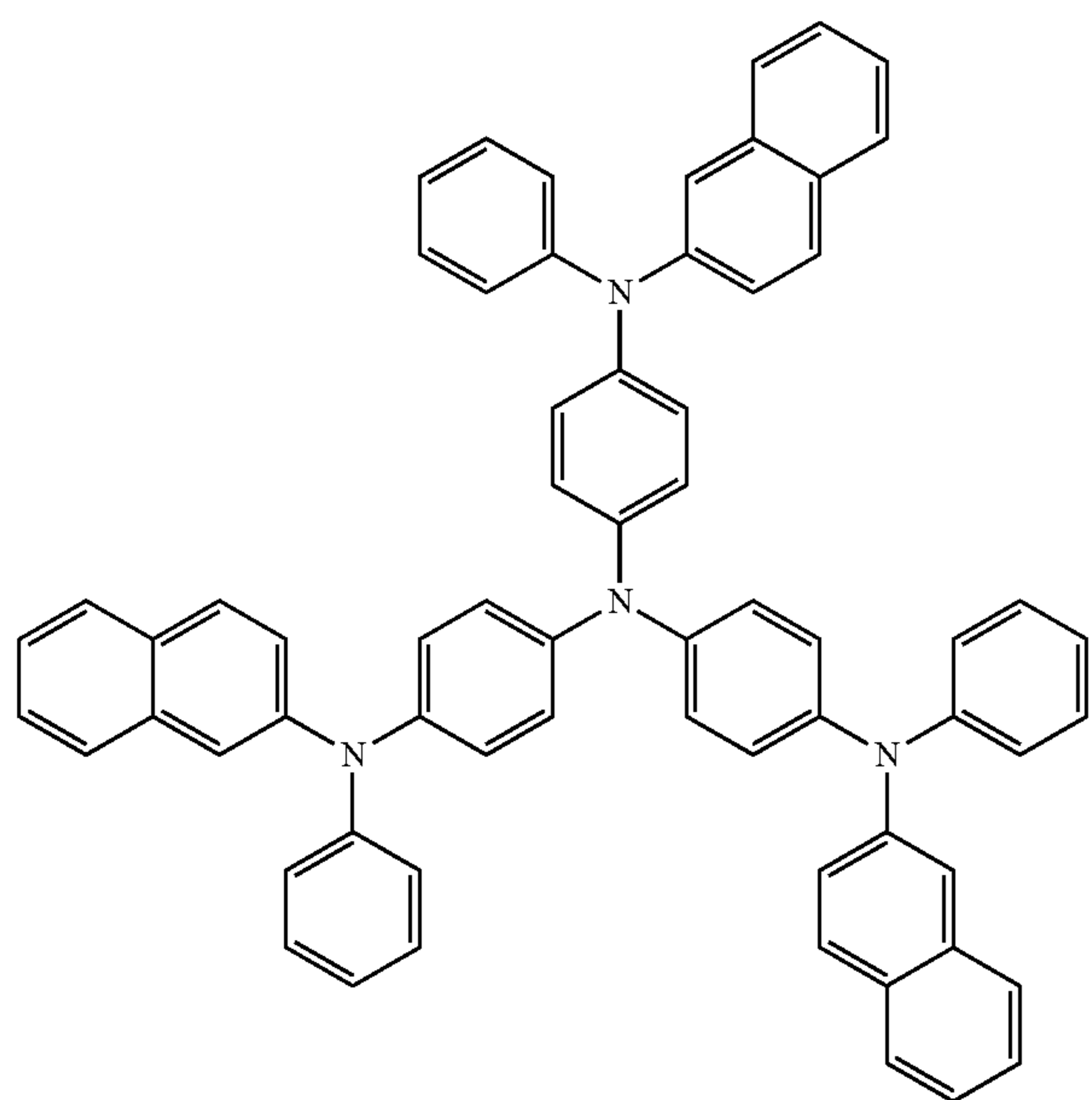
2-TNATA
