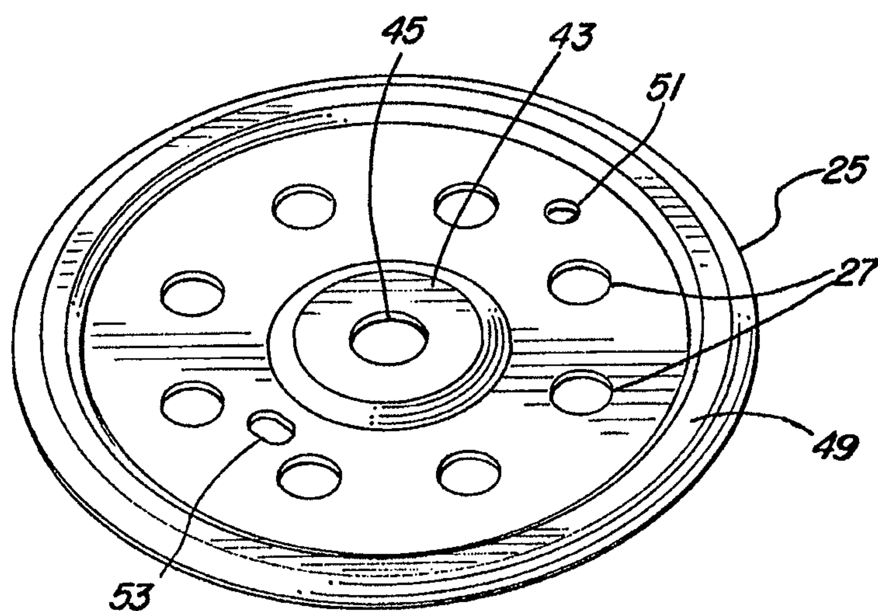
FIG. 4 PRIOR ART
