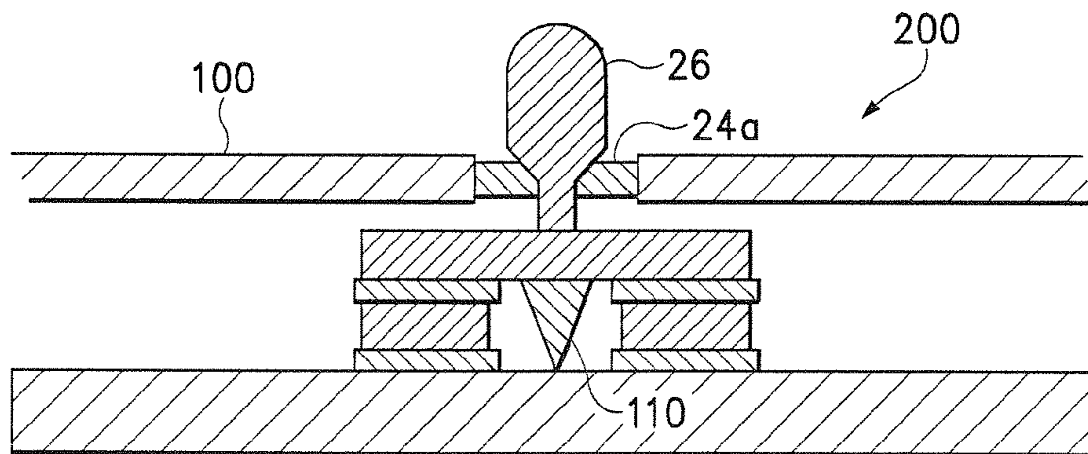
Figure 7 (CROSS-SECTION VIEW)
