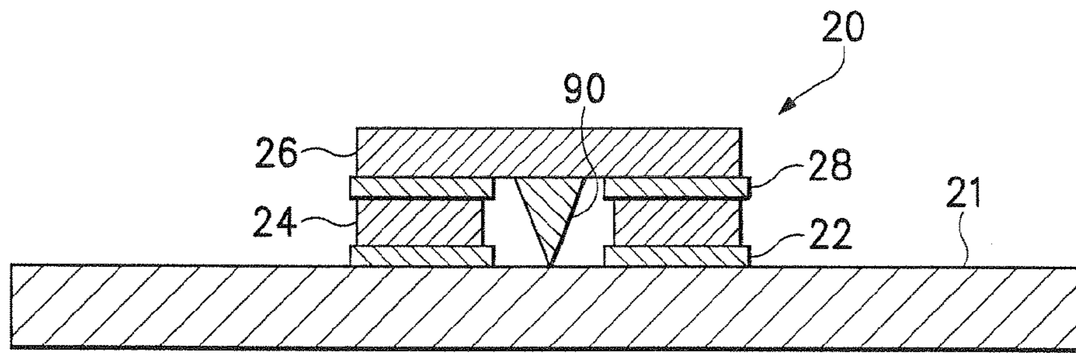
Figure 6 (CROSS-SECTION VIEW)
