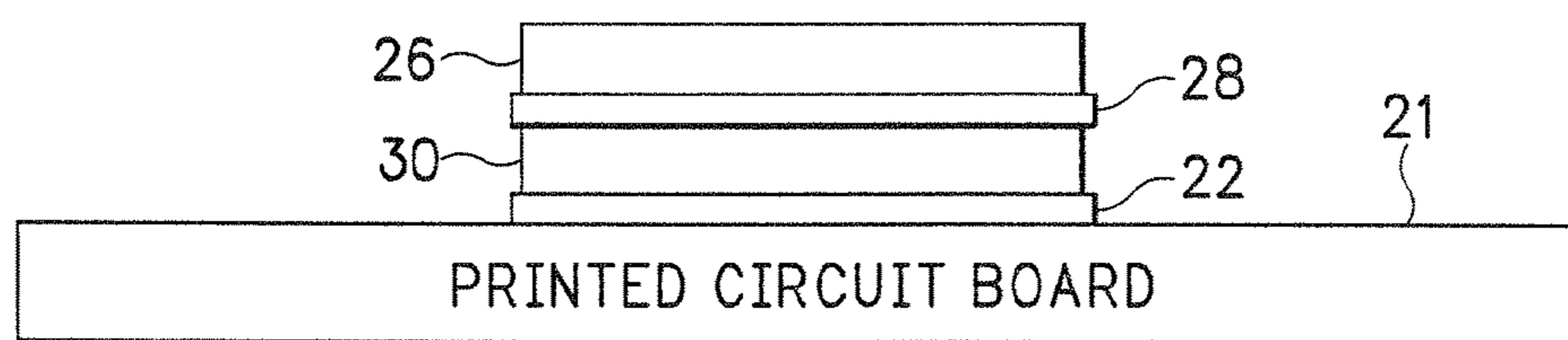
Figure 8 (SIDE VIEW)
