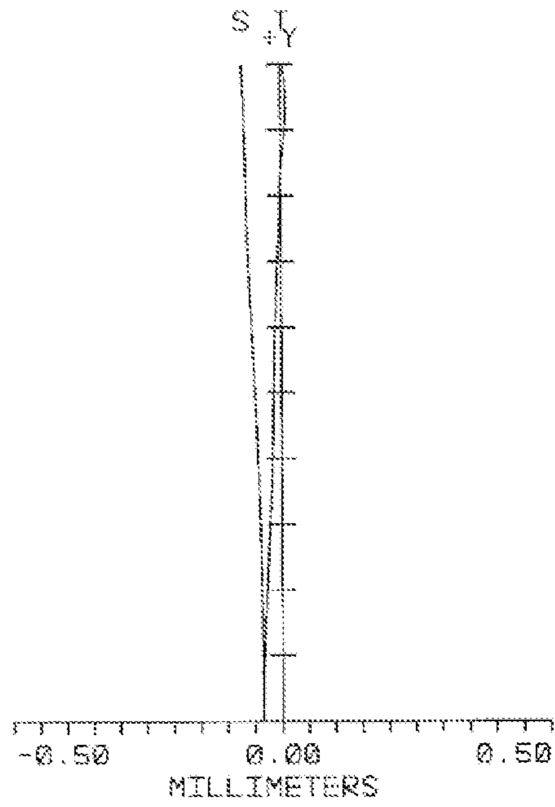
FIG. 6C FIELD CURVATURE
