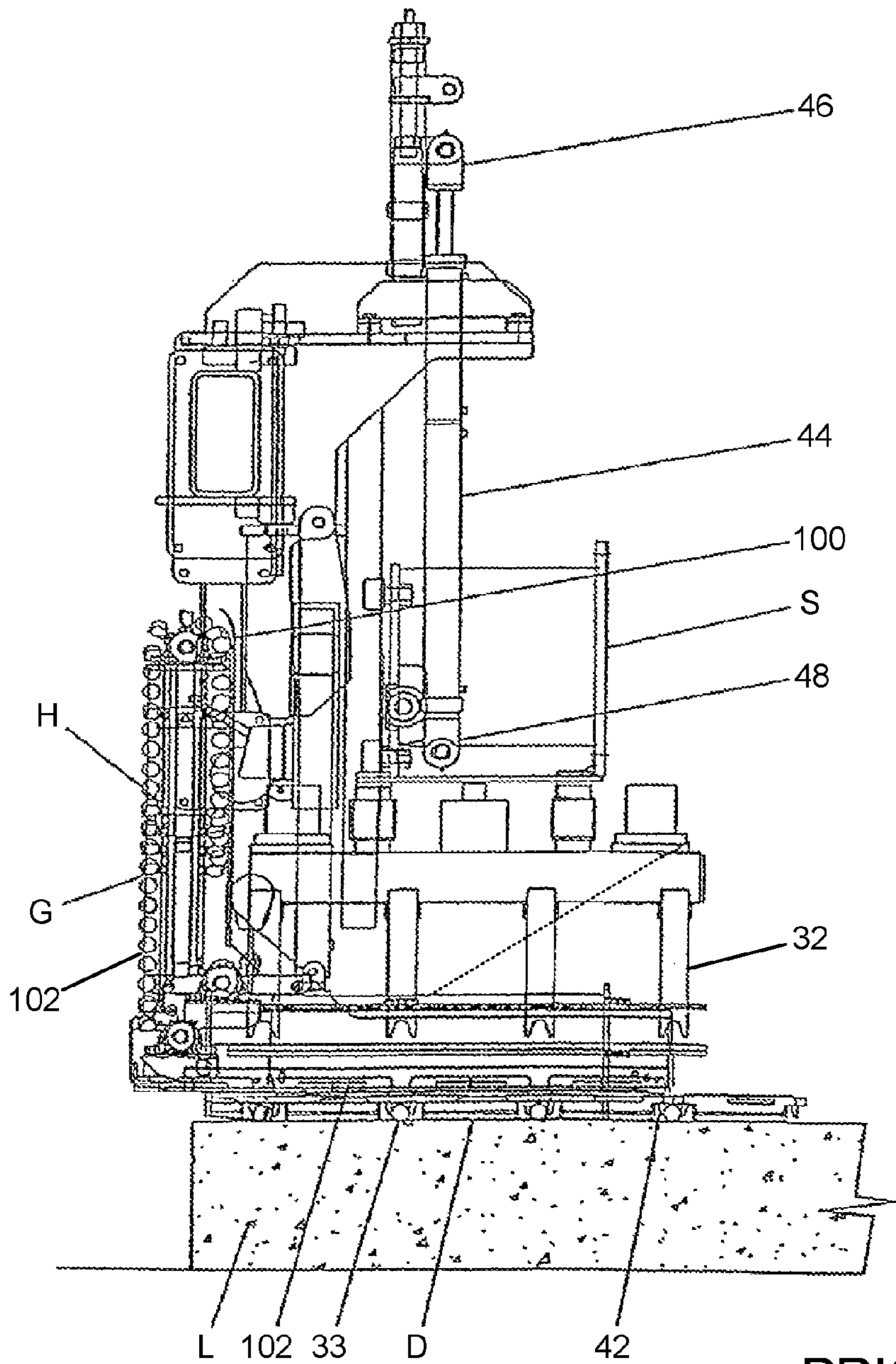
-- PRIOR ART -- FIGURE 3B
