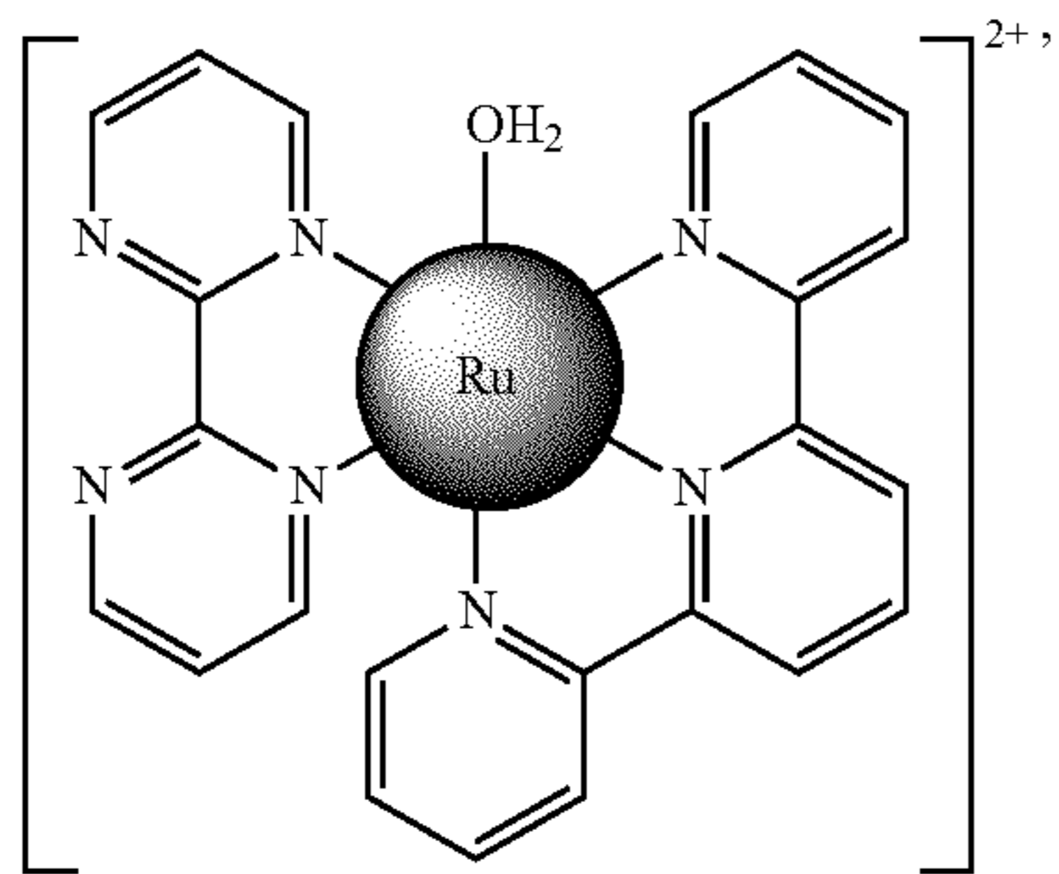
[Ru(tpy)(bpm)(OH_2)]^{2+} ,
