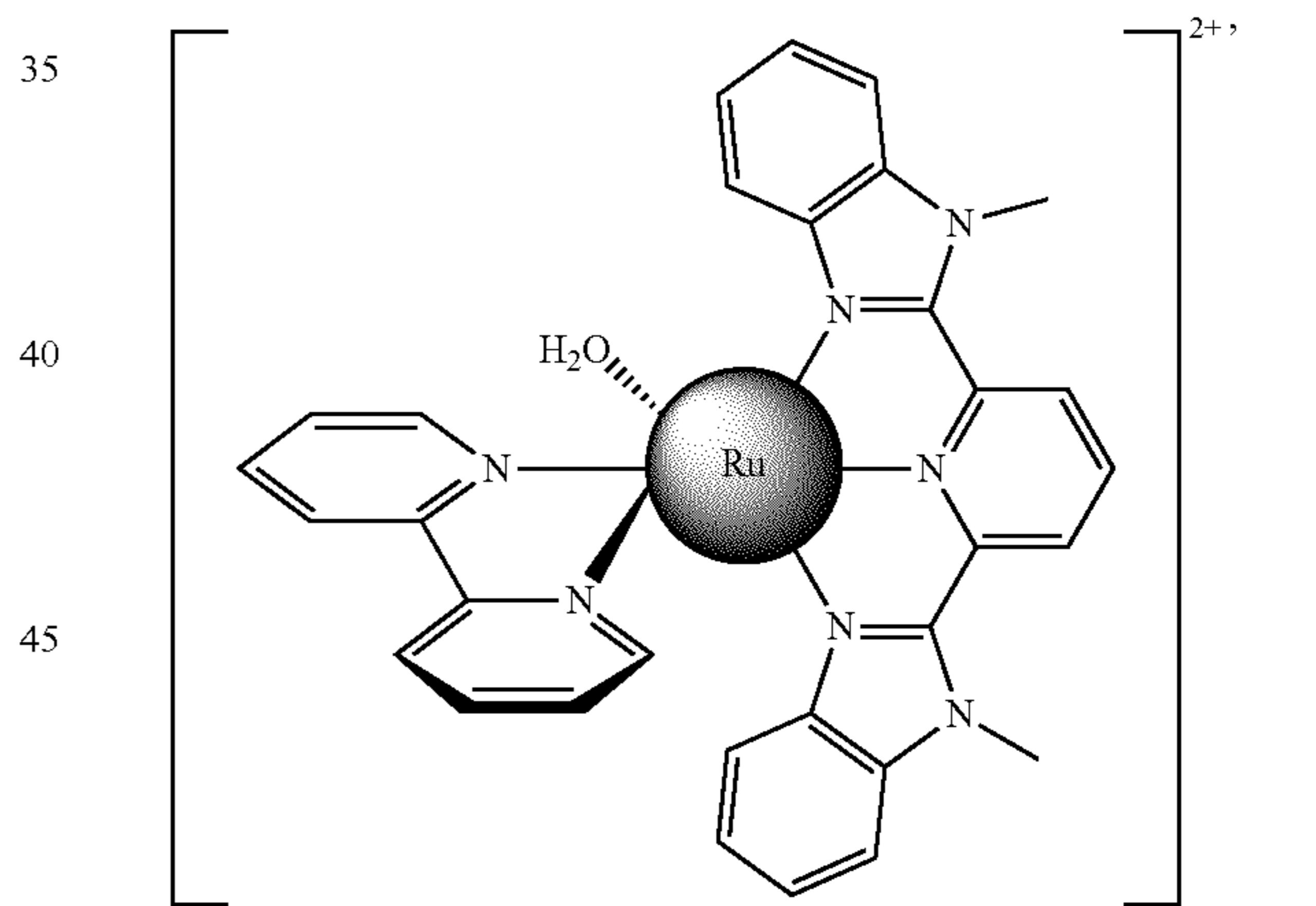
[Ru(Mebimpy)(bpy)(OH_2)]^{2+}
