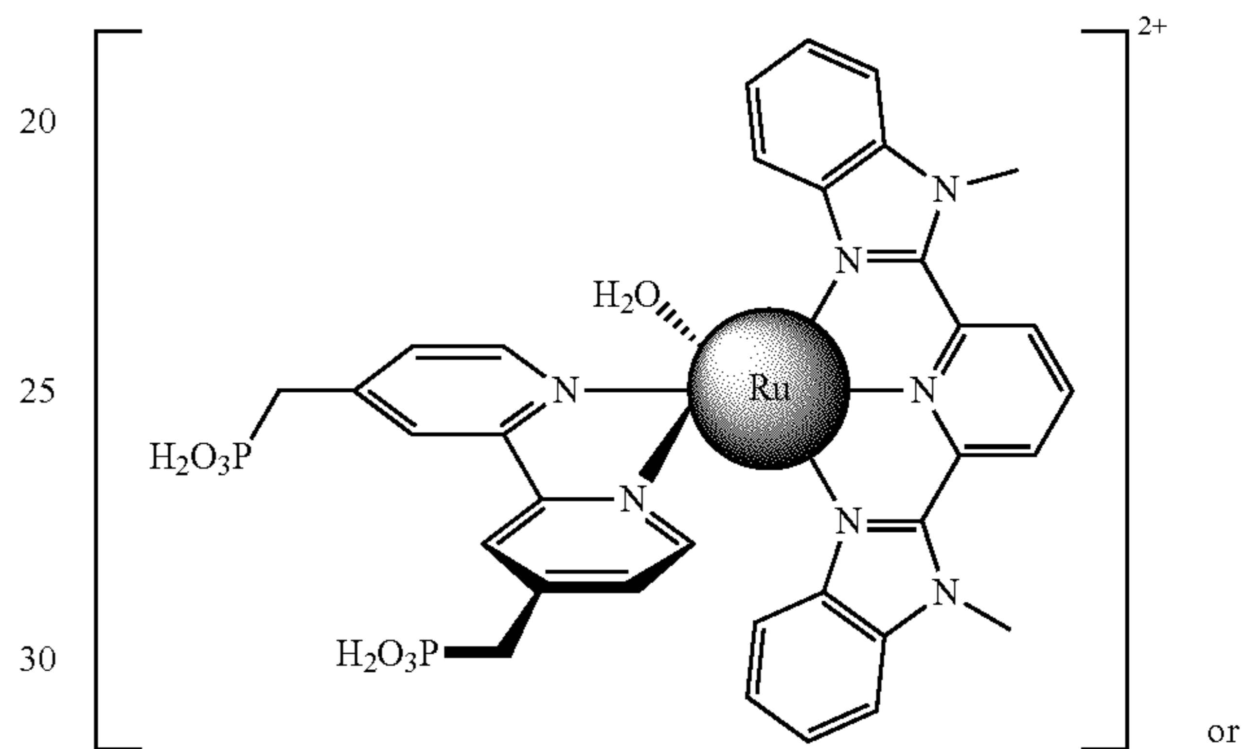
\{Ru(Mebimpy)[4,4'-((HO)_2OPCH_2)_2bpy](OH_2)\}^{2+} (1- PO_3H_2 ),
