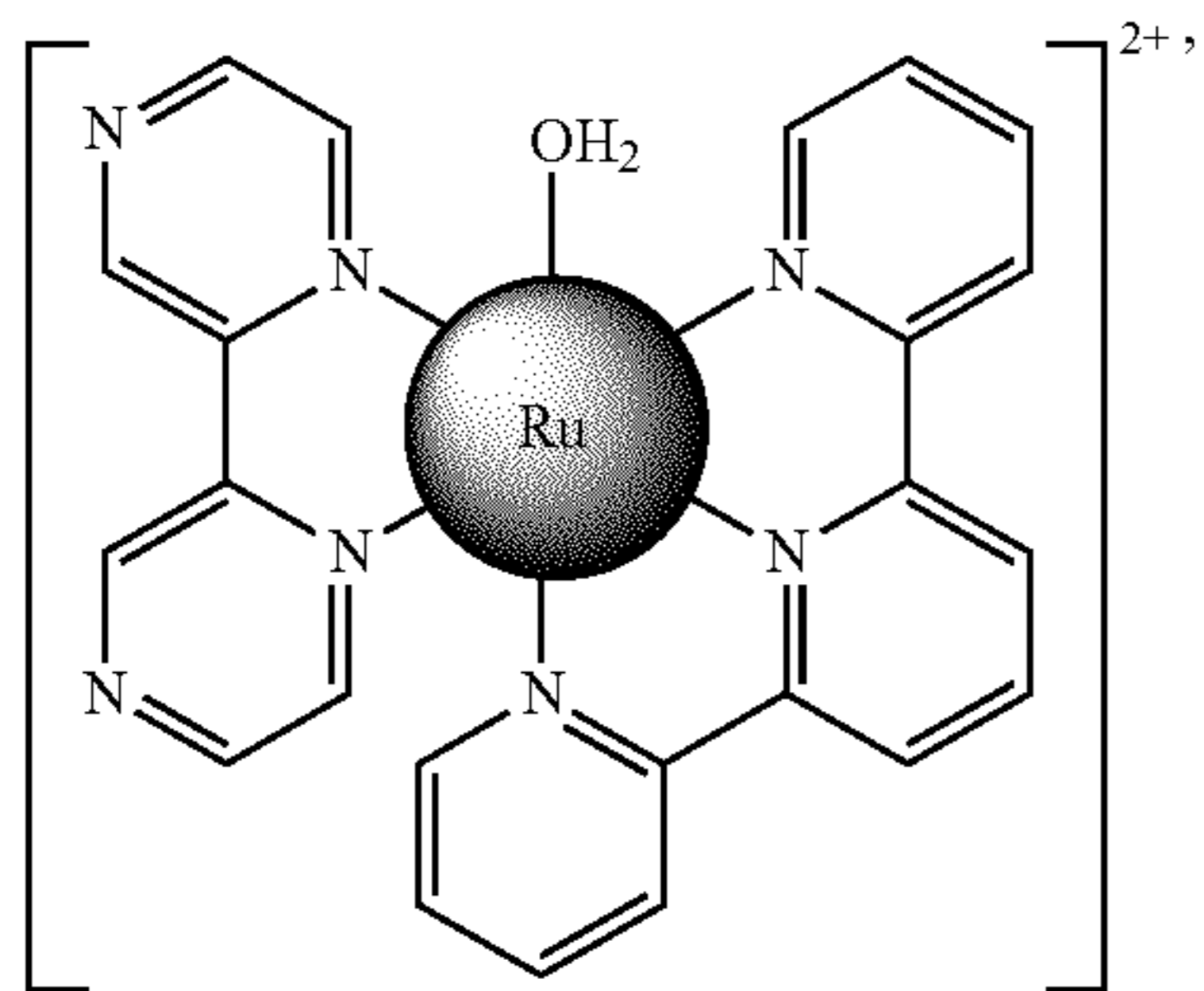
[Ru(tpy)(bpz)(OH_2)]^{2+} ,
