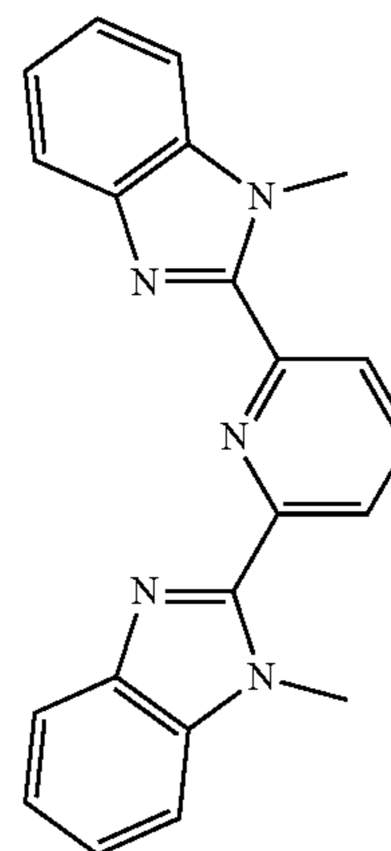
2,6-bis(1-methylbenzimidazol-2-yl)pyridine (Mebimpy).
