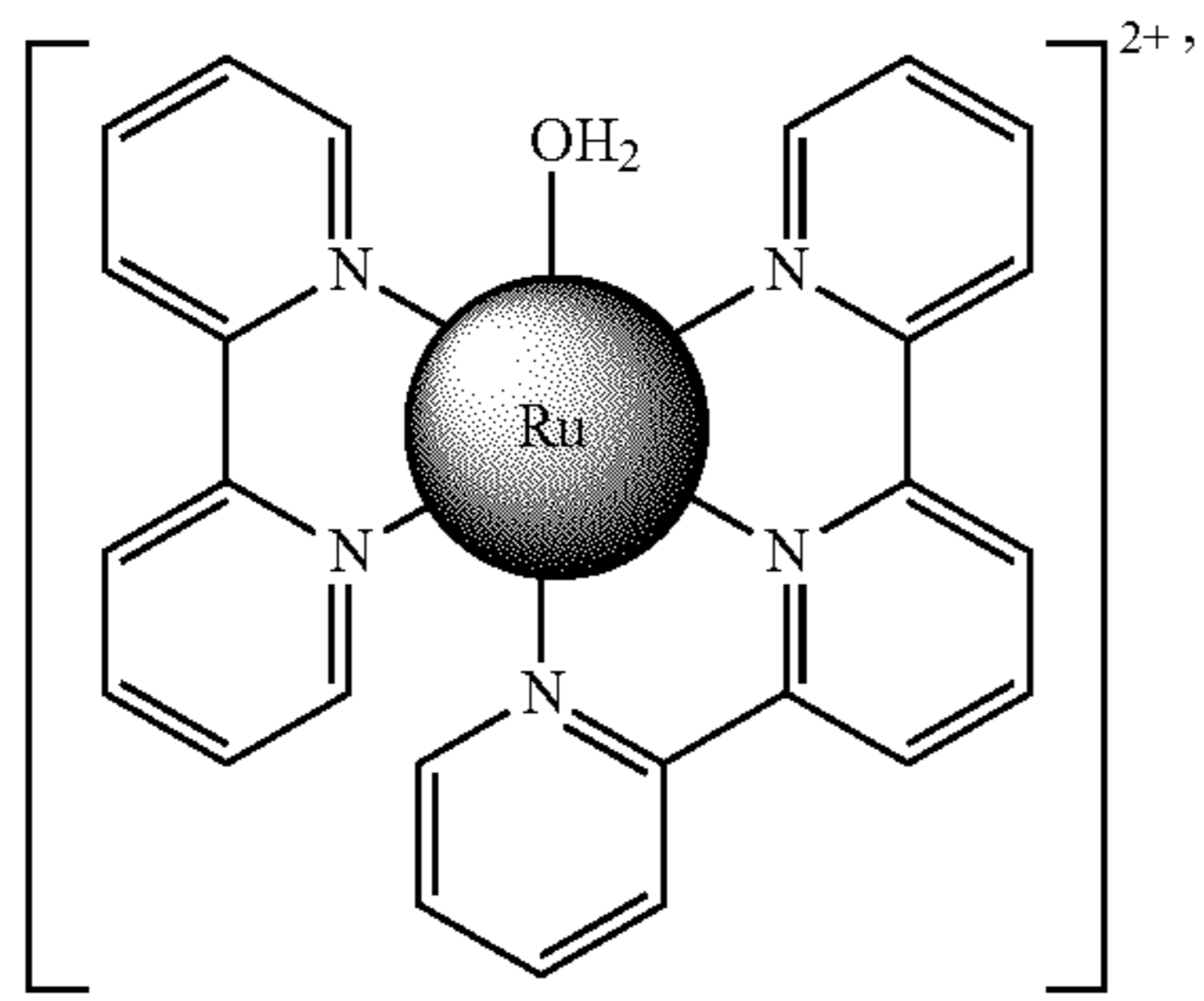
[Ru(tpy)(bpy)(OH_2)]^{2+} ,
