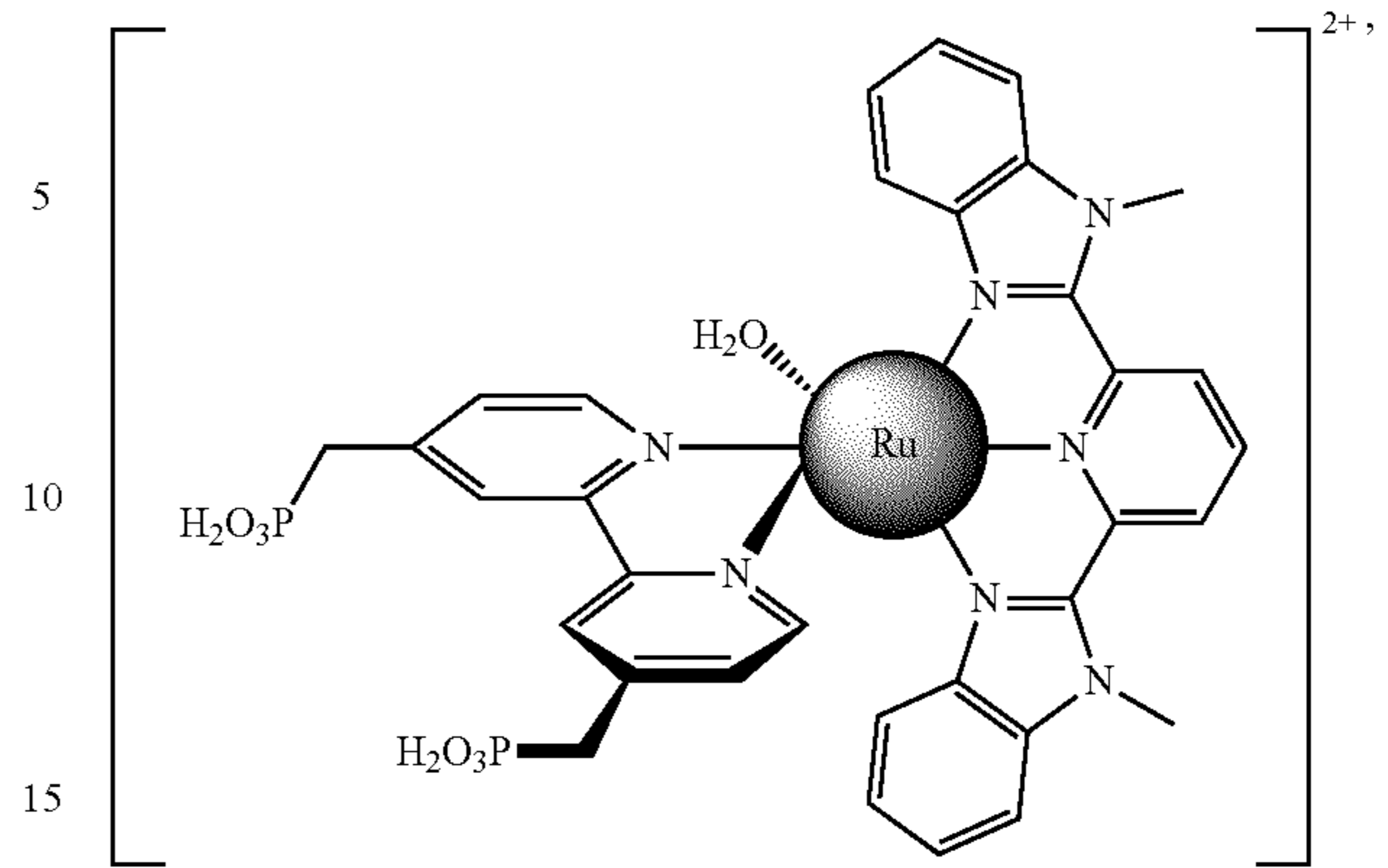
[Ru(Mebimpy)(P_2-bpy)]^{2+} ,
