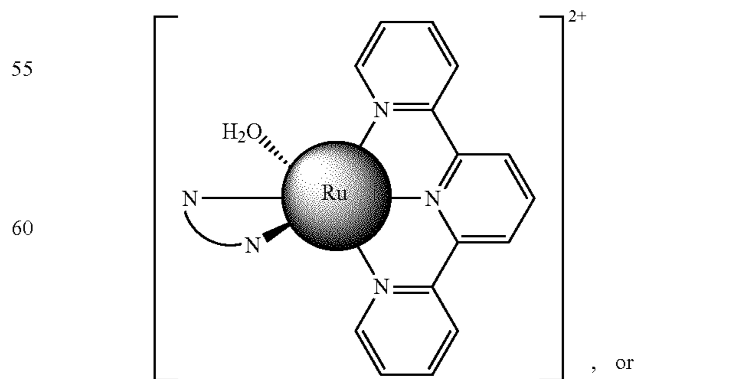
[Ru(Mebimpy)(bpy)(OH_2)]^{2+}
