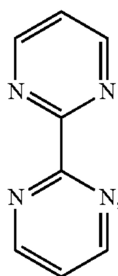
bpm
