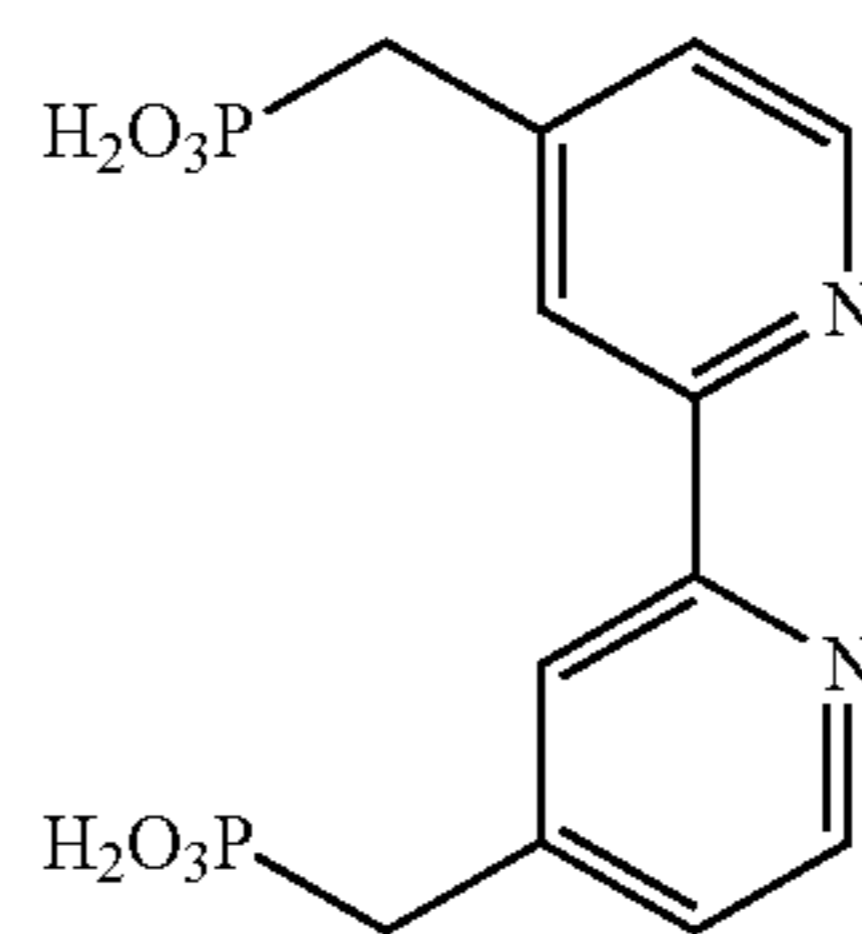
\text{P}_2 -bpy
