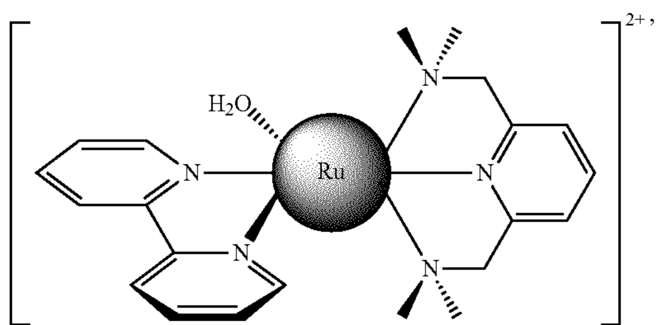
[Ru(DMAP)(bpy)(OH_2)]^{2+} ,
