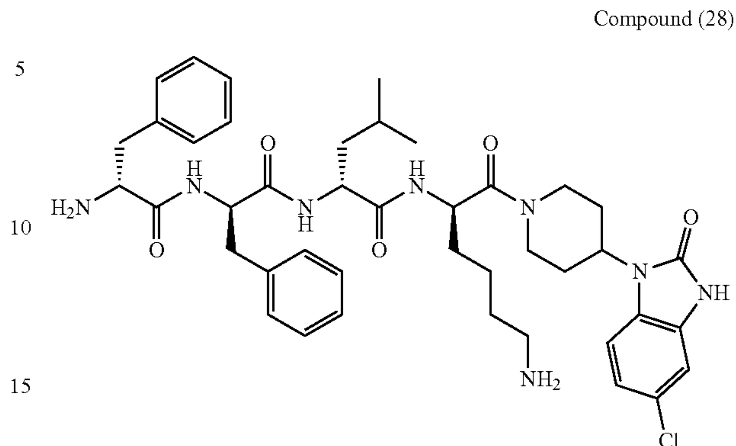
D-Phe-D-Phe-D-Leu-D-Lys-[5-chloro-1-(piperidin-4-yl)-1H-benzo[d]imidazol-2(3H)-one amide]
