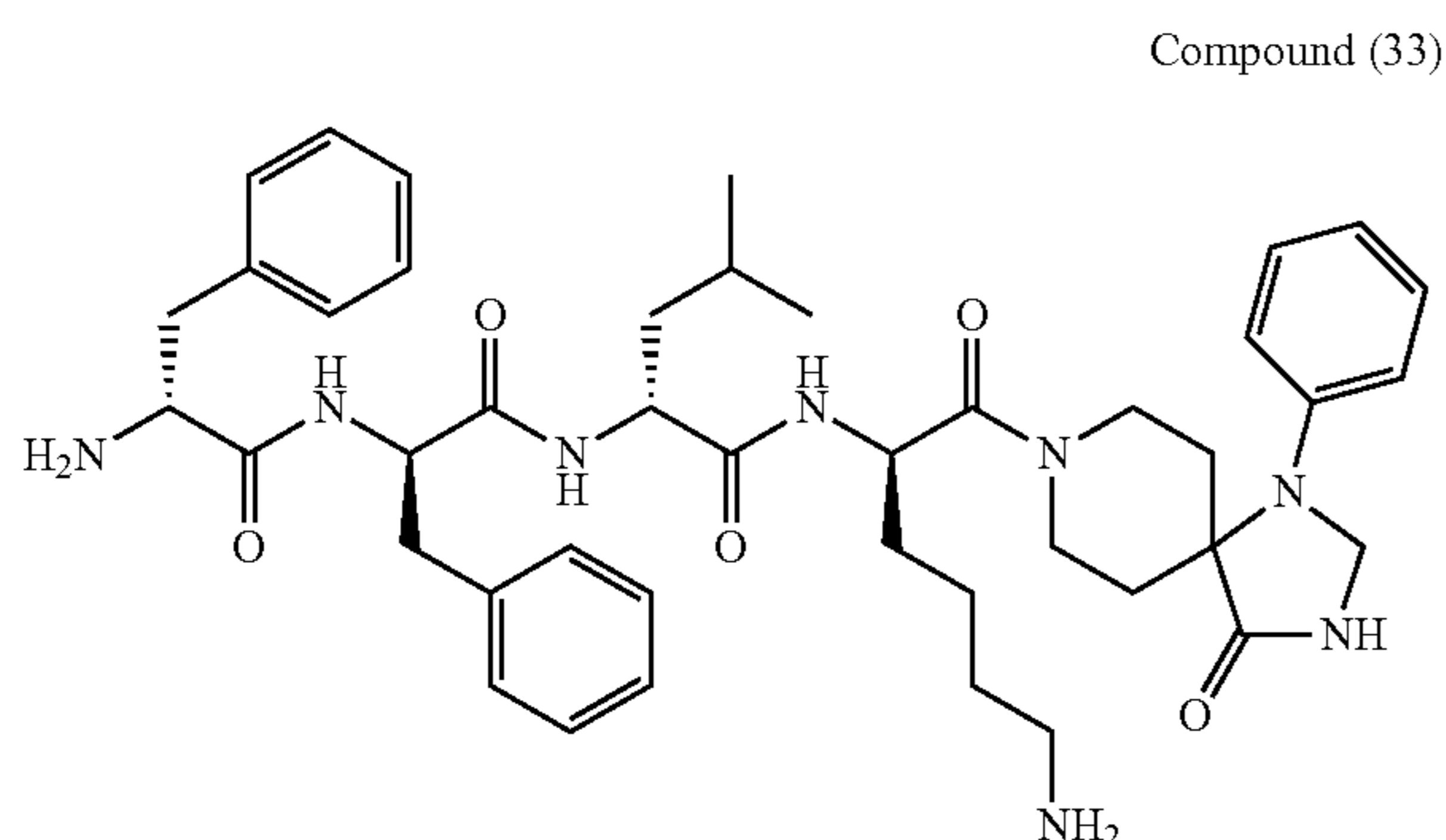
D-Phe-D-Phe-D-Leu-D-Lys-[1-phenyl-1,3,8-triazaspiro[4.5]decan-4-one amide]
