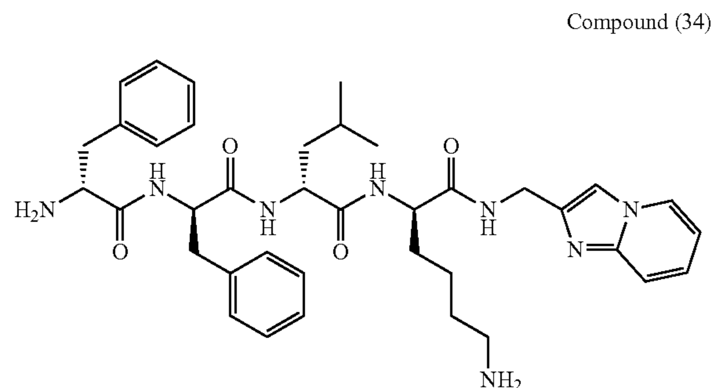
D-Phe-D-Phe-D-Leu-D-Lys-[imidazo[1,2-a]pyridine-2-ylmethyl amide]
