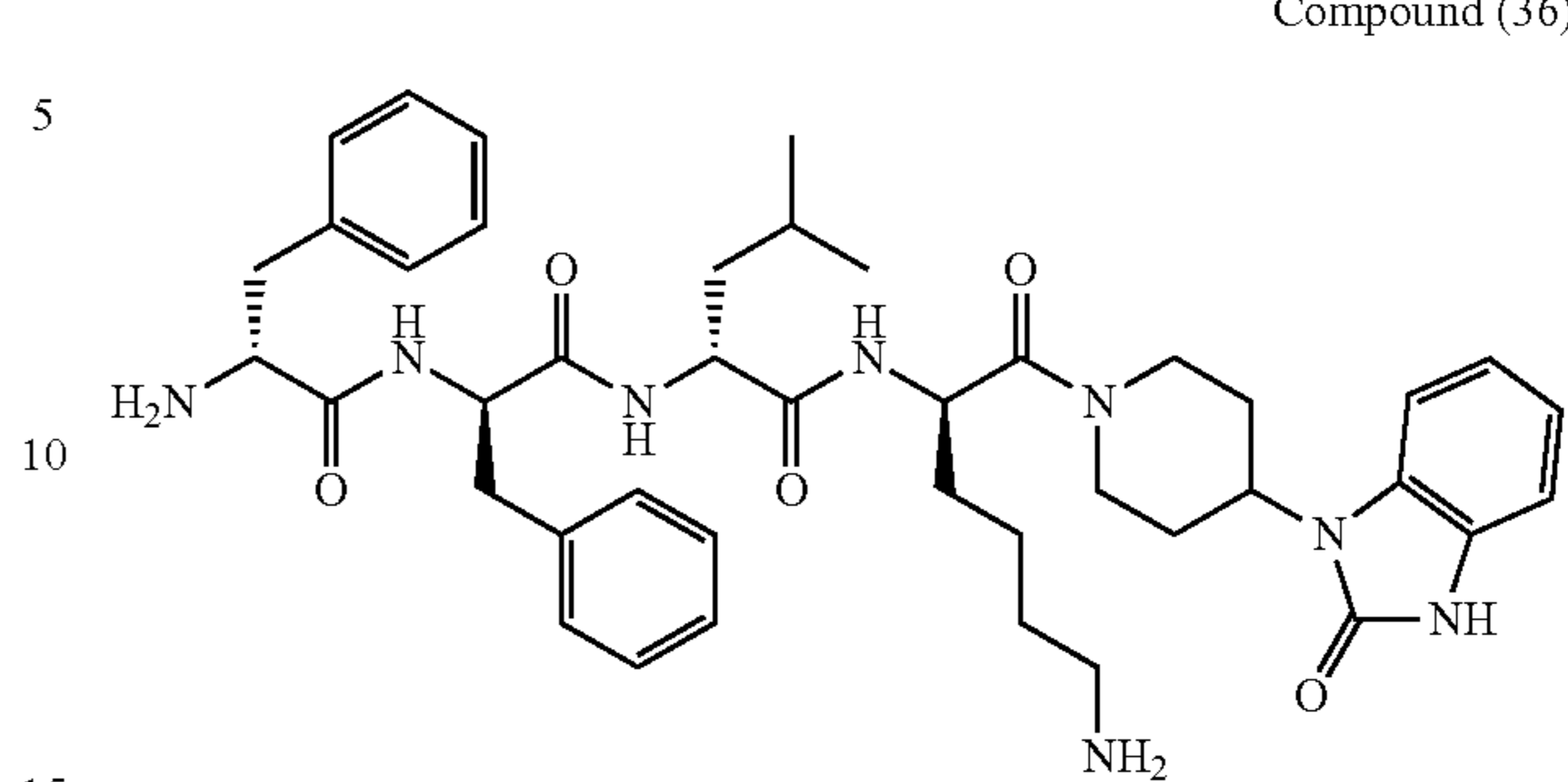
D-Phe-D-Phe-D-Leu-D-Lys-[1-(piperidin-4-yl)-1H-benzo[d]imidazol-2(3H)-one amide]
