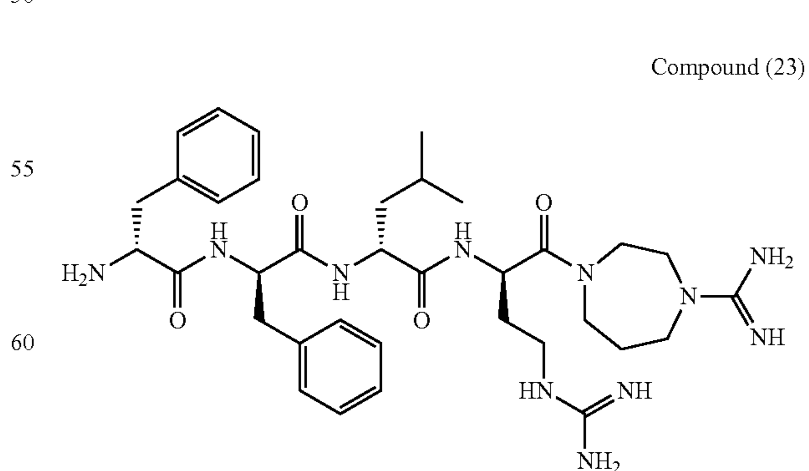
D-Phe-D-Phe-D-Leu-D-Nar-[4-Amidinohomopiperazine amide]
