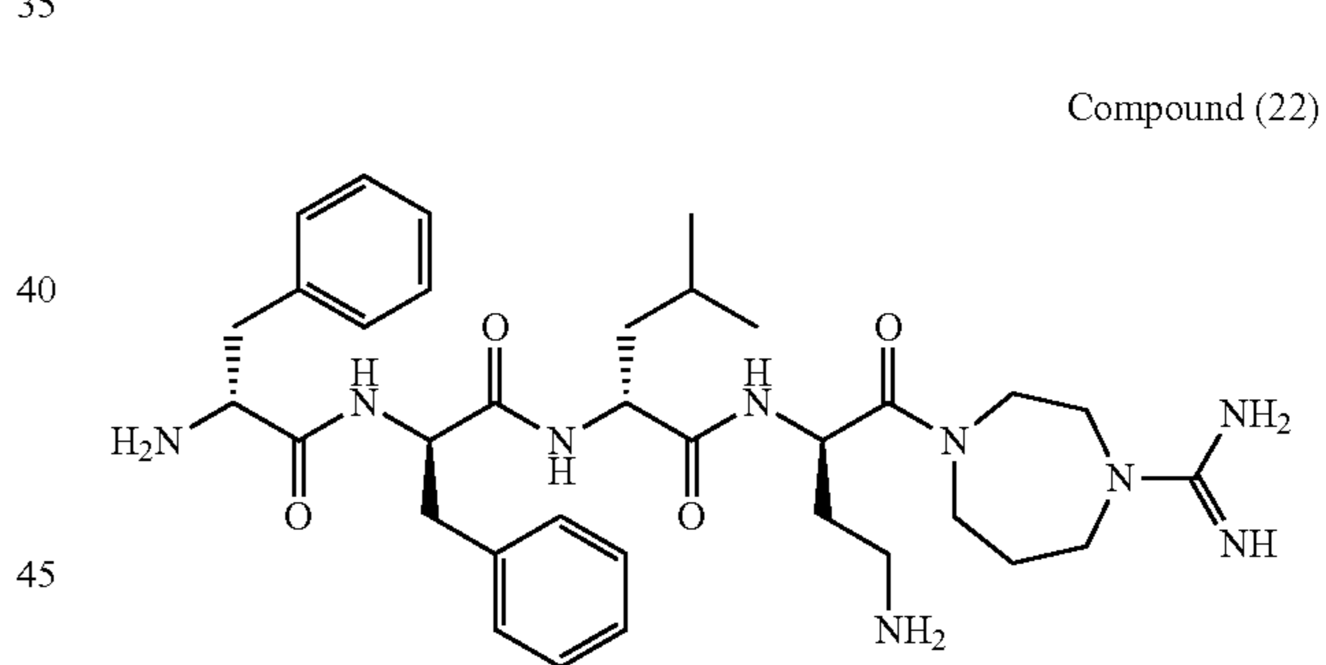
D-Phe-D-Phe-D-Leu-D-Dbu-[4-Amidinohomopiperazine amide]
