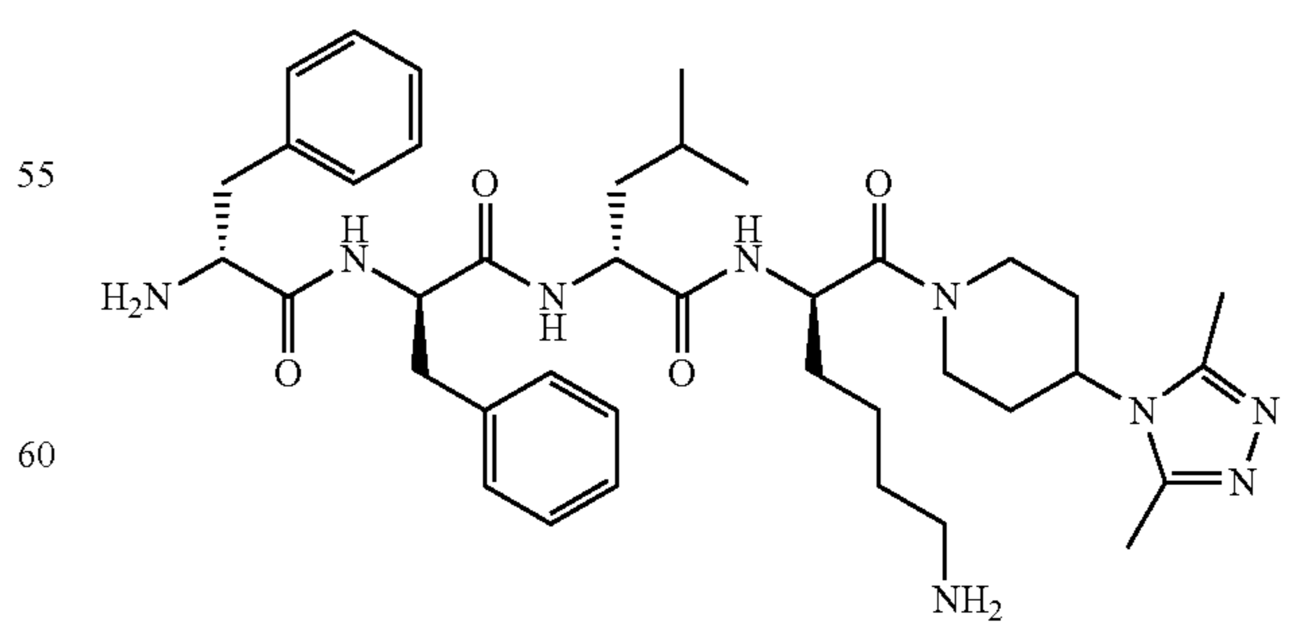
D-Phe-D-Phe-D-Leu-D-Lys-[4-(3,5-dimethyl-4H-1,2,4-triazol-4-yl)piperidine amide]
