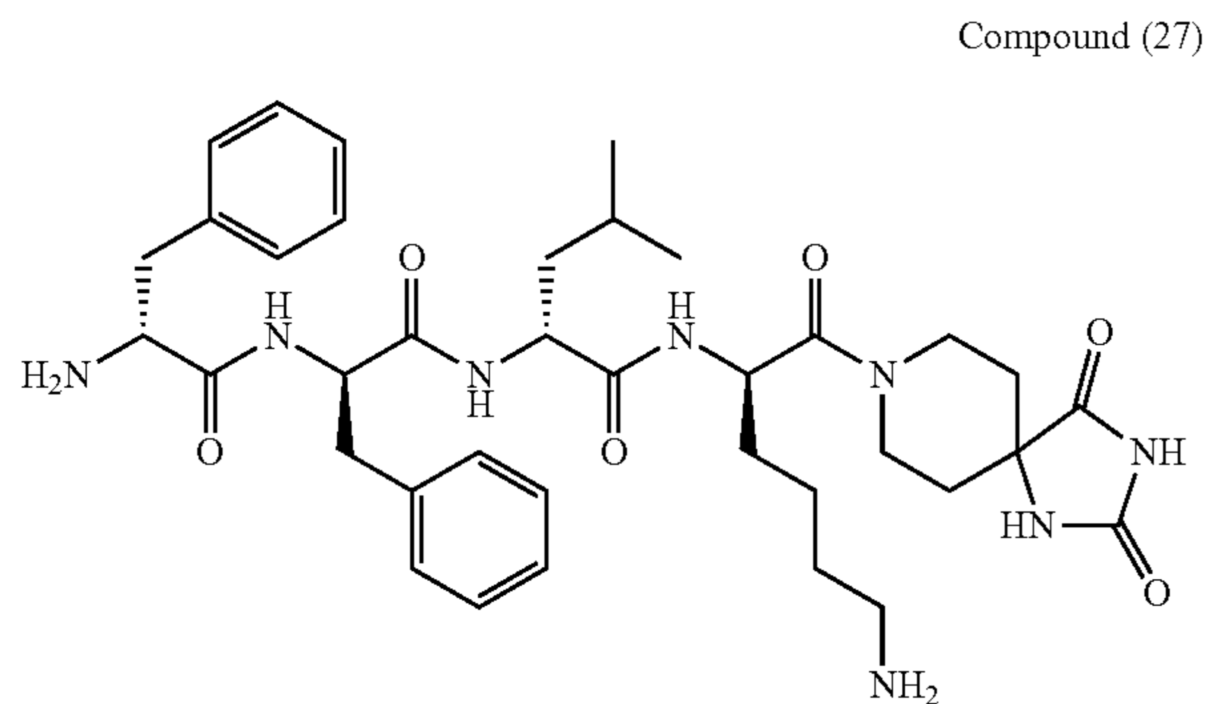
D-Phe-D-Phe-D-Leu-D-Lys-[1,3,8-triazaspiro[4,5]decane-2,4-dione amide]
