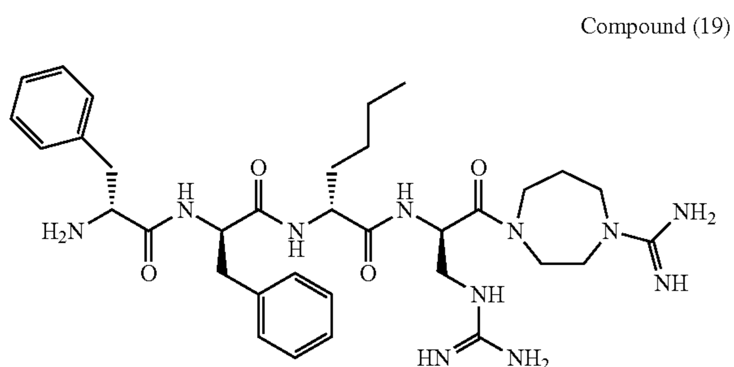
D-Phe-D-Phe-D-Nle-(β-amidino)D-Dap-[4-Amidinohomopiperazine amide]
