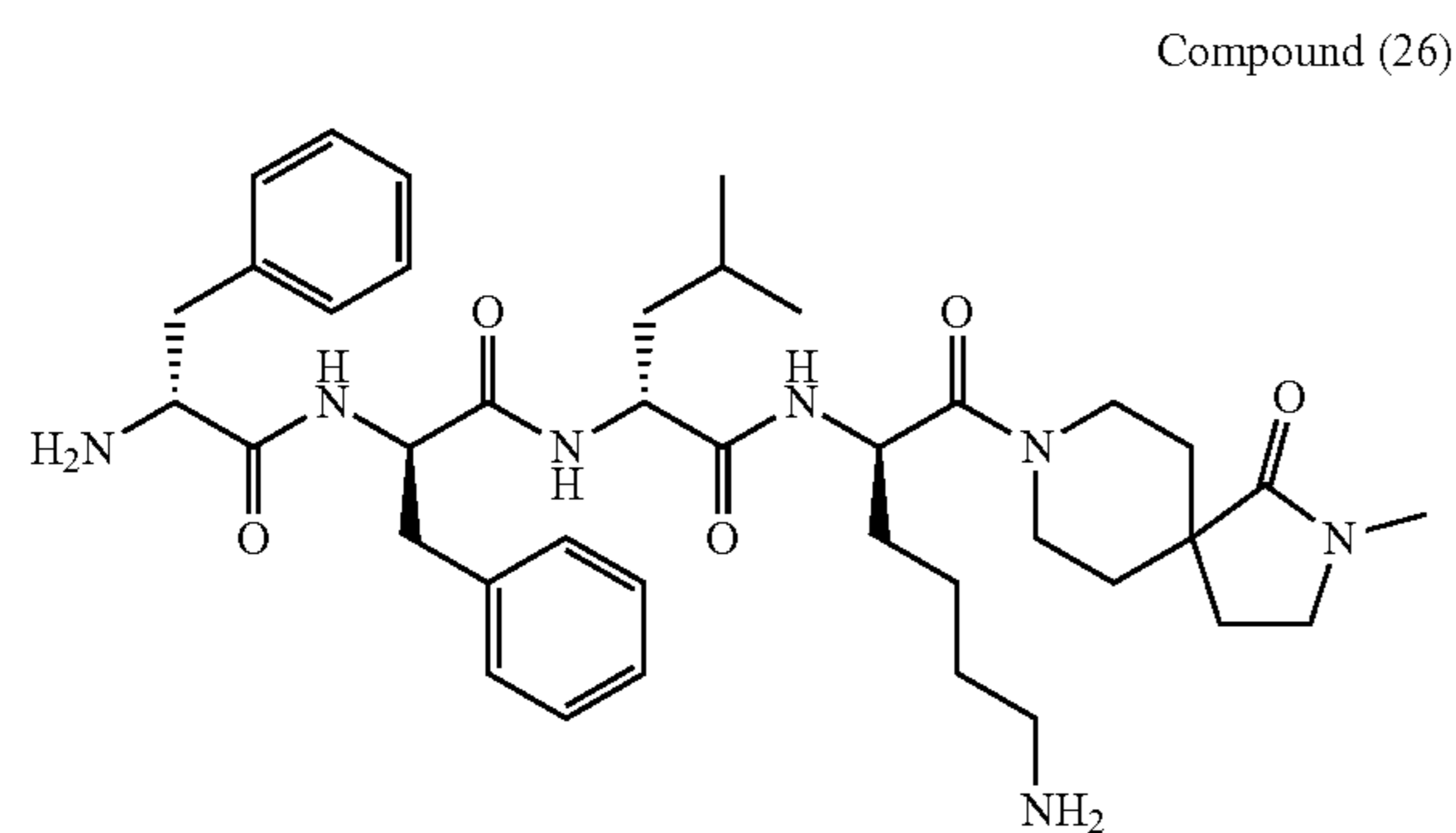
D-Phe-D-Phe-D-Leu-D-Lys-[2-methyl-2,8-diazaspiro[4,5]decan-1-one amide]
