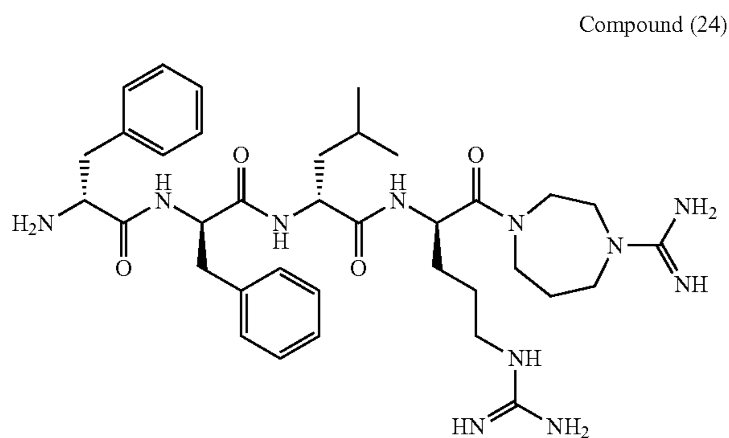
D-Phe-D-Phe-D-Leu-D-Arg-[4-Amidinohomopiperazine amide]
