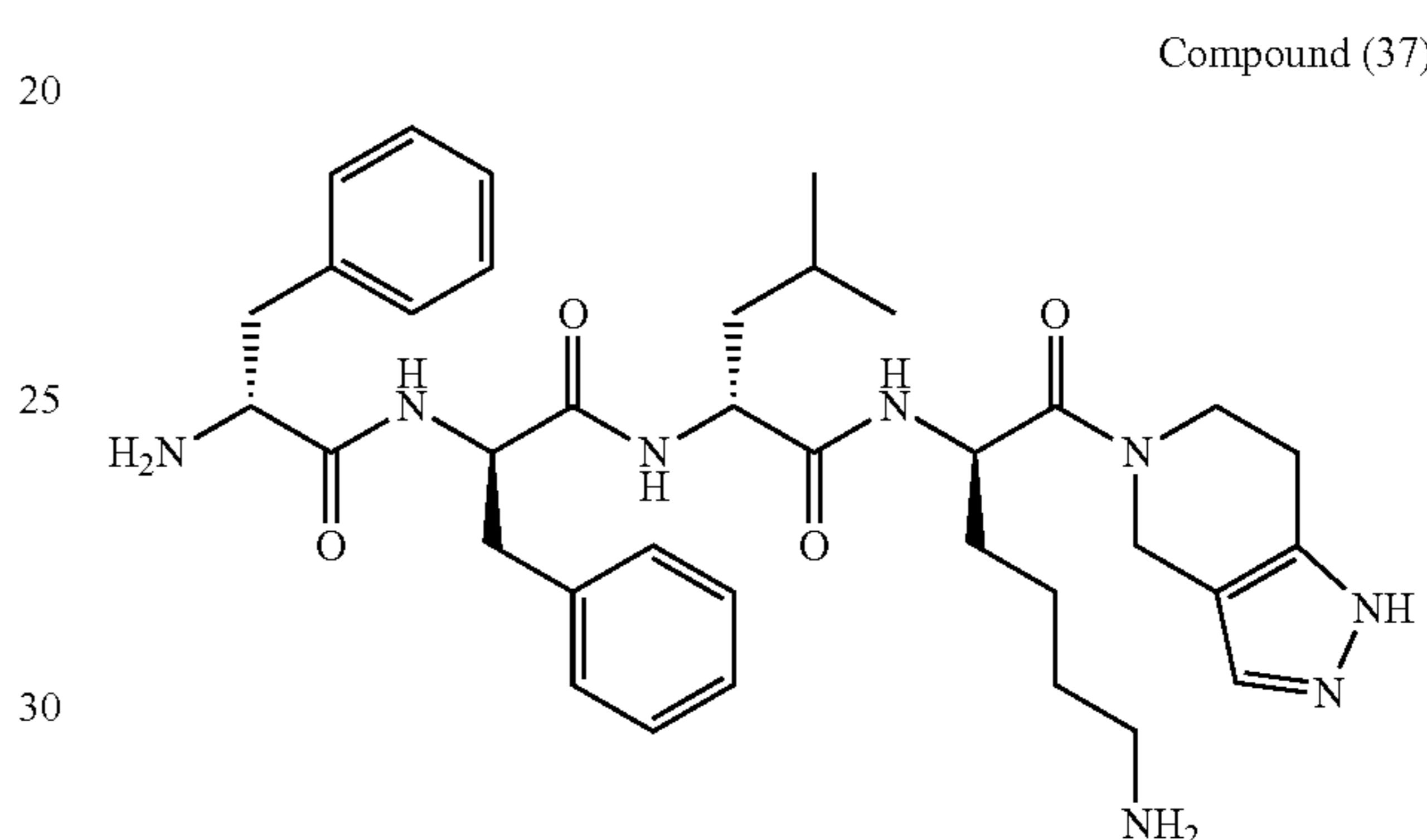
D-Phe-D-Phe-D-Leu-D-Lys-[4,5,6,7-tetrahydro-1H-pyrazolo[4,3-c]pyridine amide]
