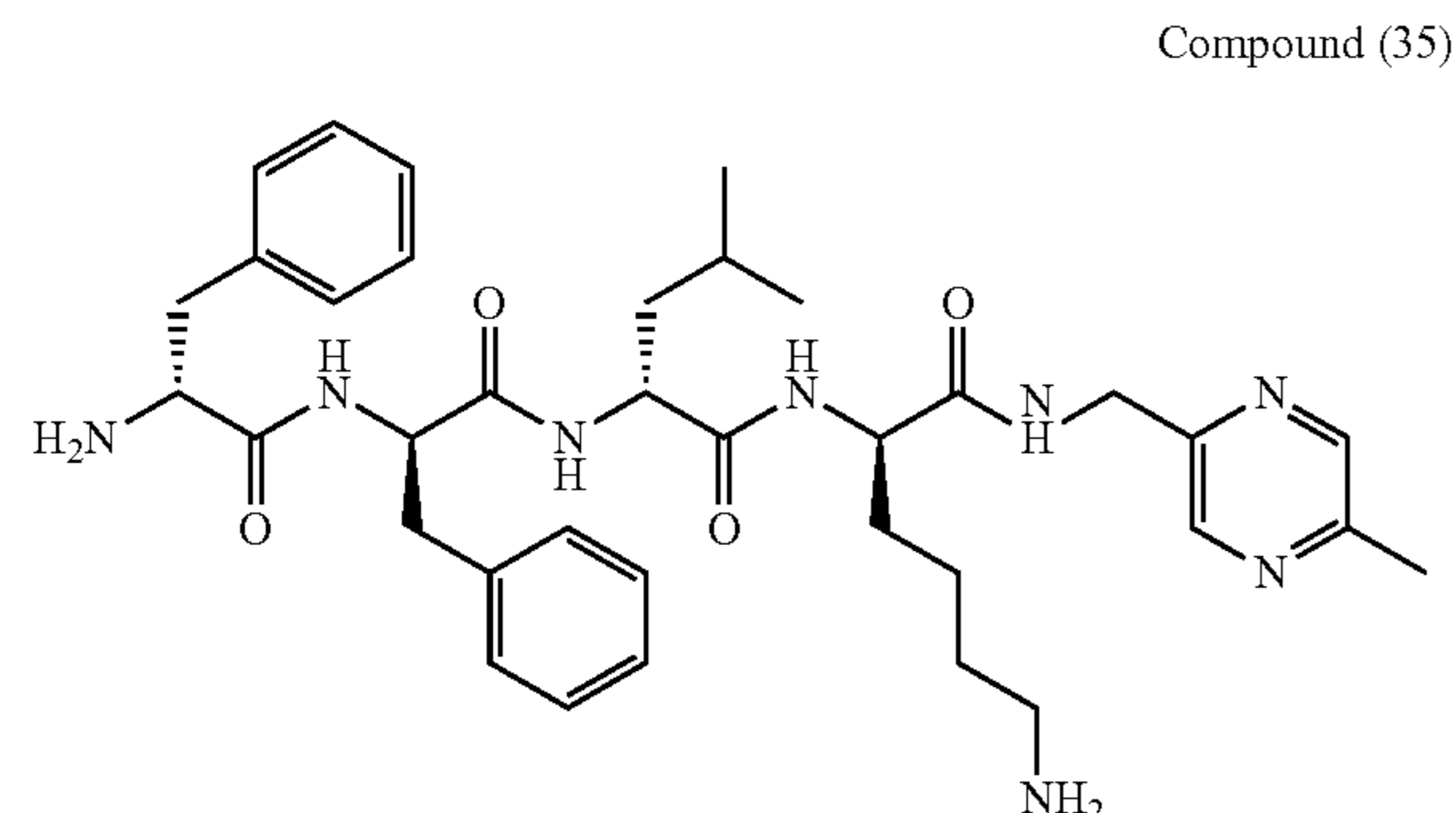
D-Phe-D-Phe-D-Leu-D-Lys-[(5-methylpyrazin-2-yl)methyl amide]
