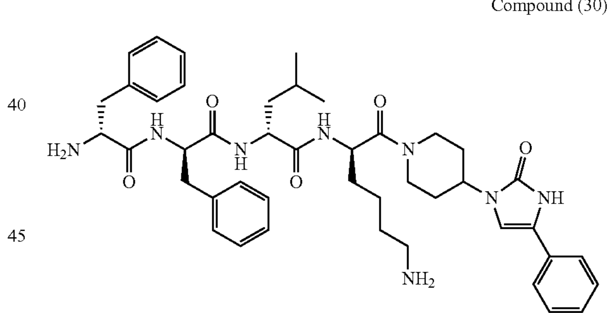
D-Phe-D-Phe-D-Leu-D-Lys-[4-phenyl-1-(piperidin-yl)-1H-imidazol-2(3H)-one amide]
