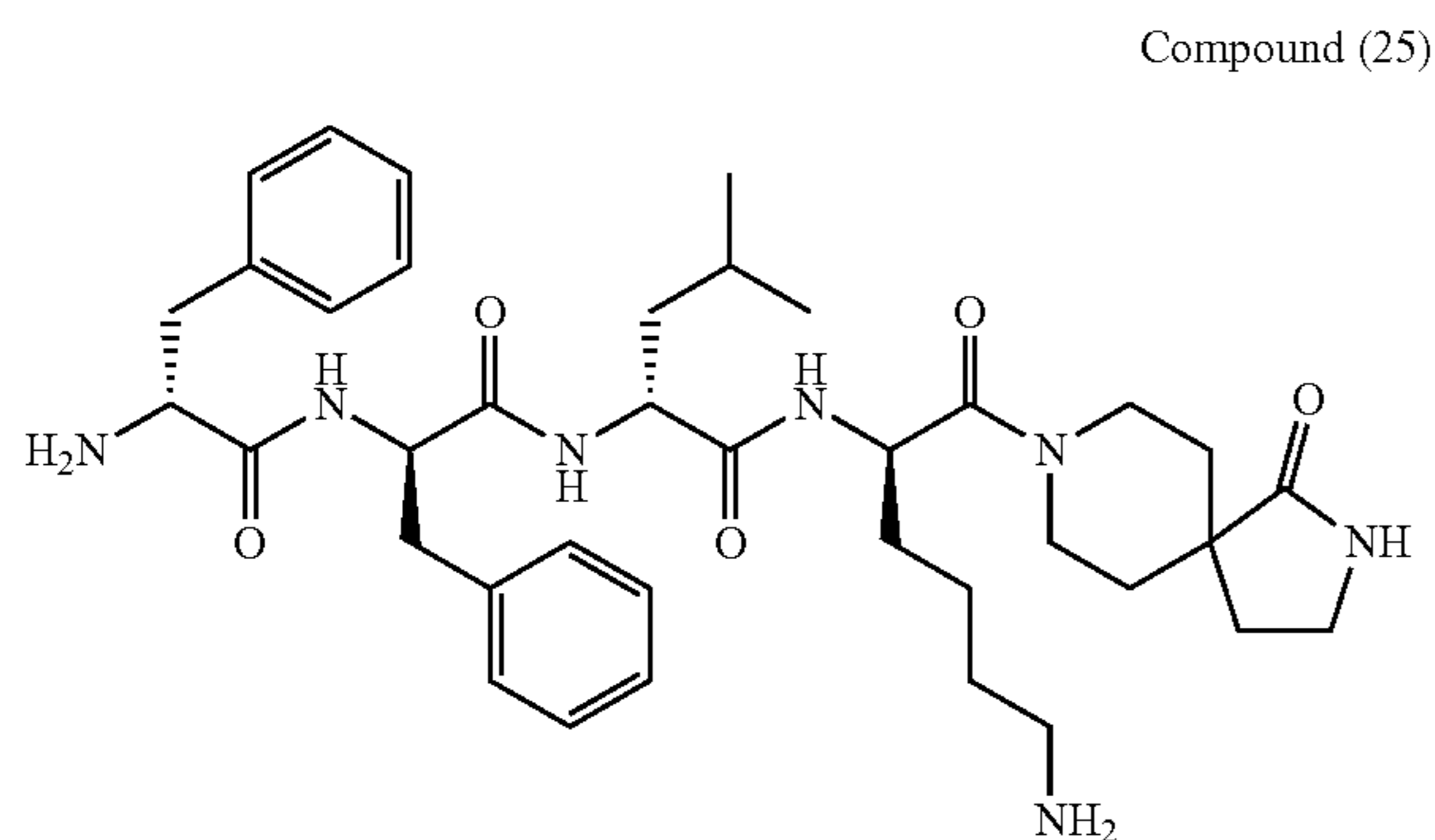
D-Phe-D-Phe-D-Leu-D-Lys-[2,8-diazaspiro[4,5]decan-1-one amide]
