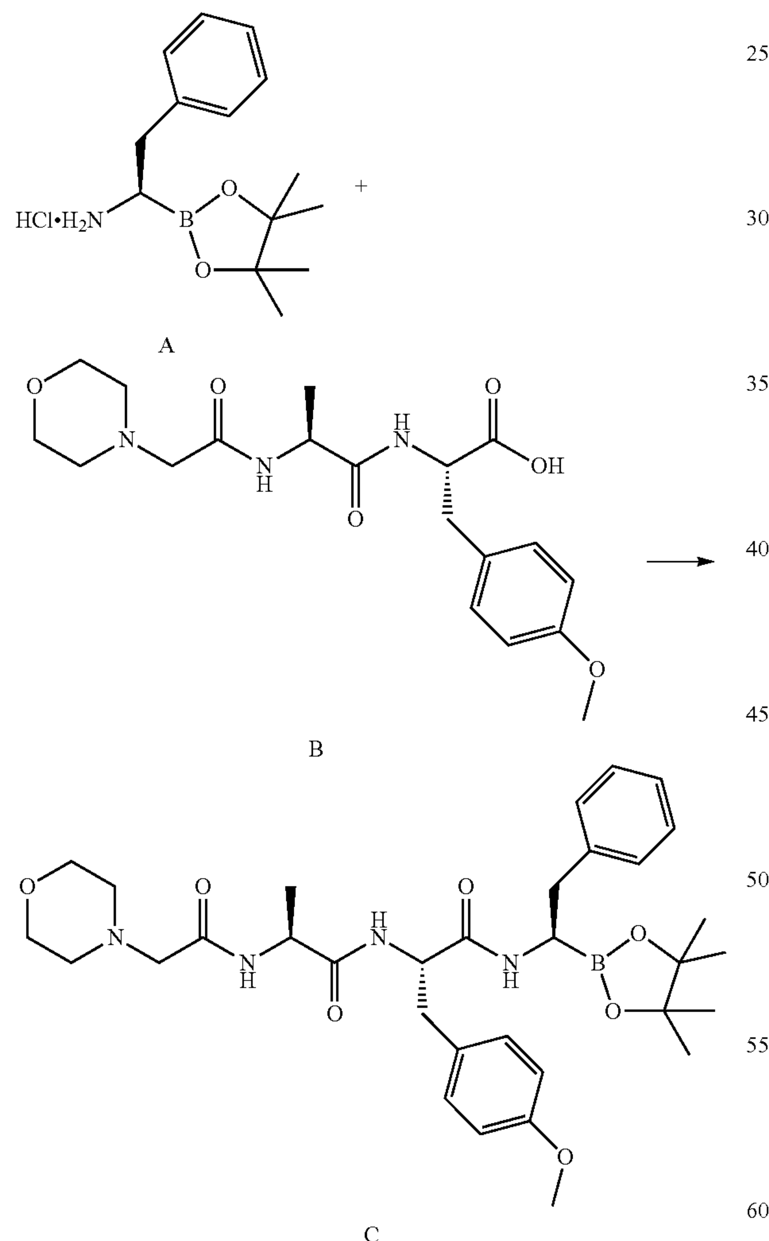
Scheme 1: Synthesis of Compound 1
