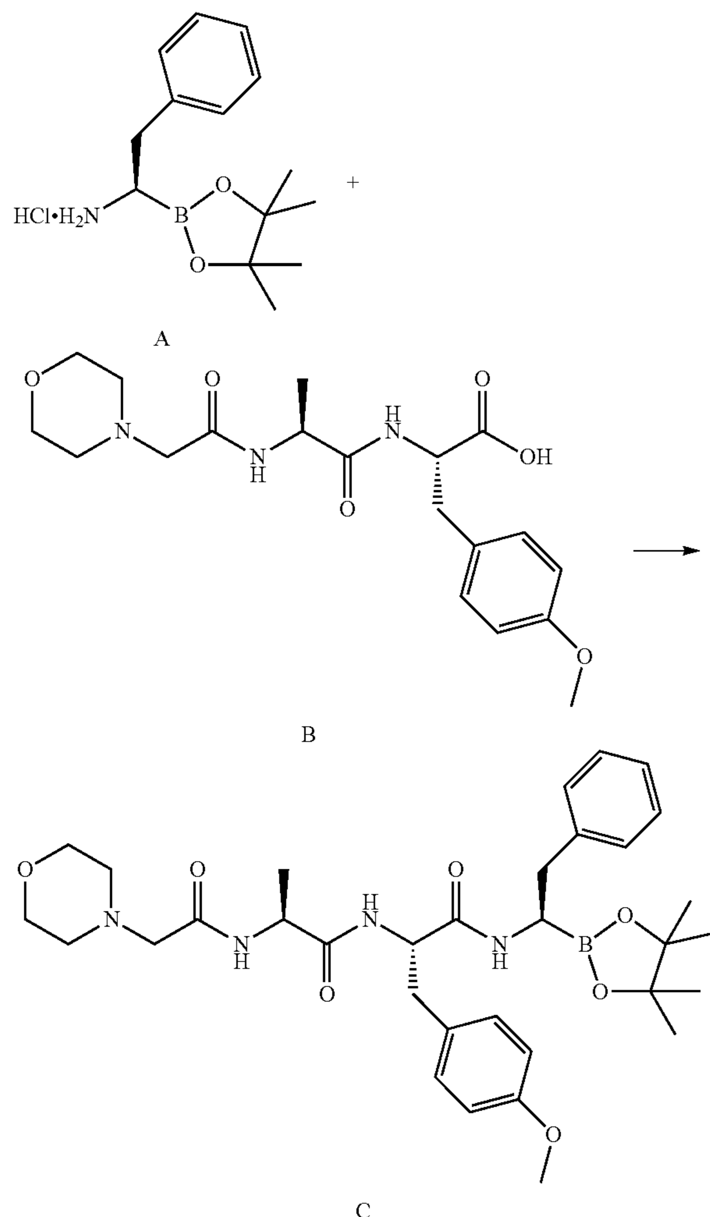
Scheme 1: Synthesis of Compound 1
