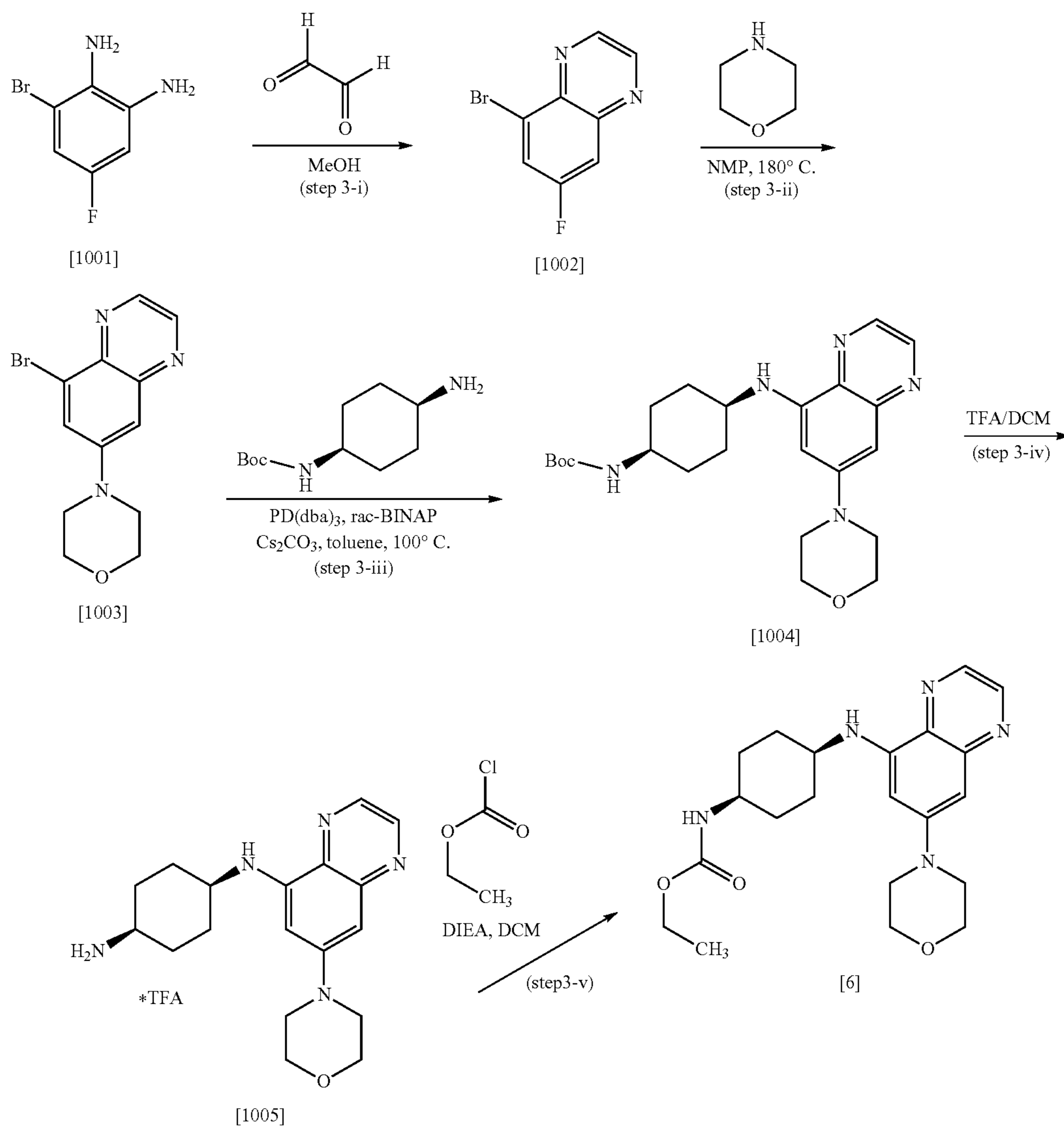
Scheme 3
