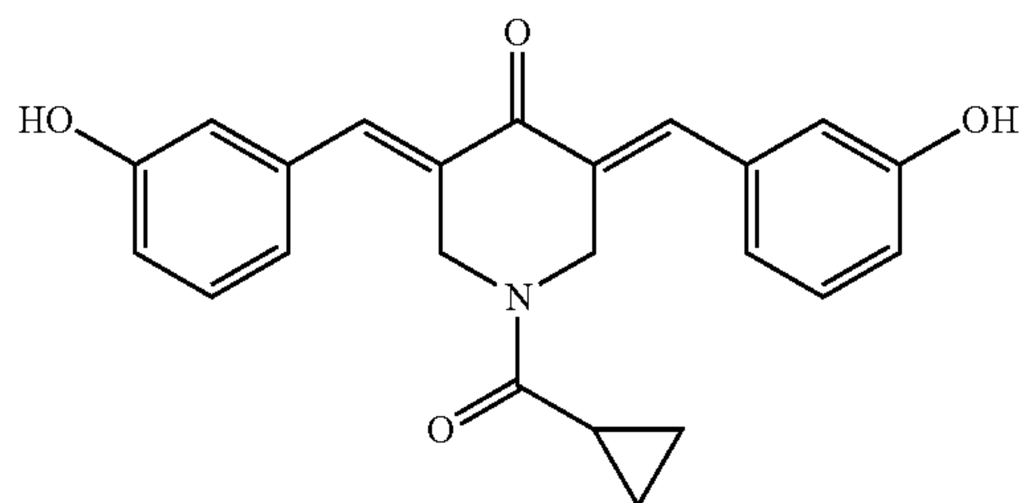
Compound 16
