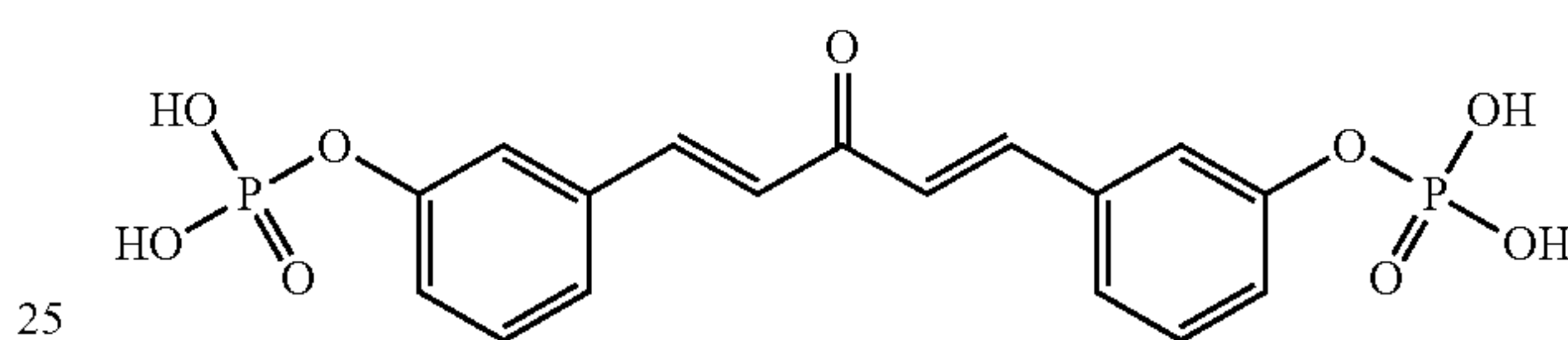
Compound 34
