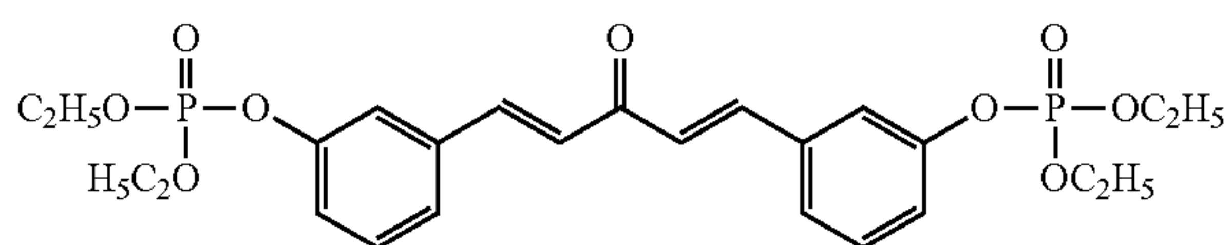
Compound 18
