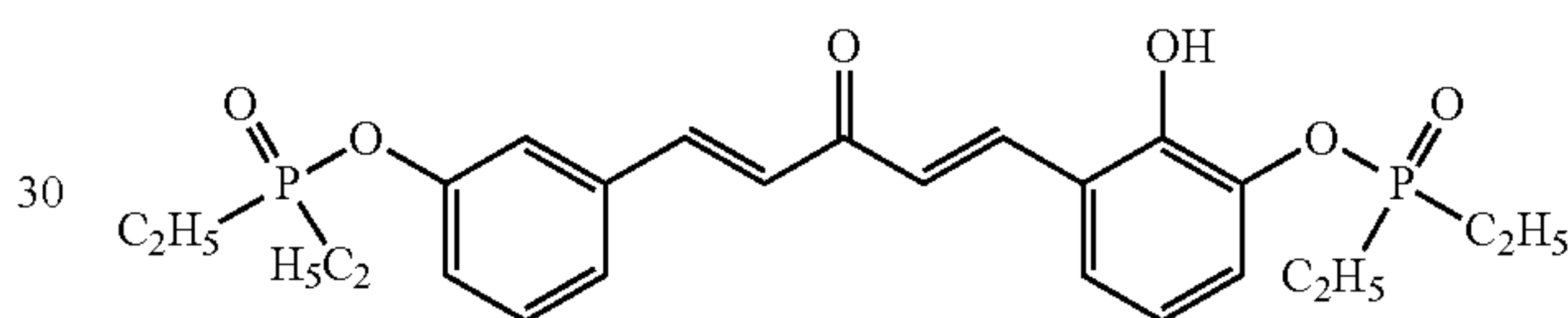
Compound 37
