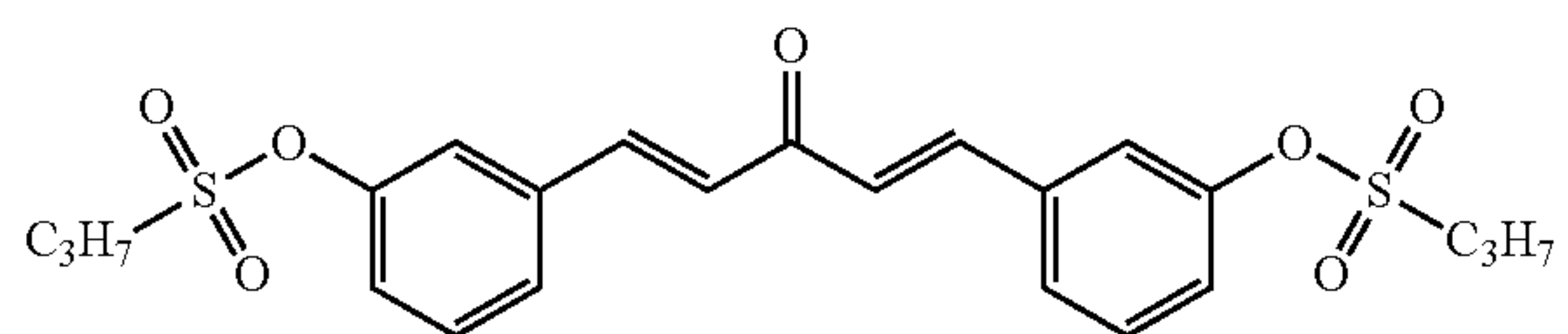
Compound 11
