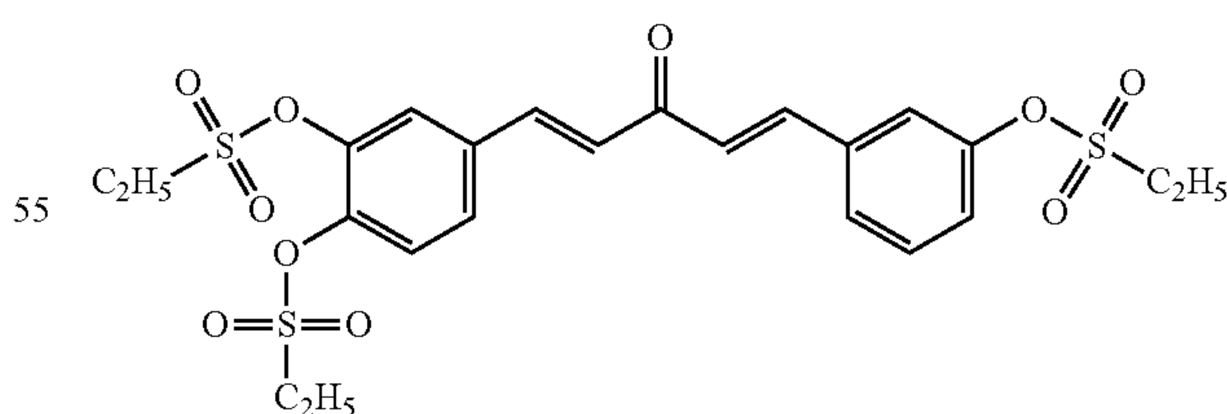
Compound 48
