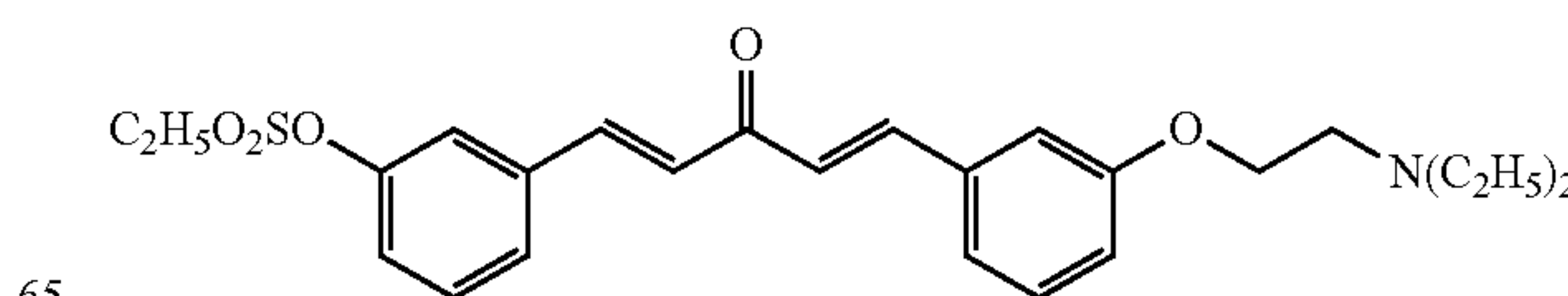
Compound 48
