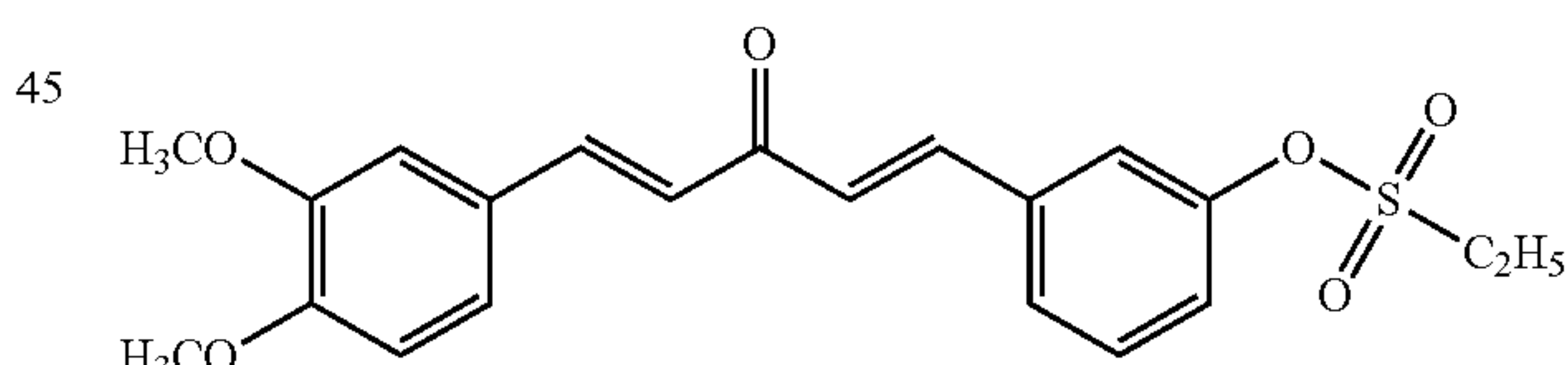
Compound 43
