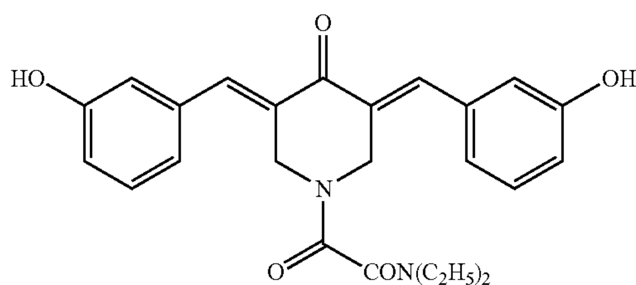
Compound 13
