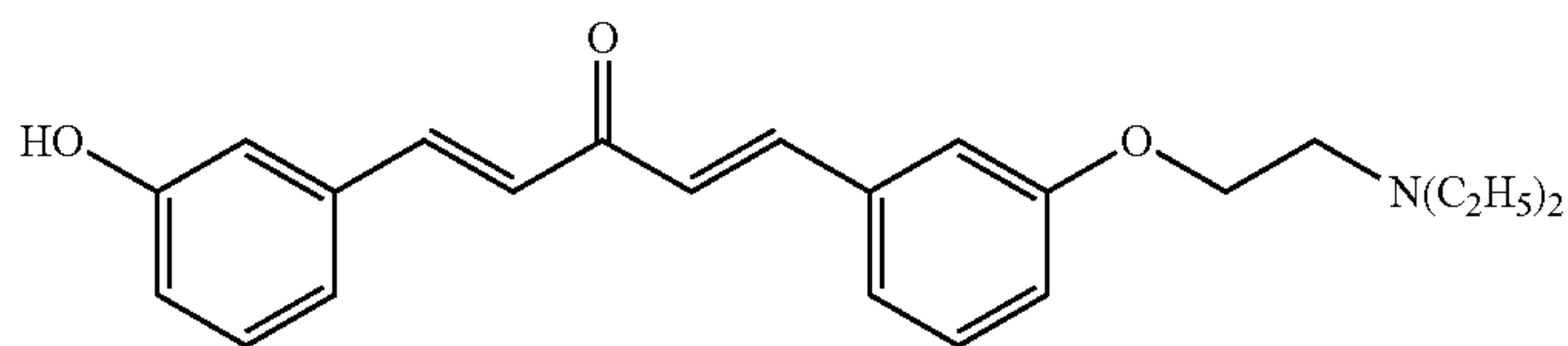
Compound 19
