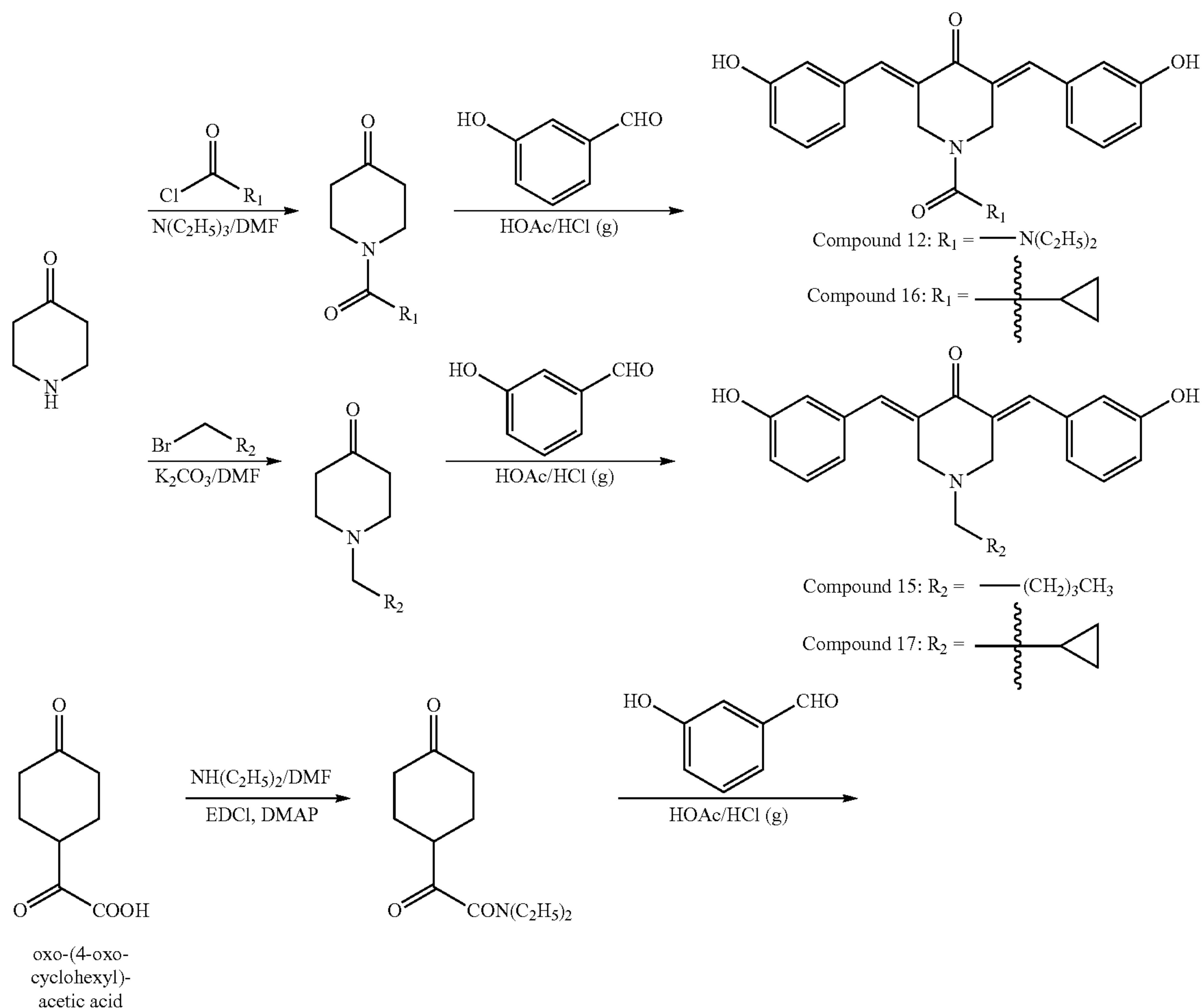
Scheme 6
