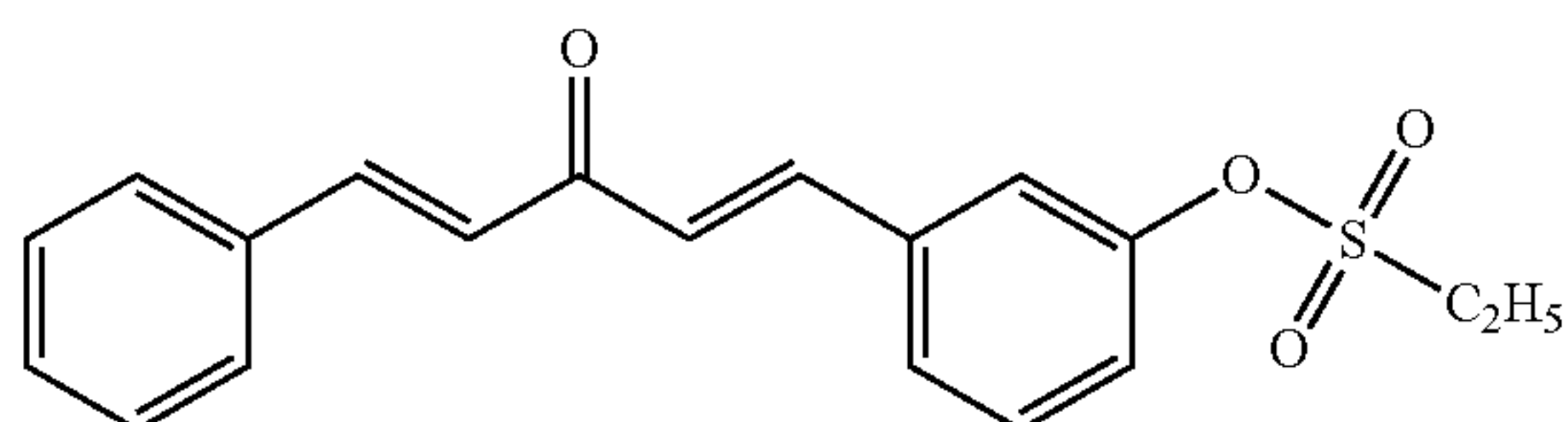
Compound 9
