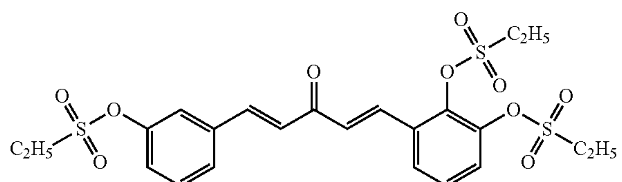
Compound 26
