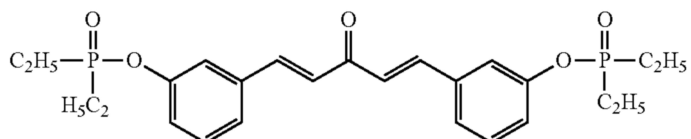
Compound 26
