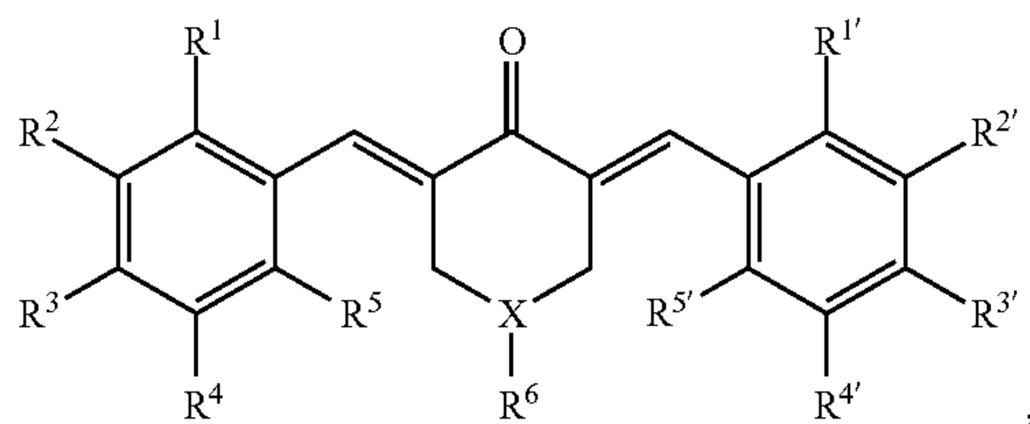
Formula (III)
