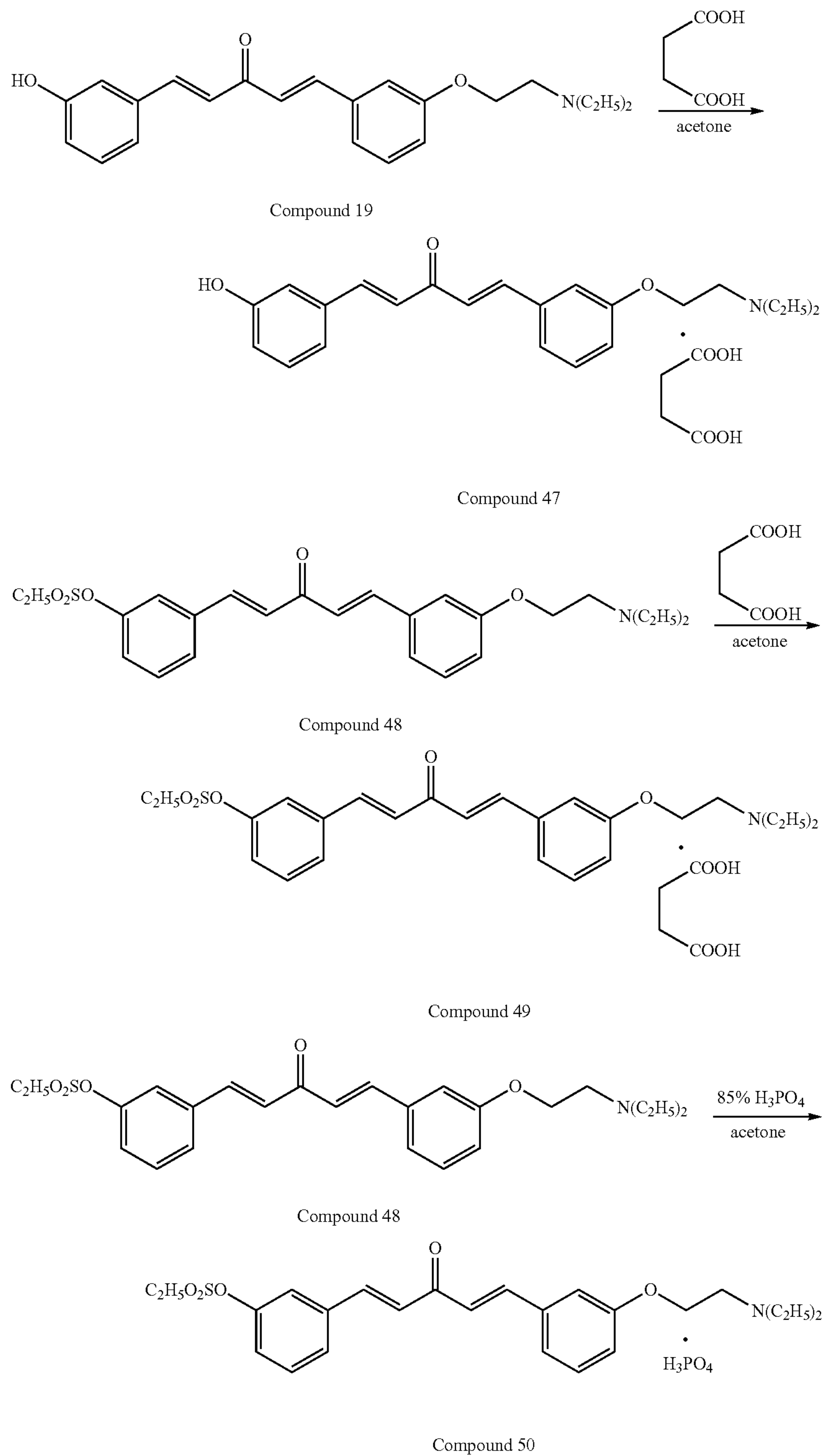
Scheme 9
