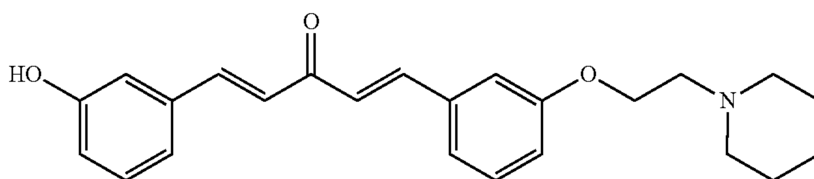
Compound 59
