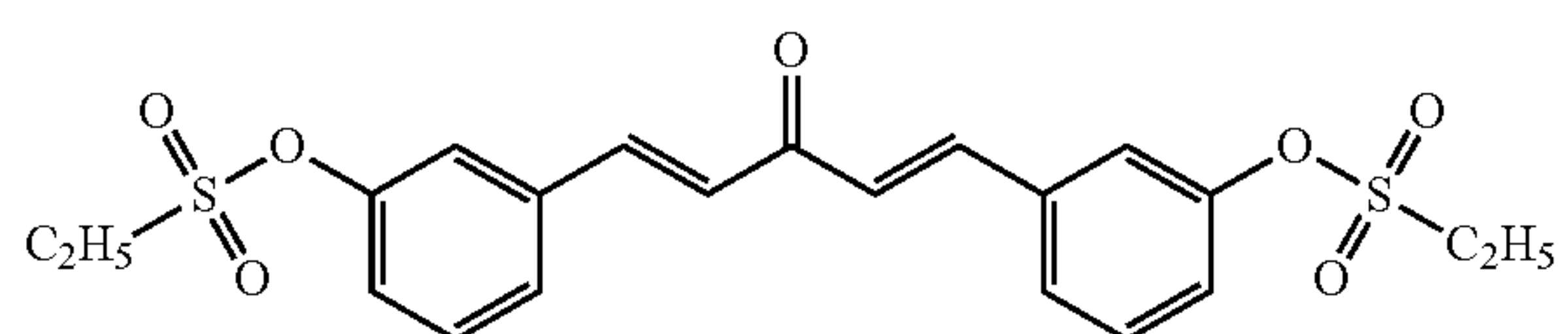
Compound 7
