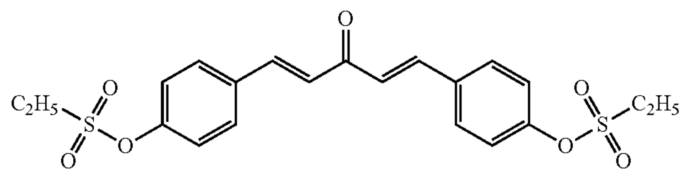
Compound 6
