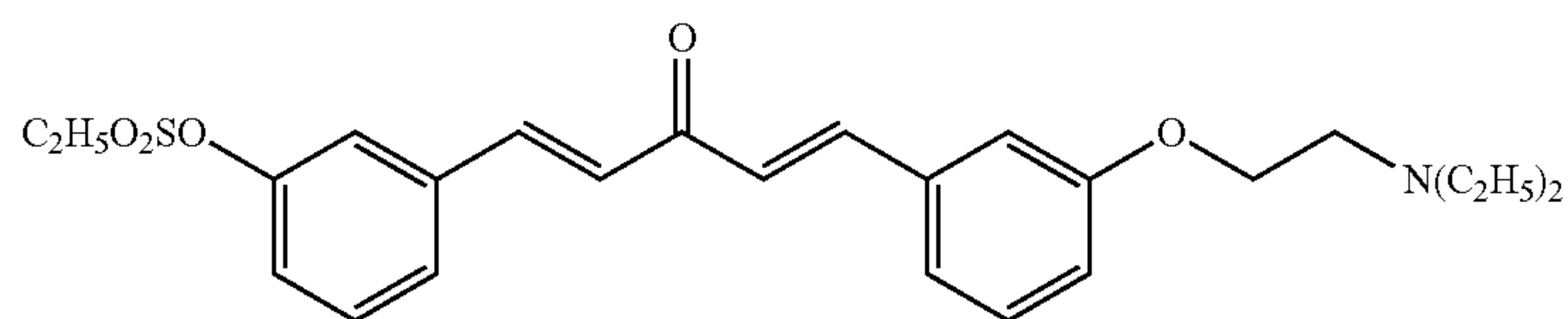
Compound 48
