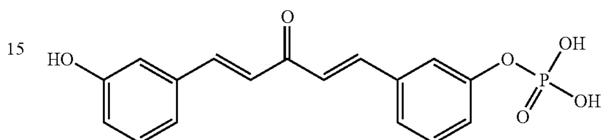
Compound 29
