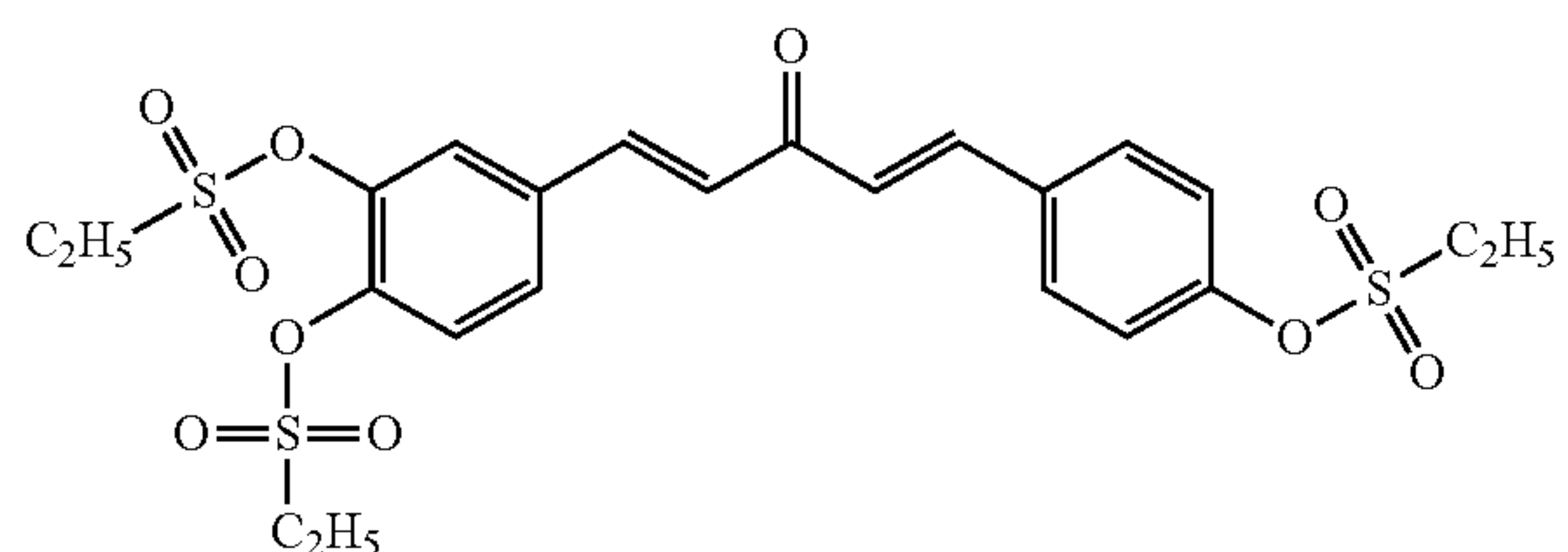
Compound 14
