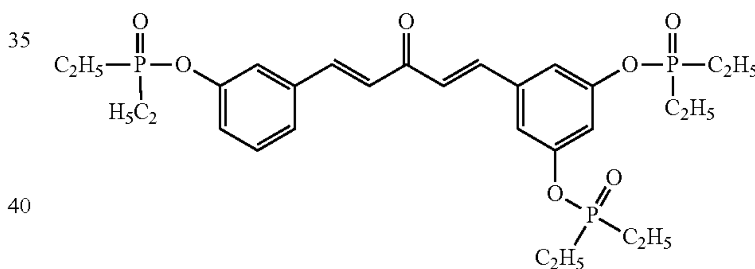
Compound 40
