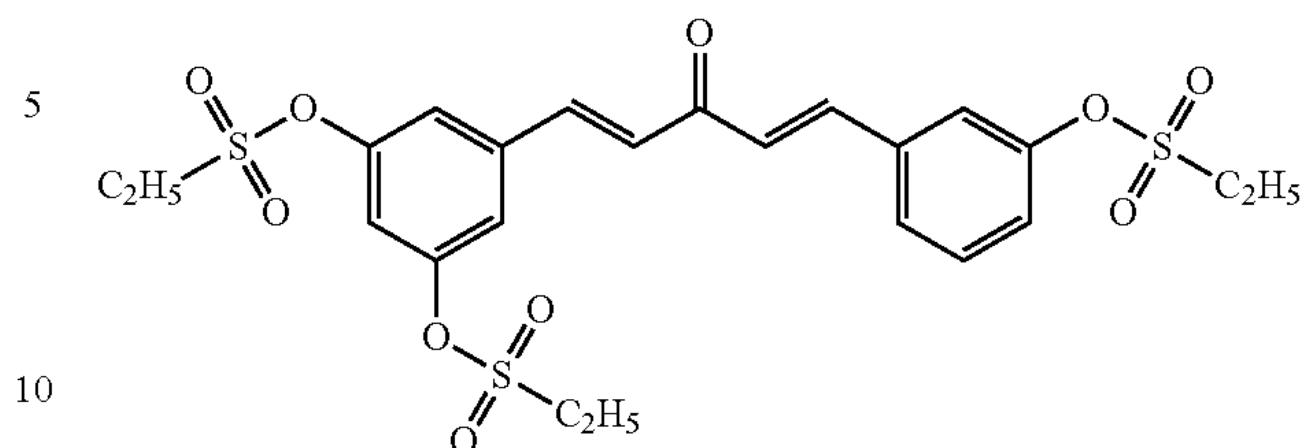
Compound 28
