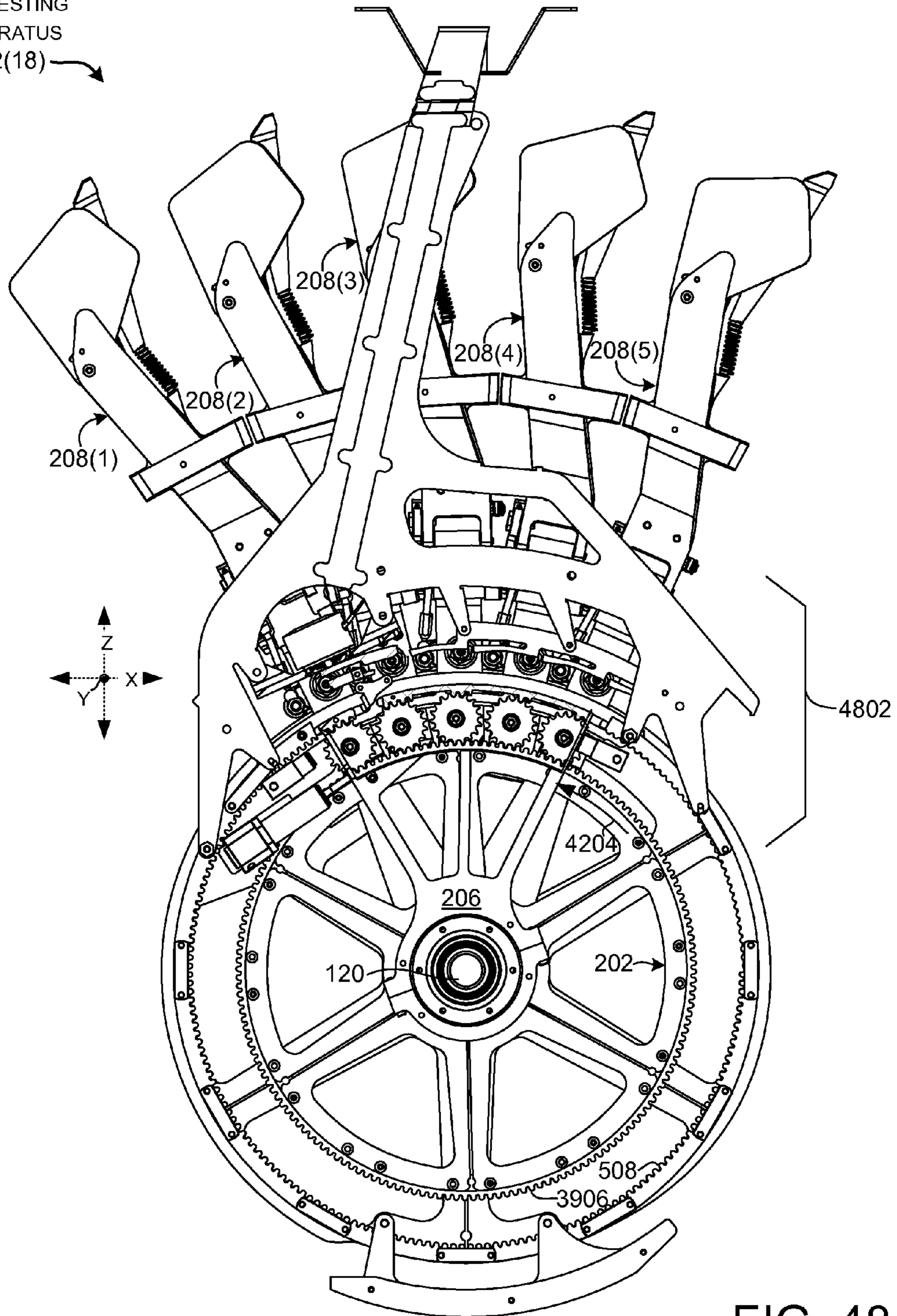
Mechanism 2009 Position 4
