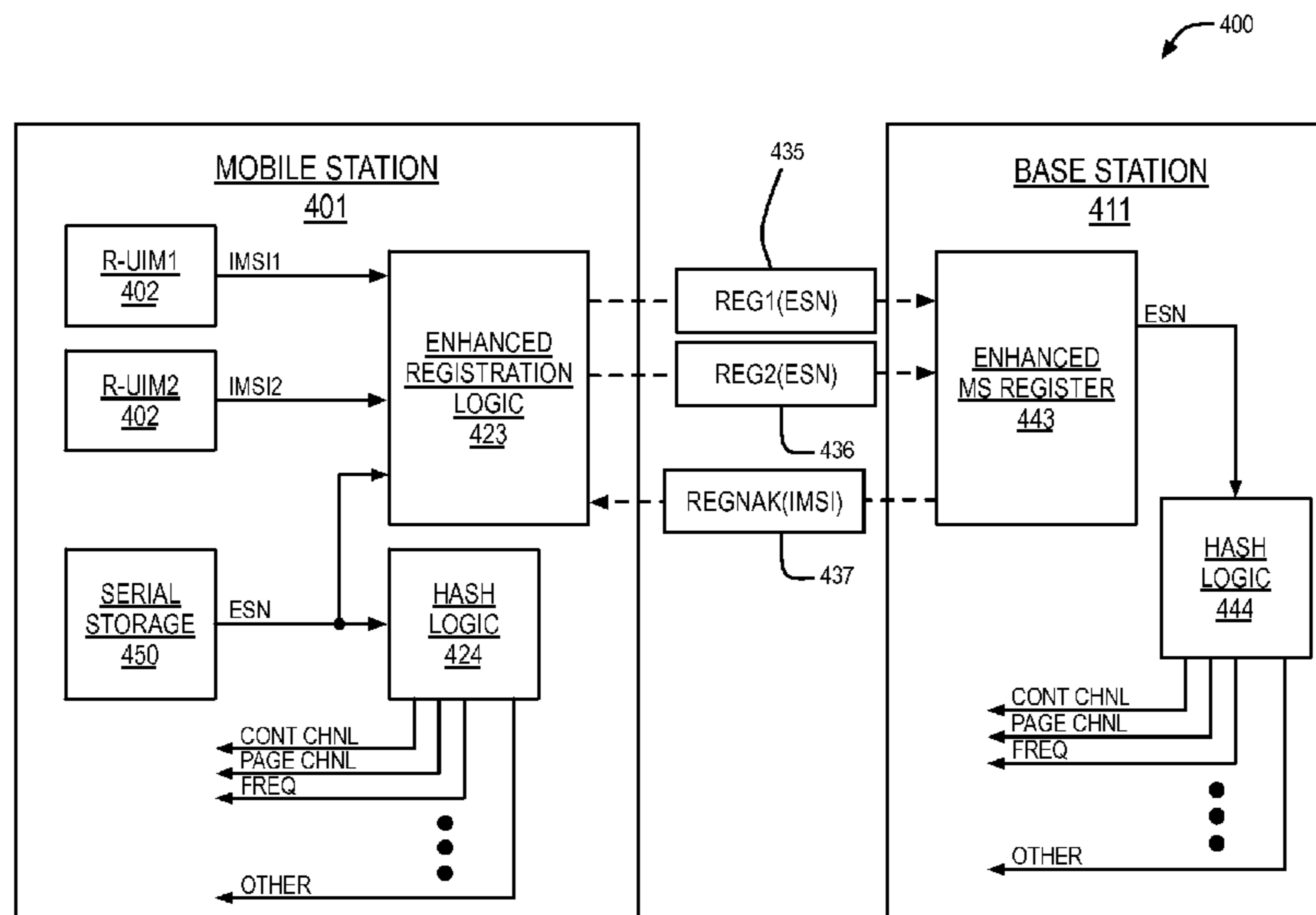
ESN-BASED HASH APPARATUS
