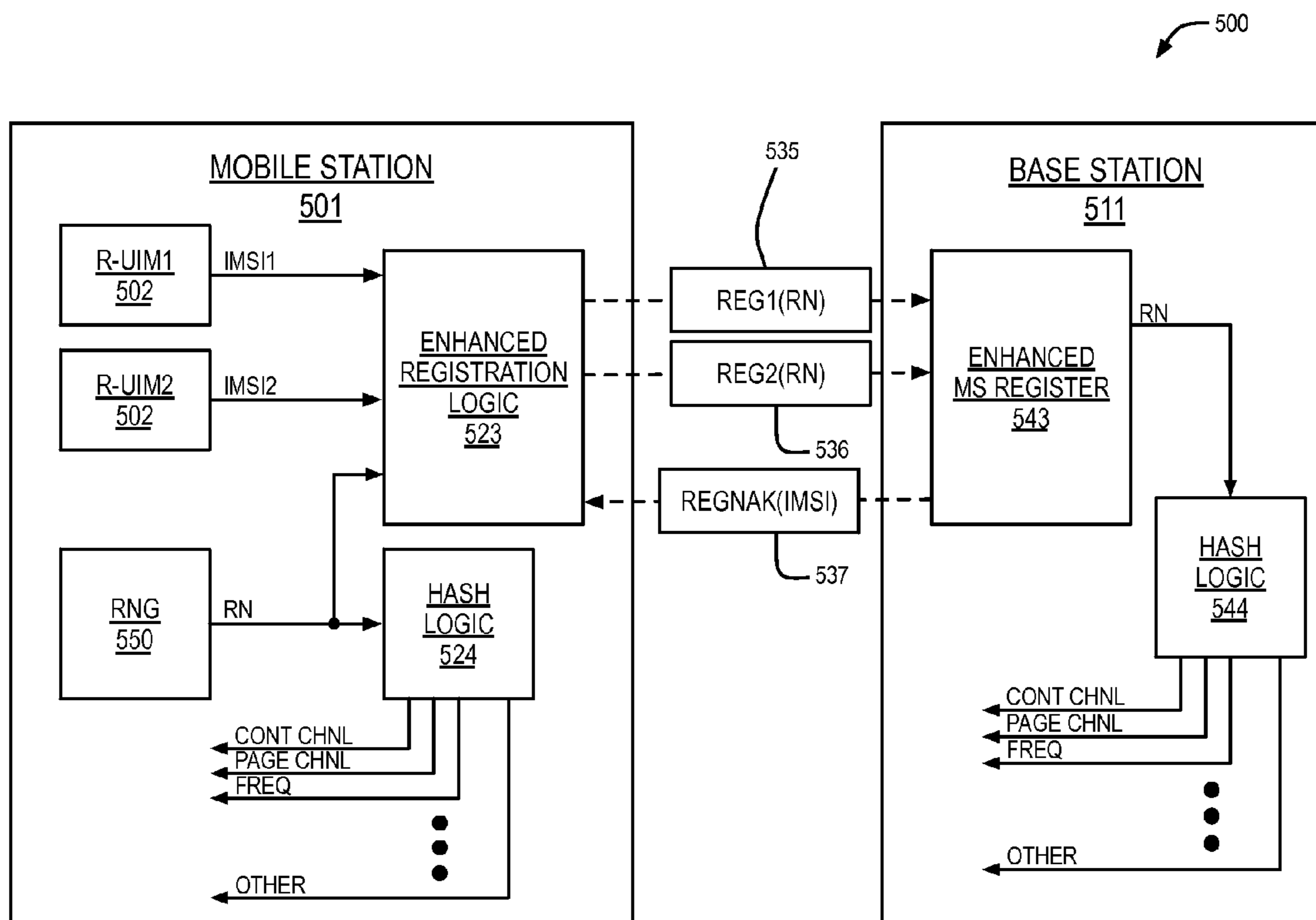
RANDOM NUMBER HASH APPARATUS
