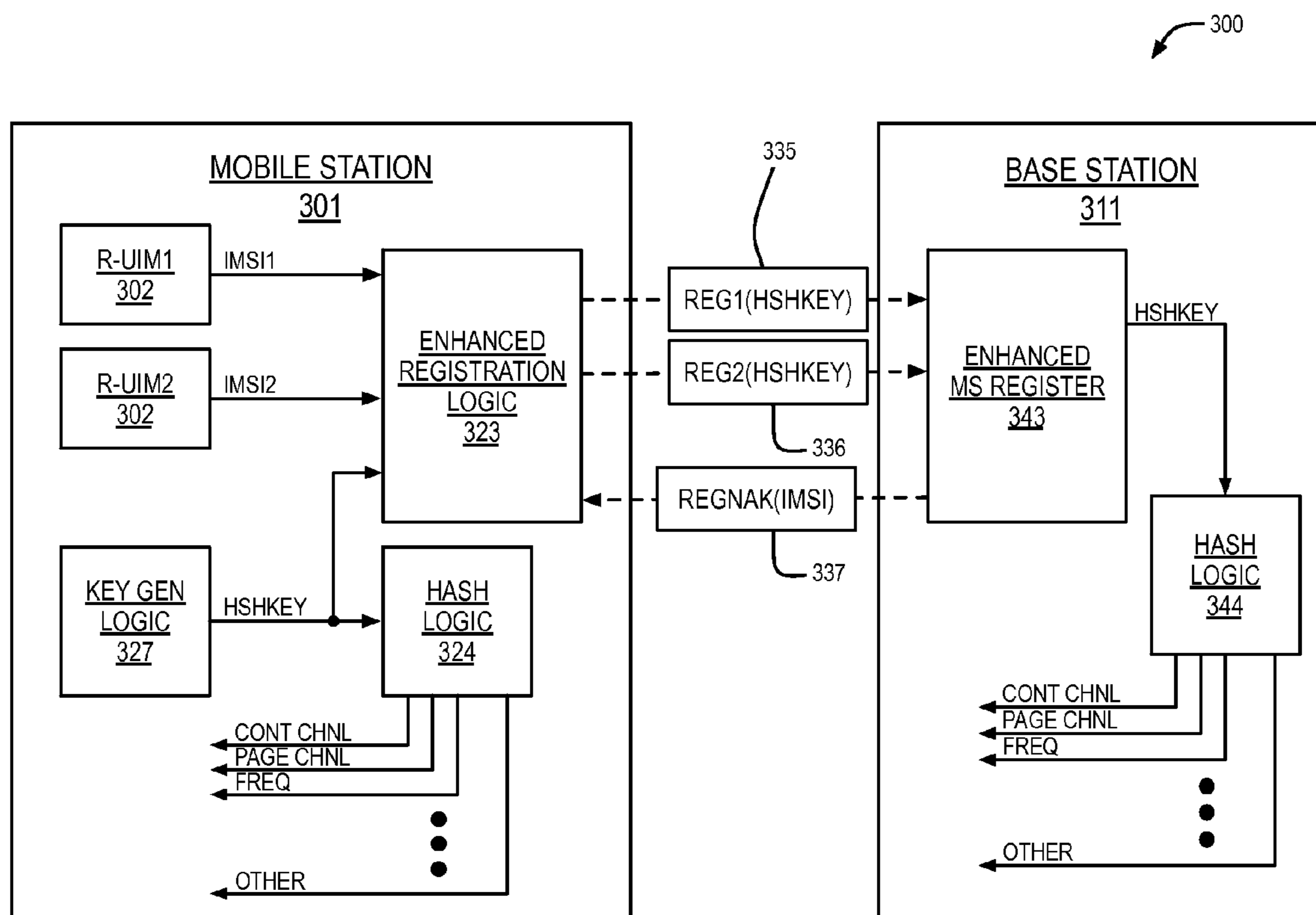
IMSI-INDEPENDENT HASH APPARATUS
