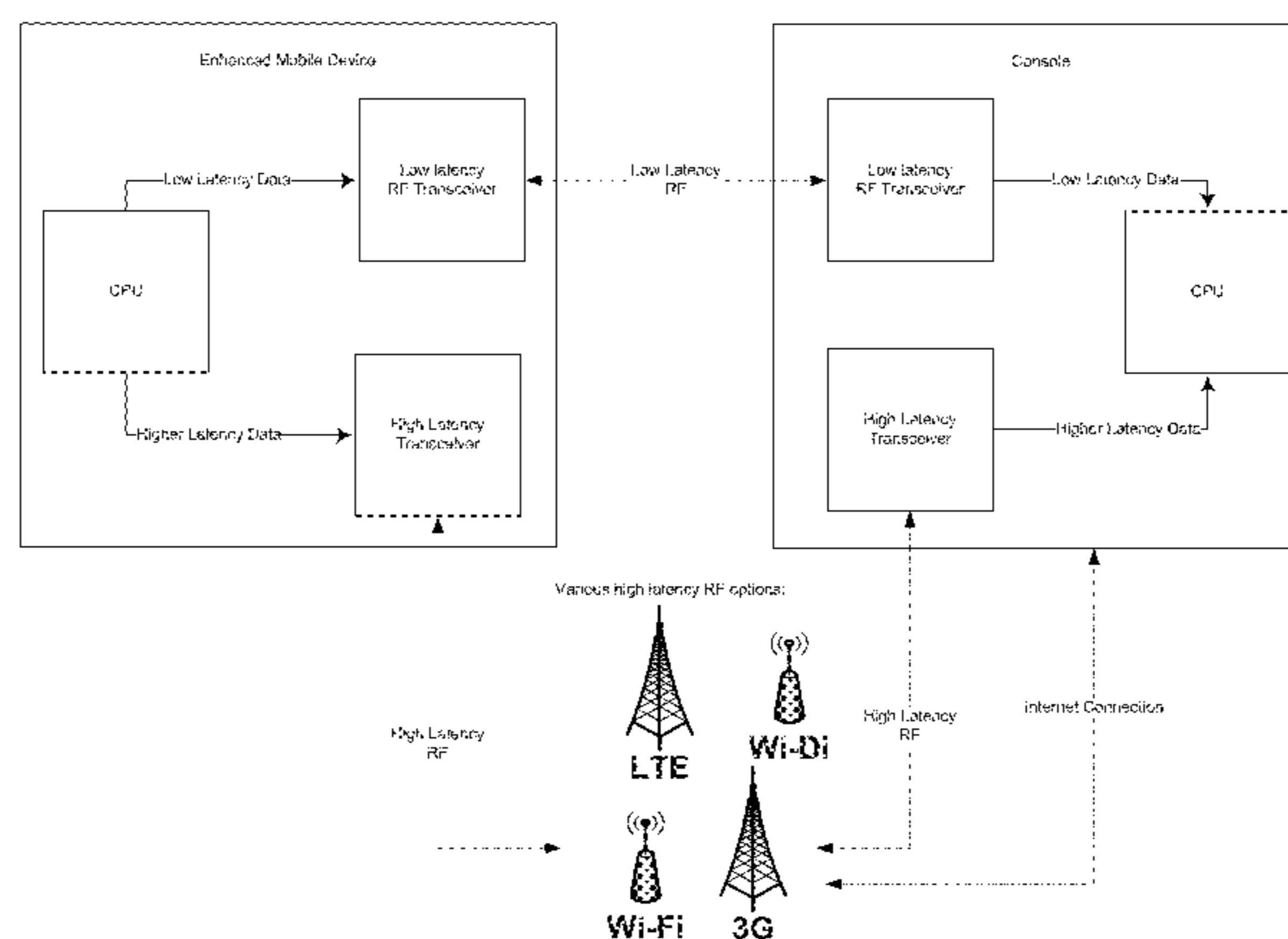
Dual-Mode Mobile Device Communication
