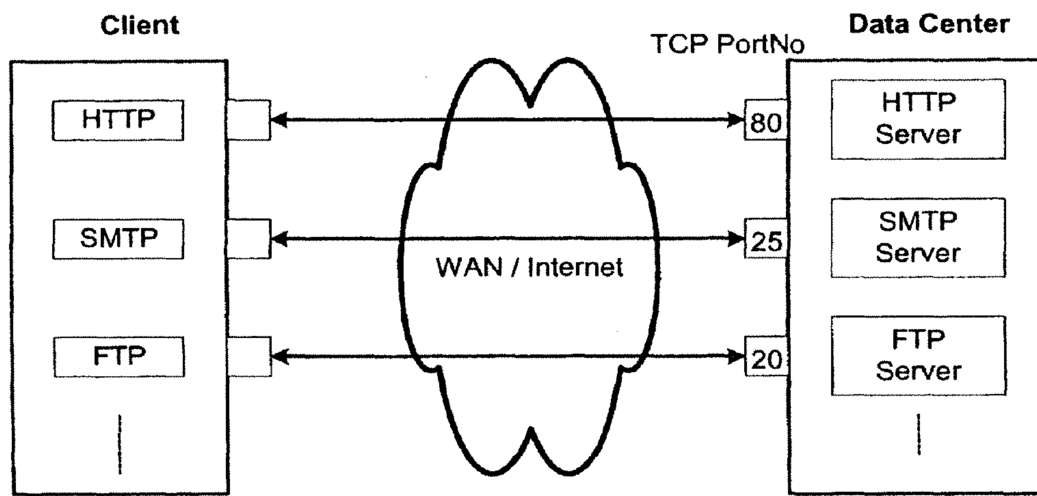
Well-Known TCP port (Softport) Connections
