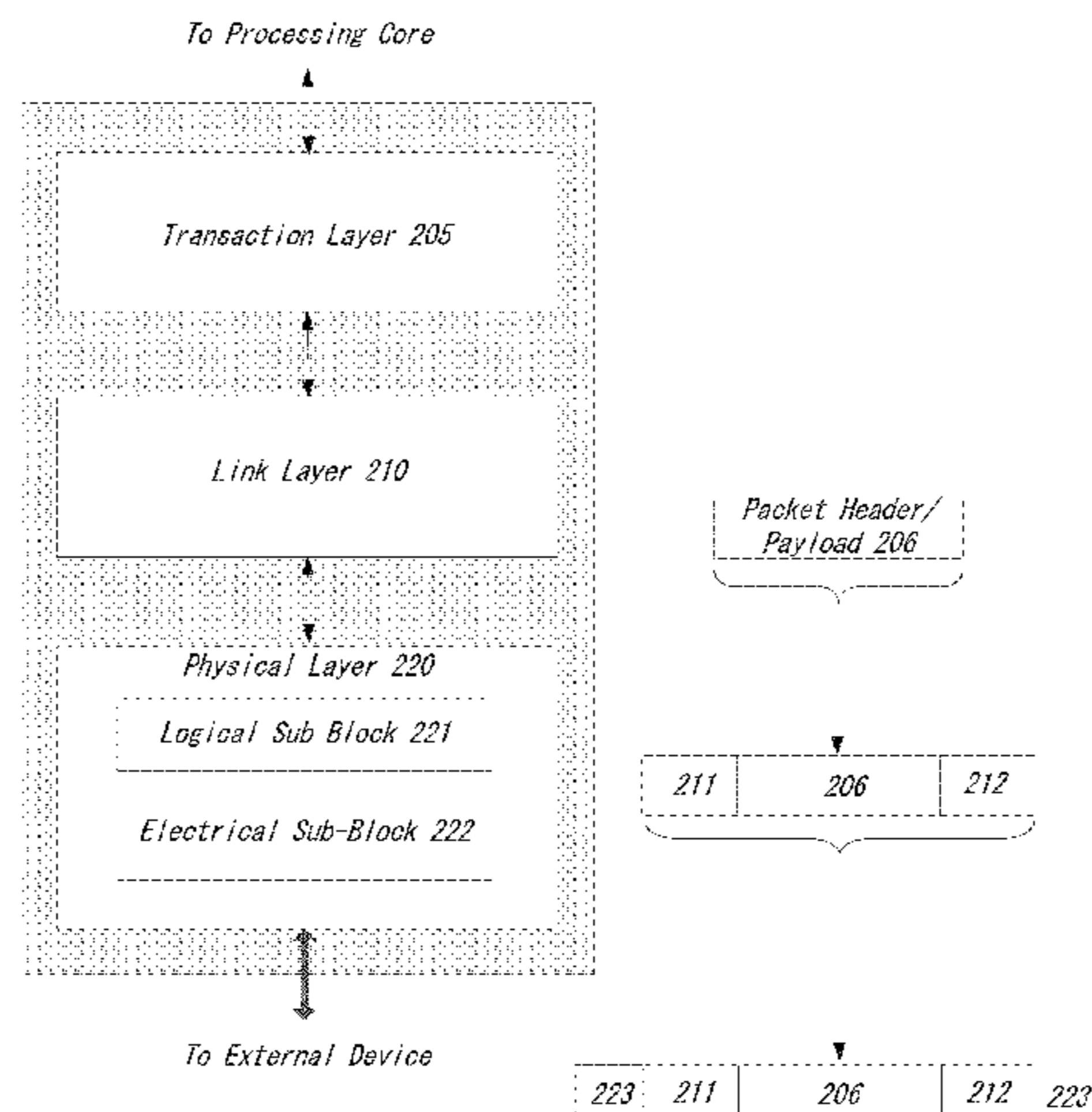
Layered Protocol Stack 200
