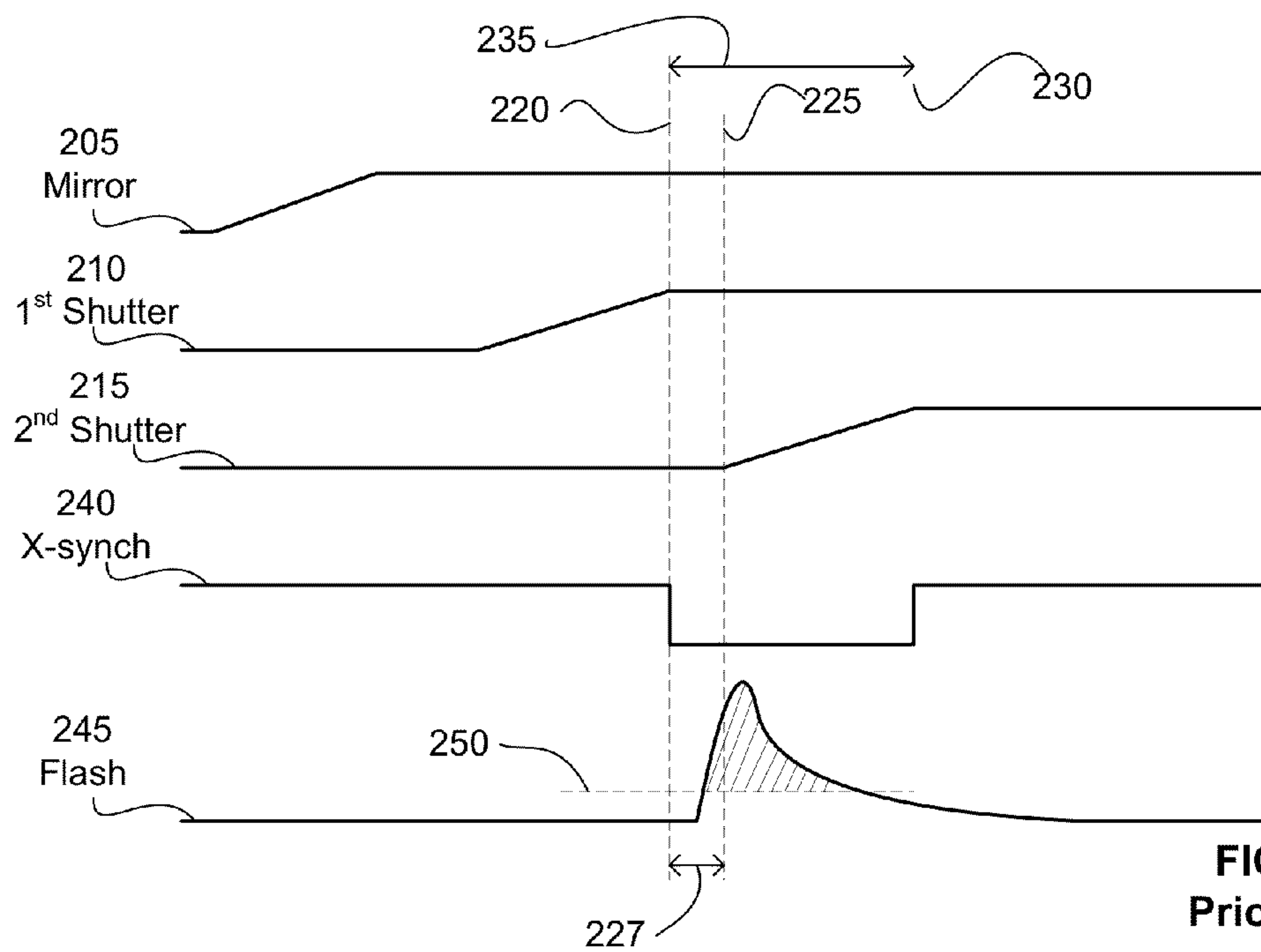
FIG. 1 Prior Art
