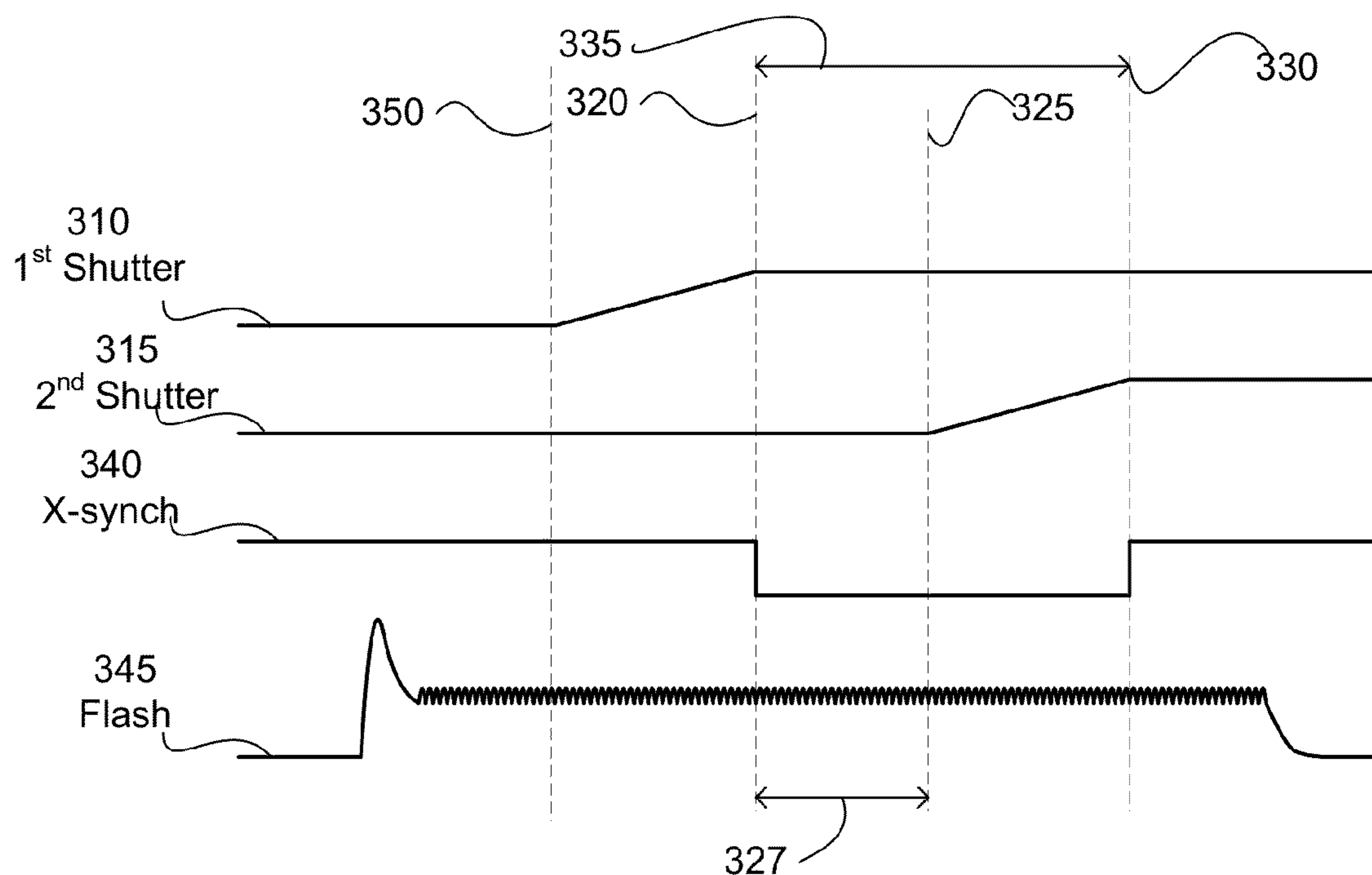
FIG. 3 Prior Art
