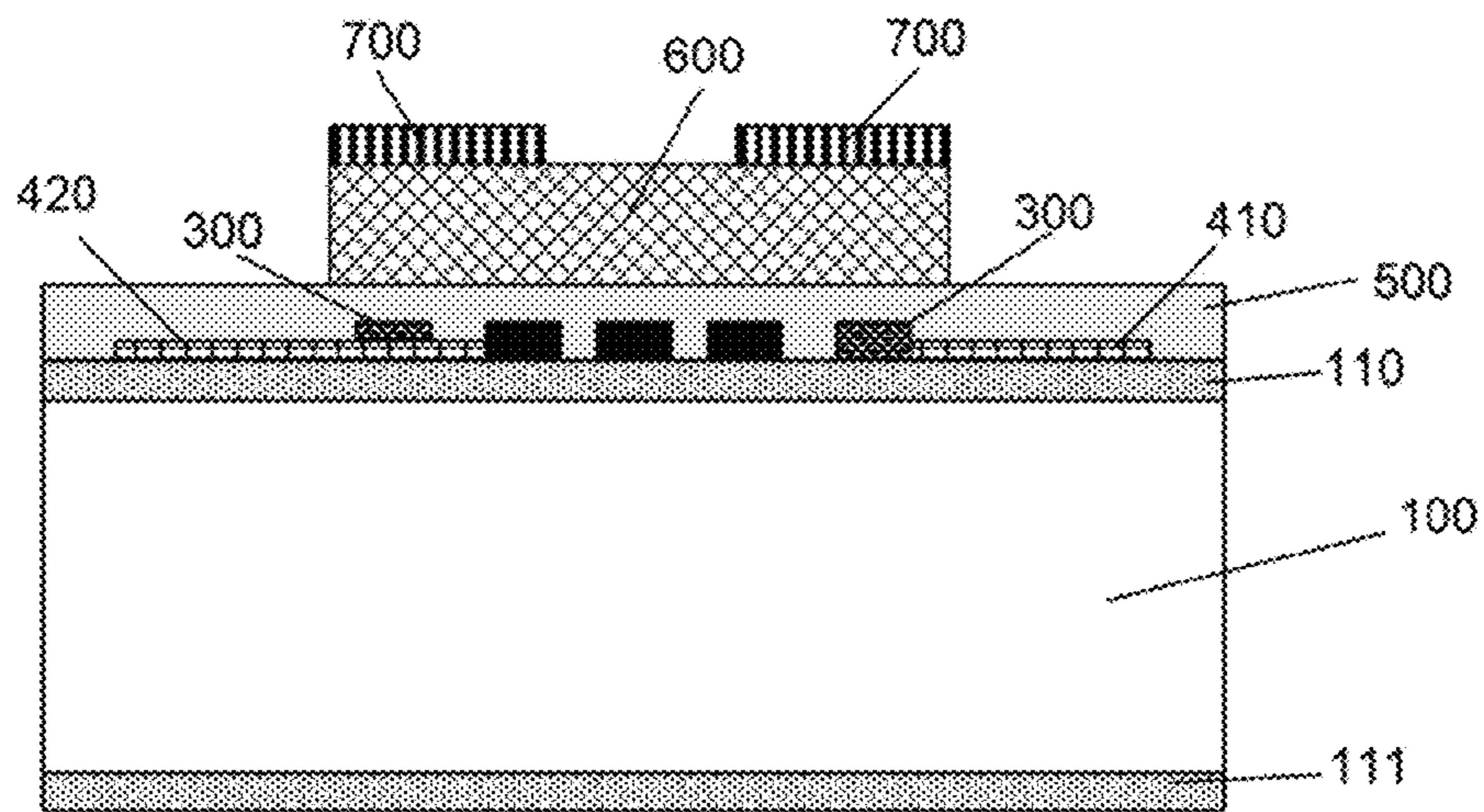
FIG 7. Form electrodes.
