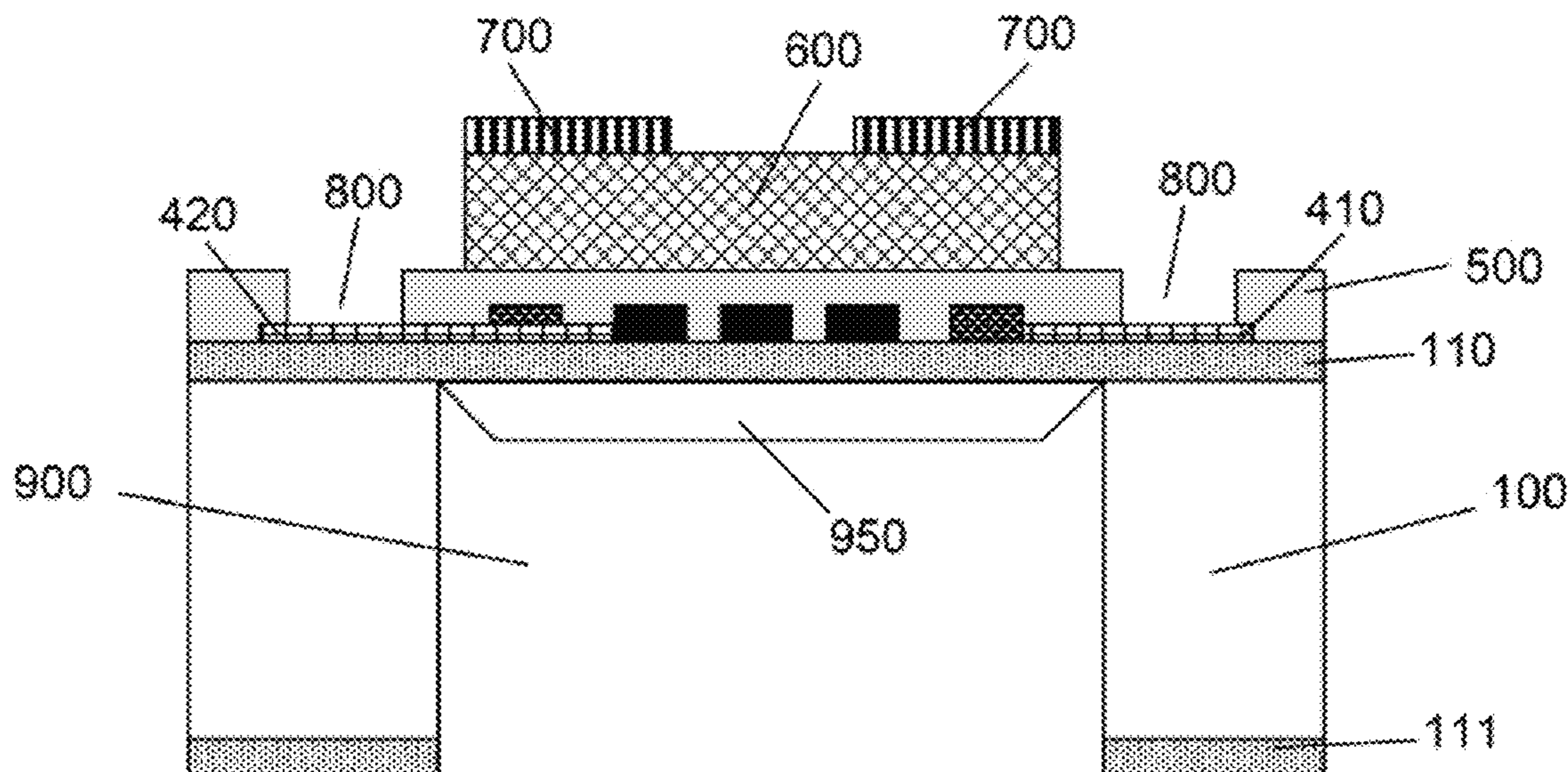
Form air isolation/cavity with a silicon plug.
