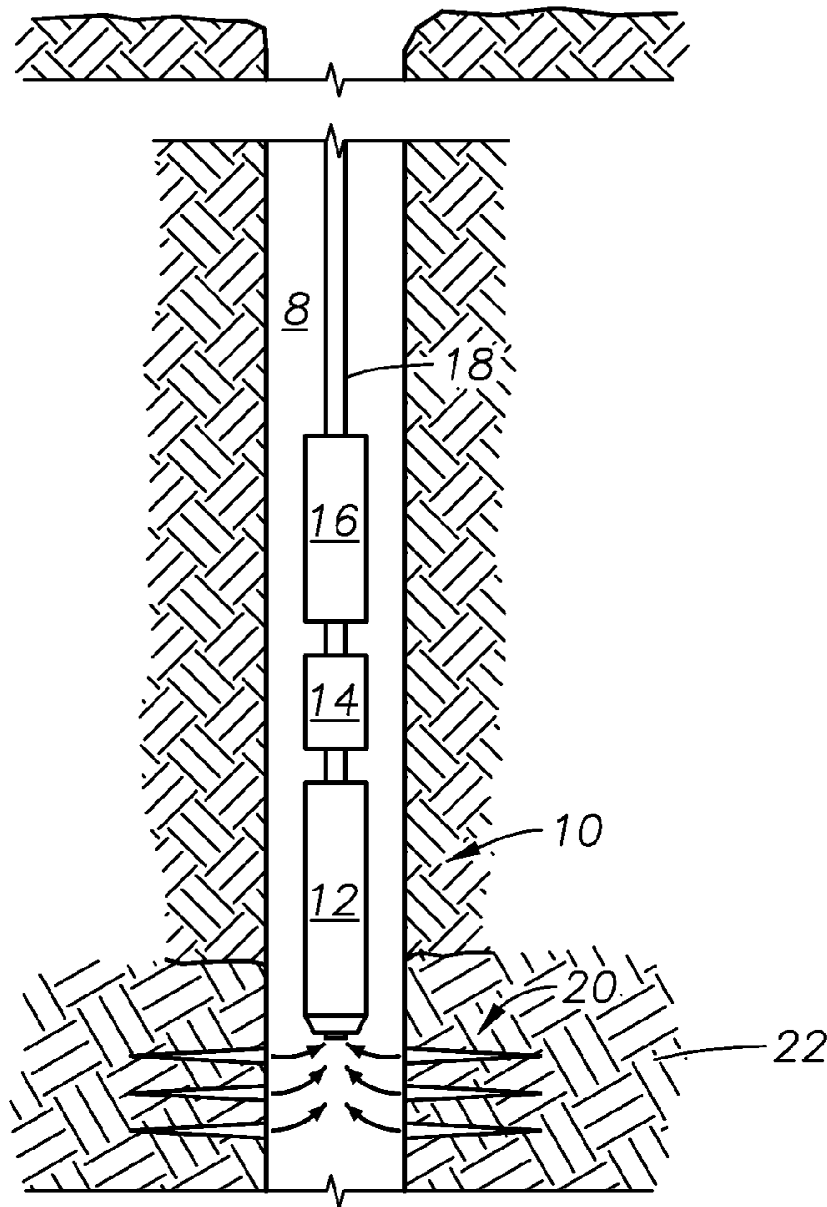
Fig. 1 (Prior Art)
