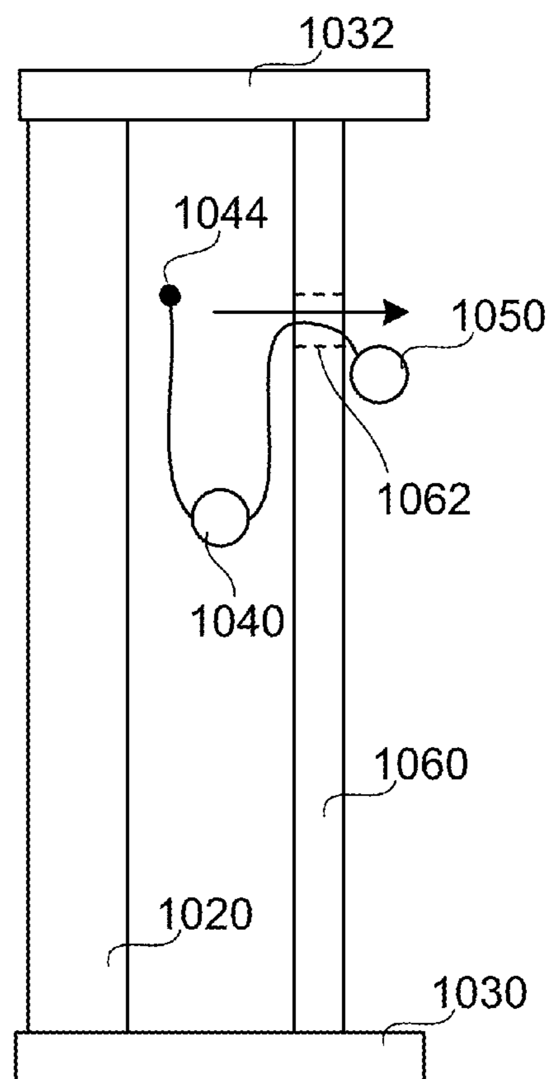
Fig. 14B Venting
