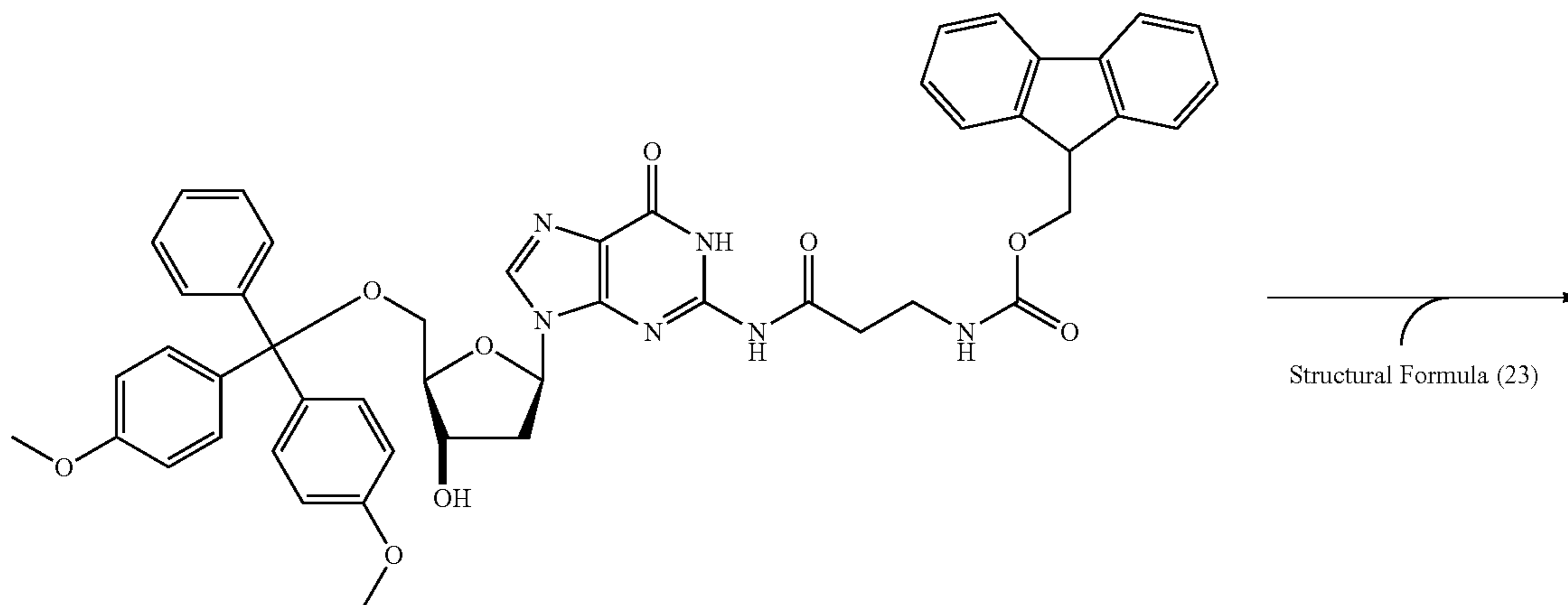
Structural Formula (10)
