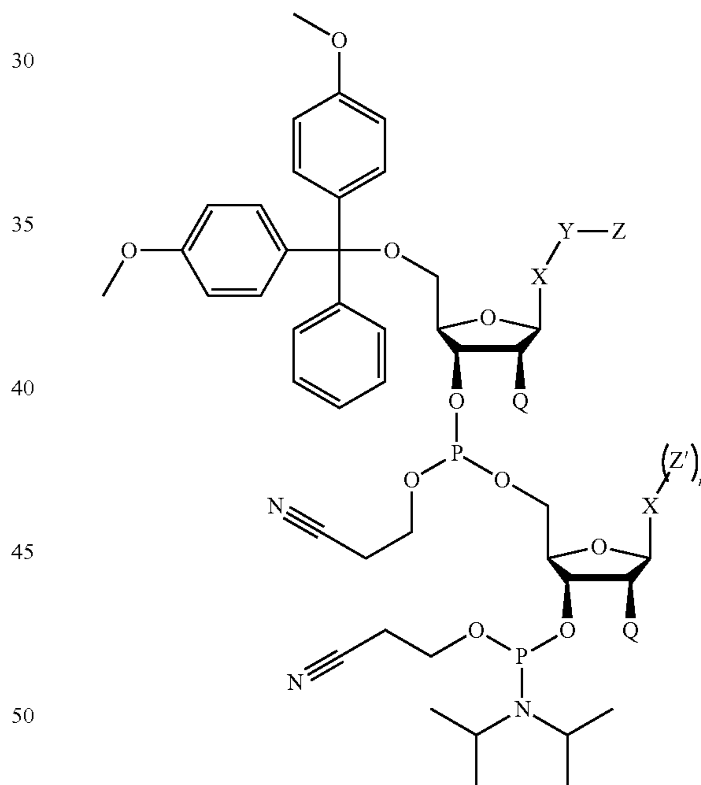
Formula (IV)
