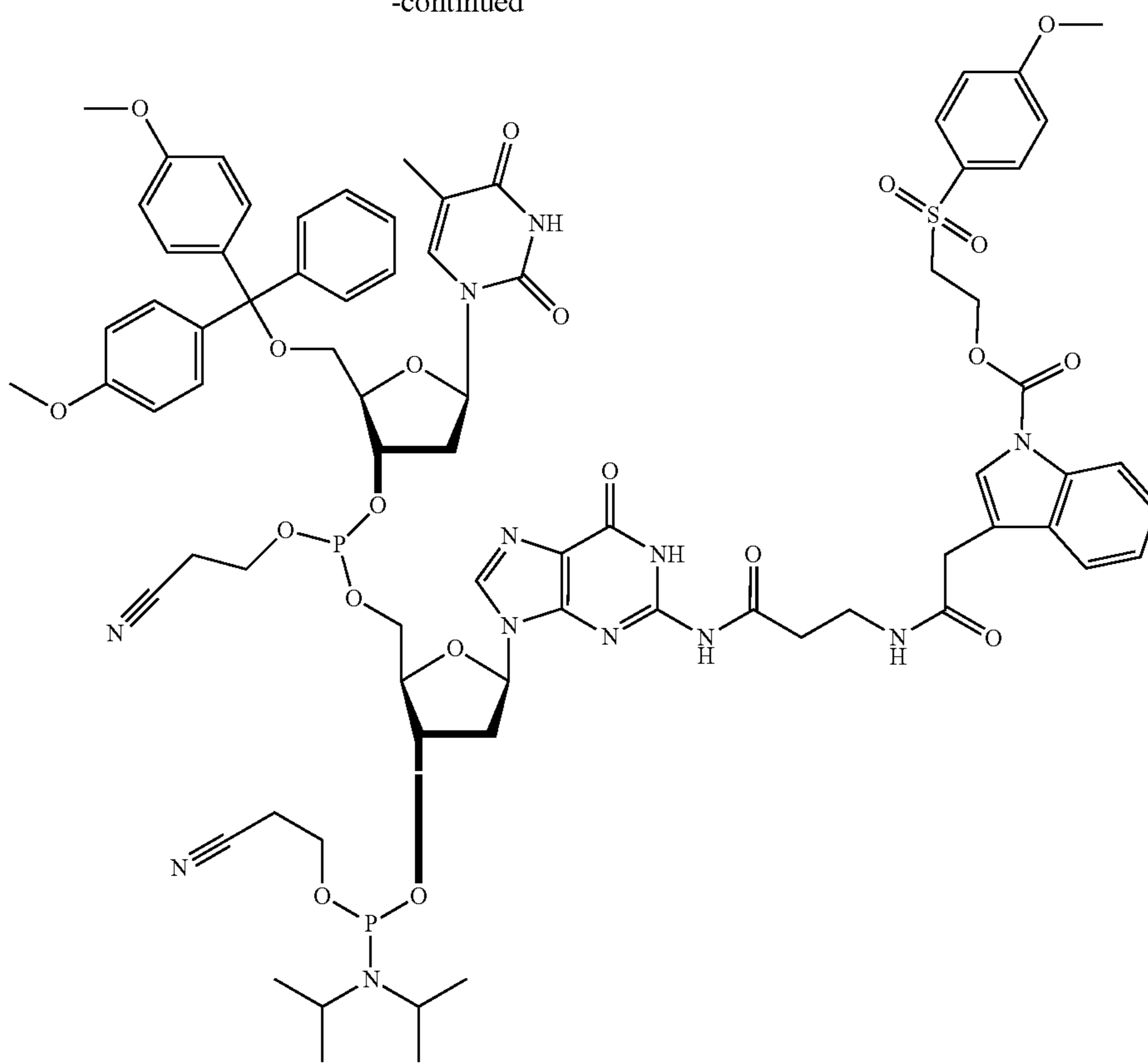
Structural Formula (2)
