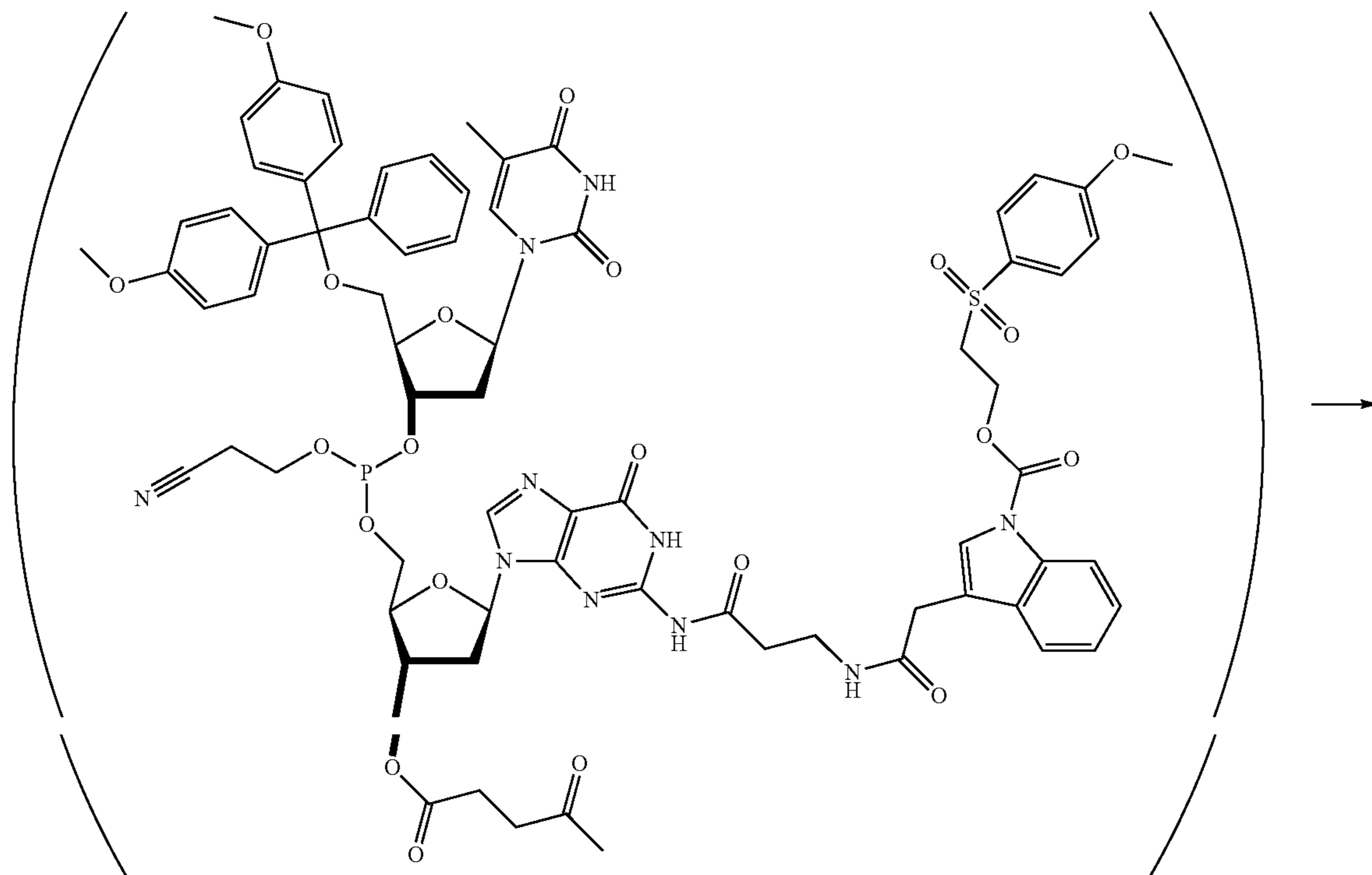
Structural Formula (7')
