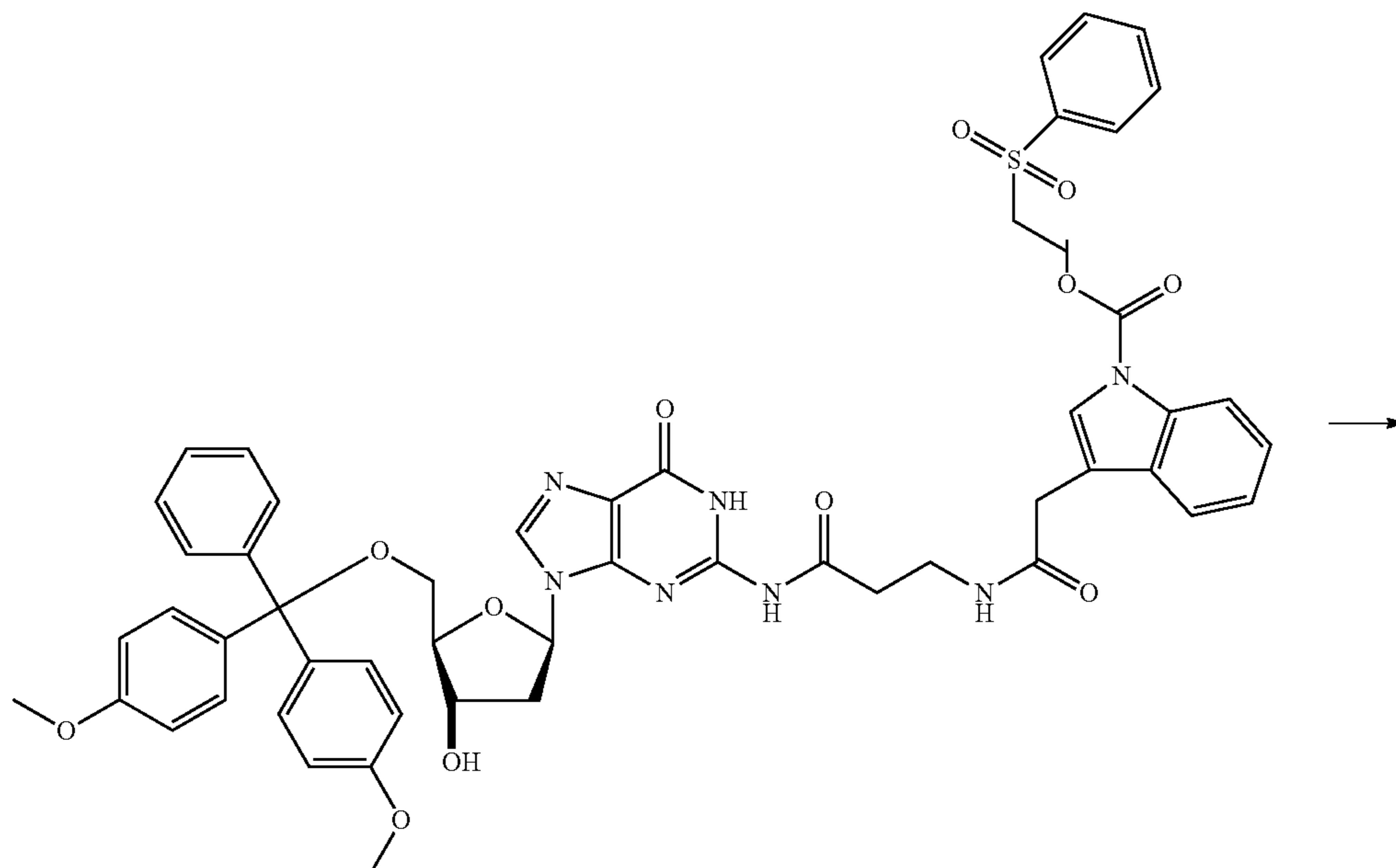
Structural Formula (24)
