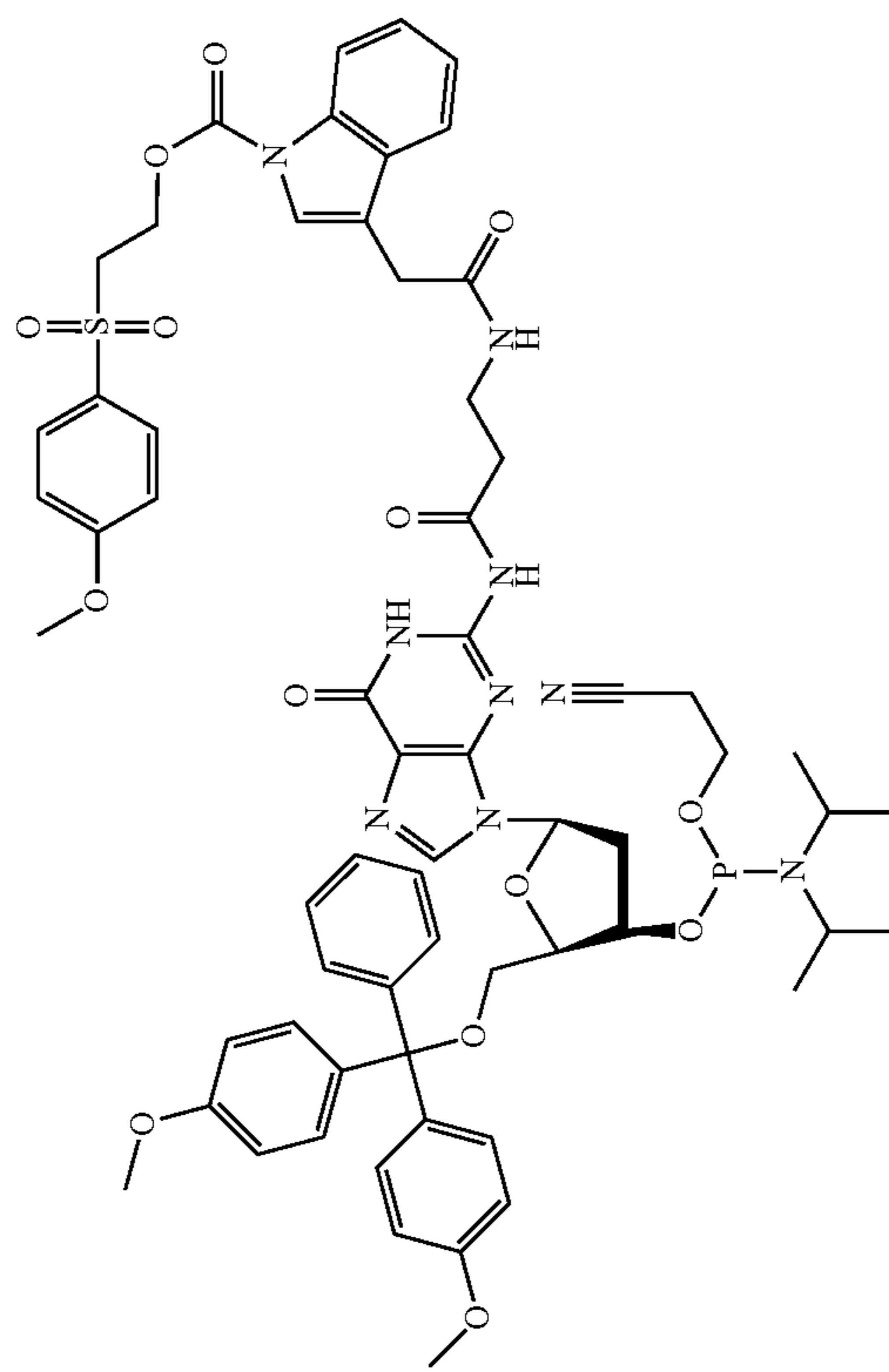
Structural Formula (1)
