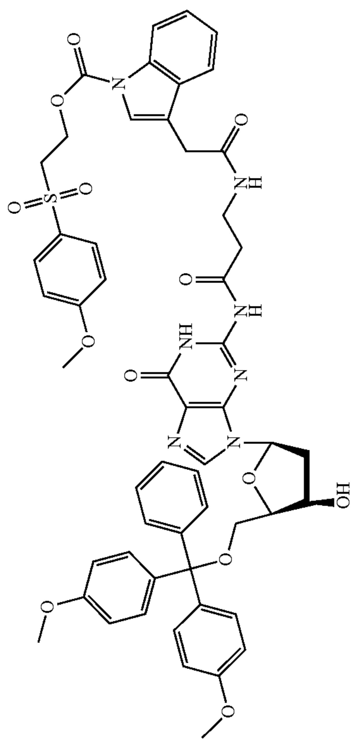
Structural Formula (5)
