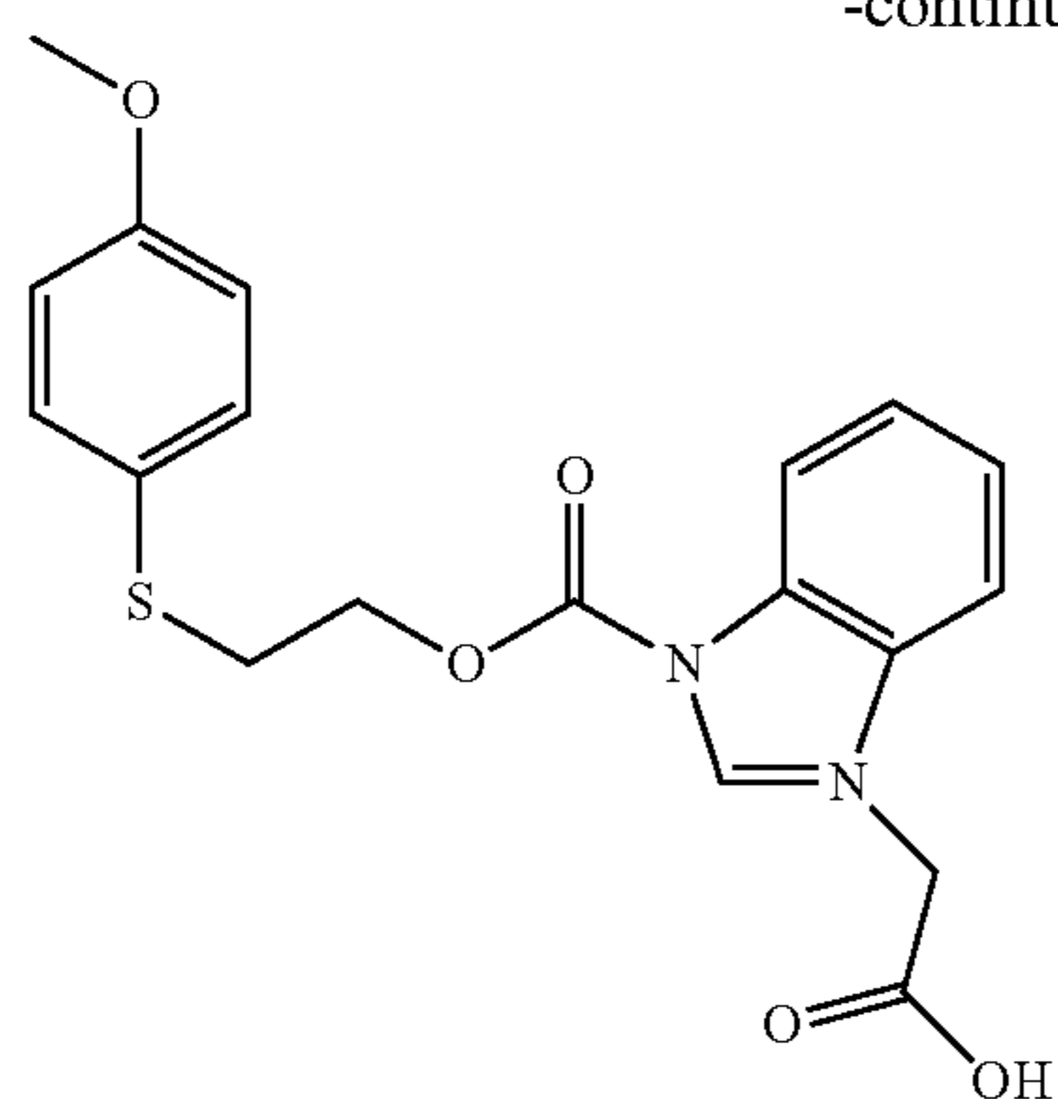
Structural Formula (3)
