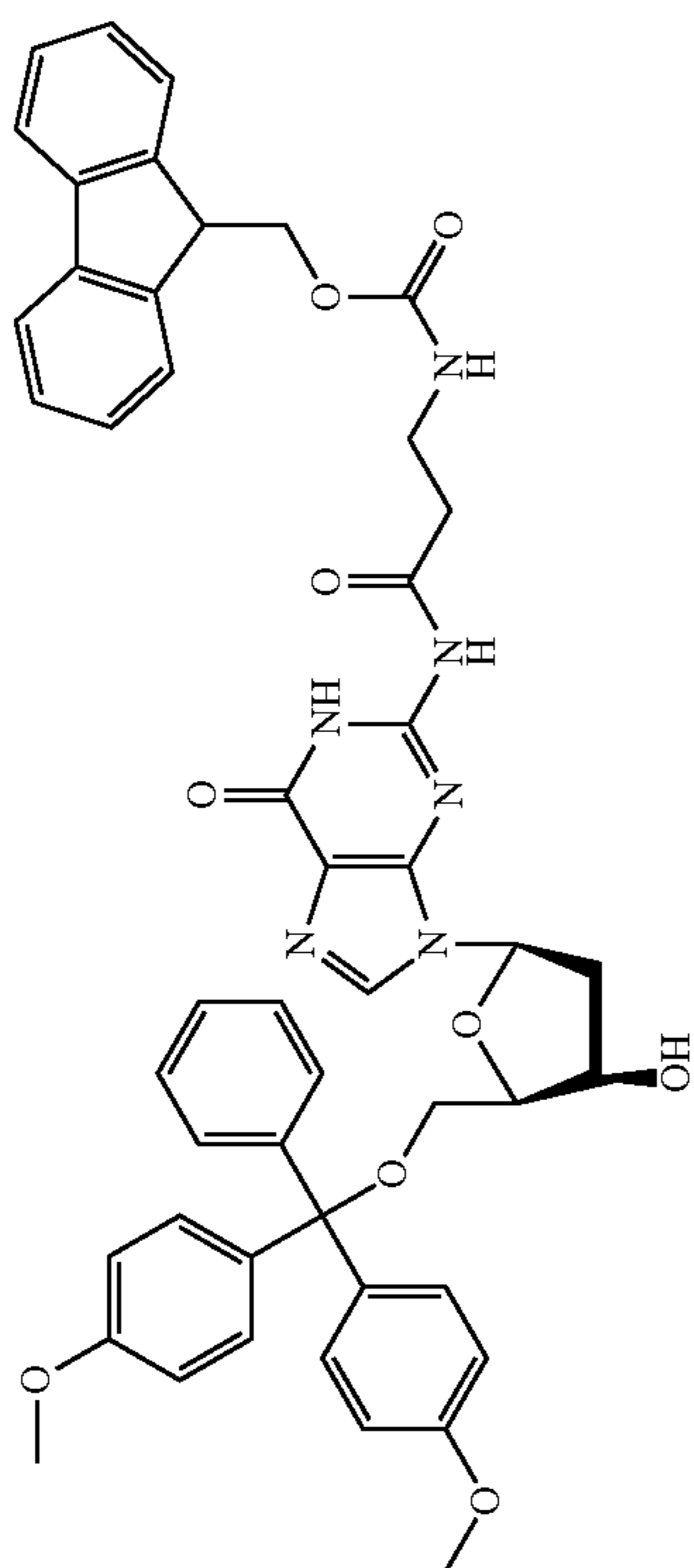
Structural Formula (10)
