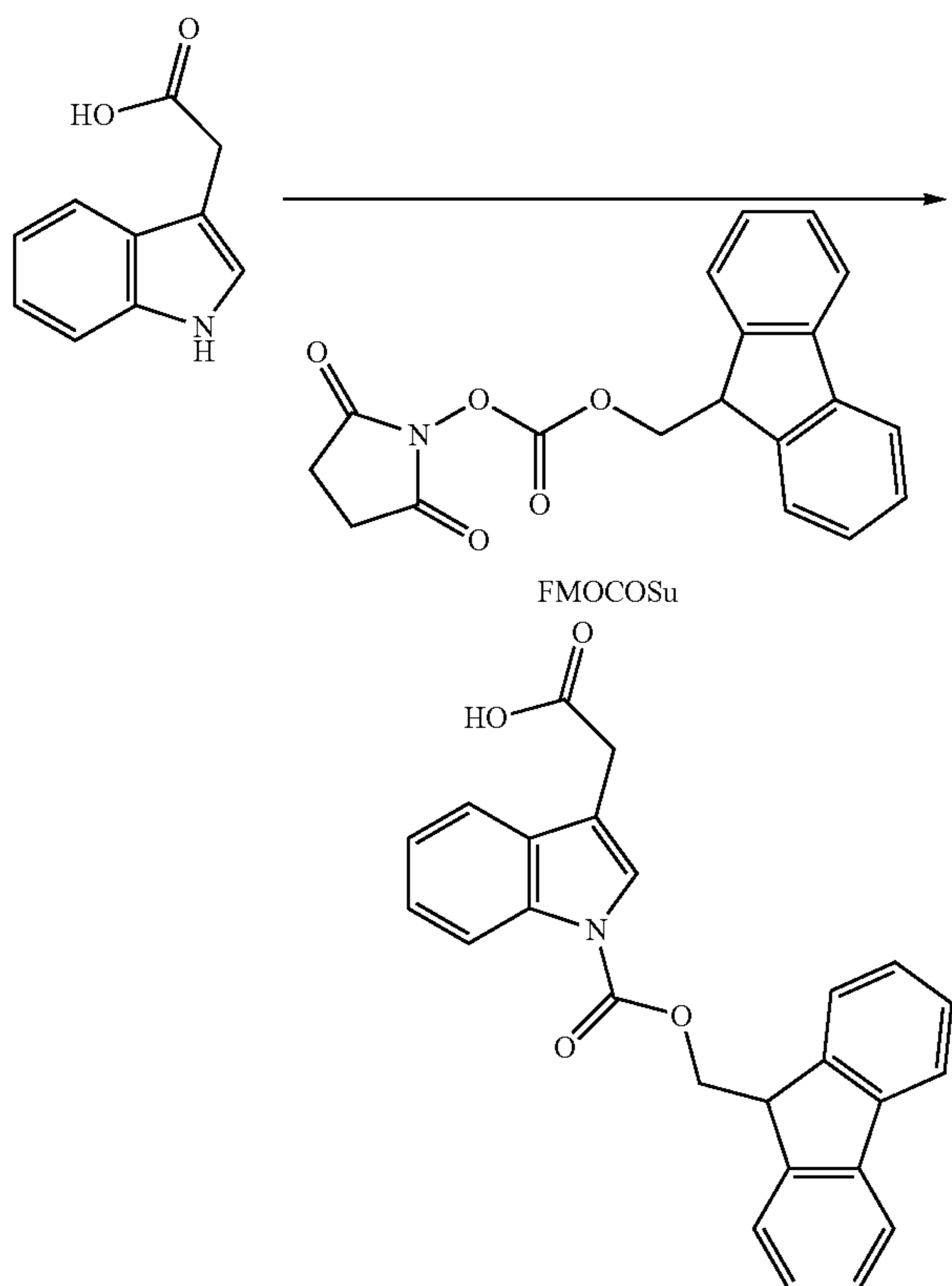
Structural Formula (26)
