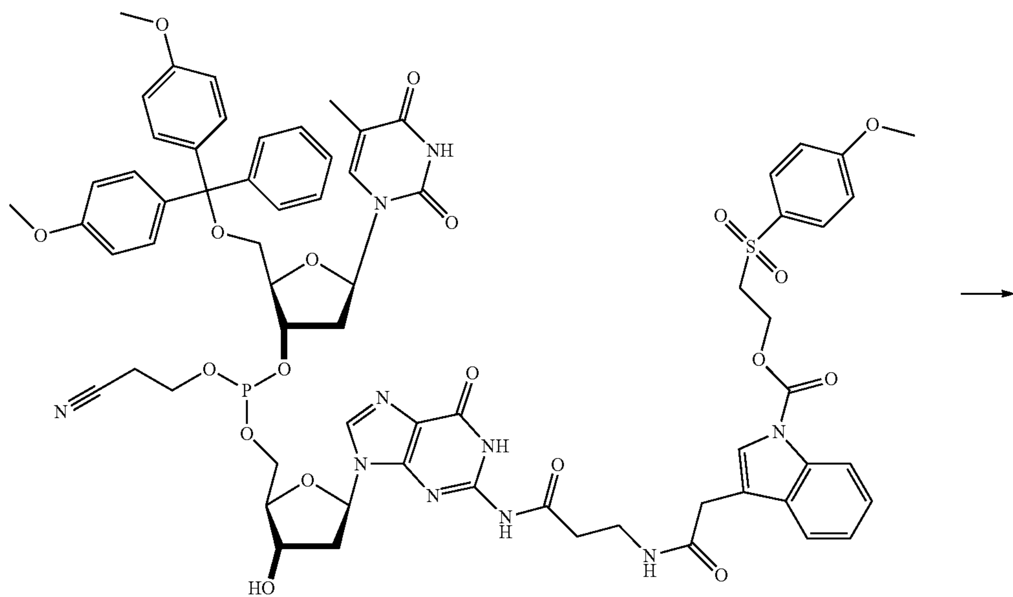
Structural Formula (7)
