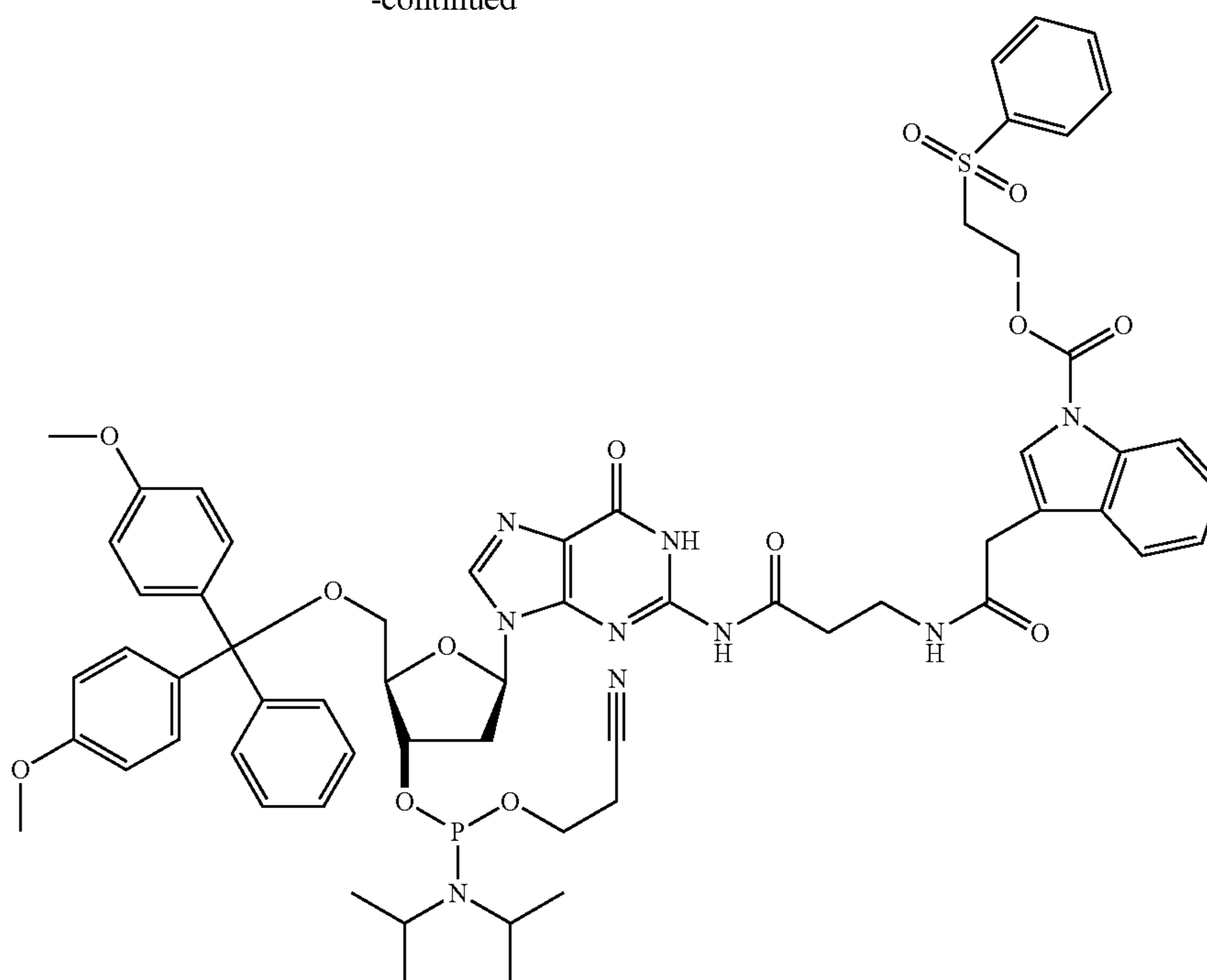
Structural Formula (25)
