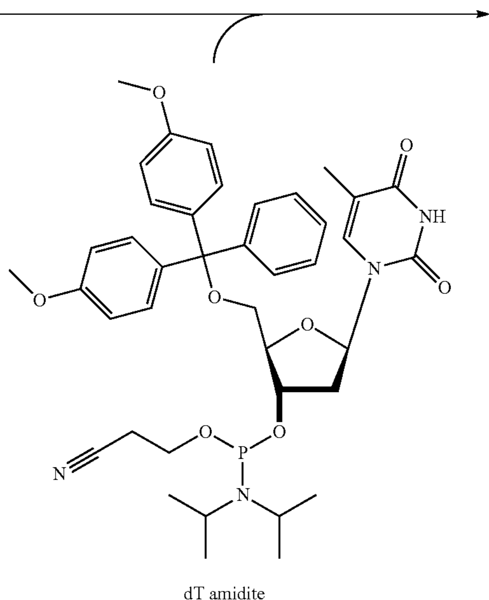
Structural Formula (6)
