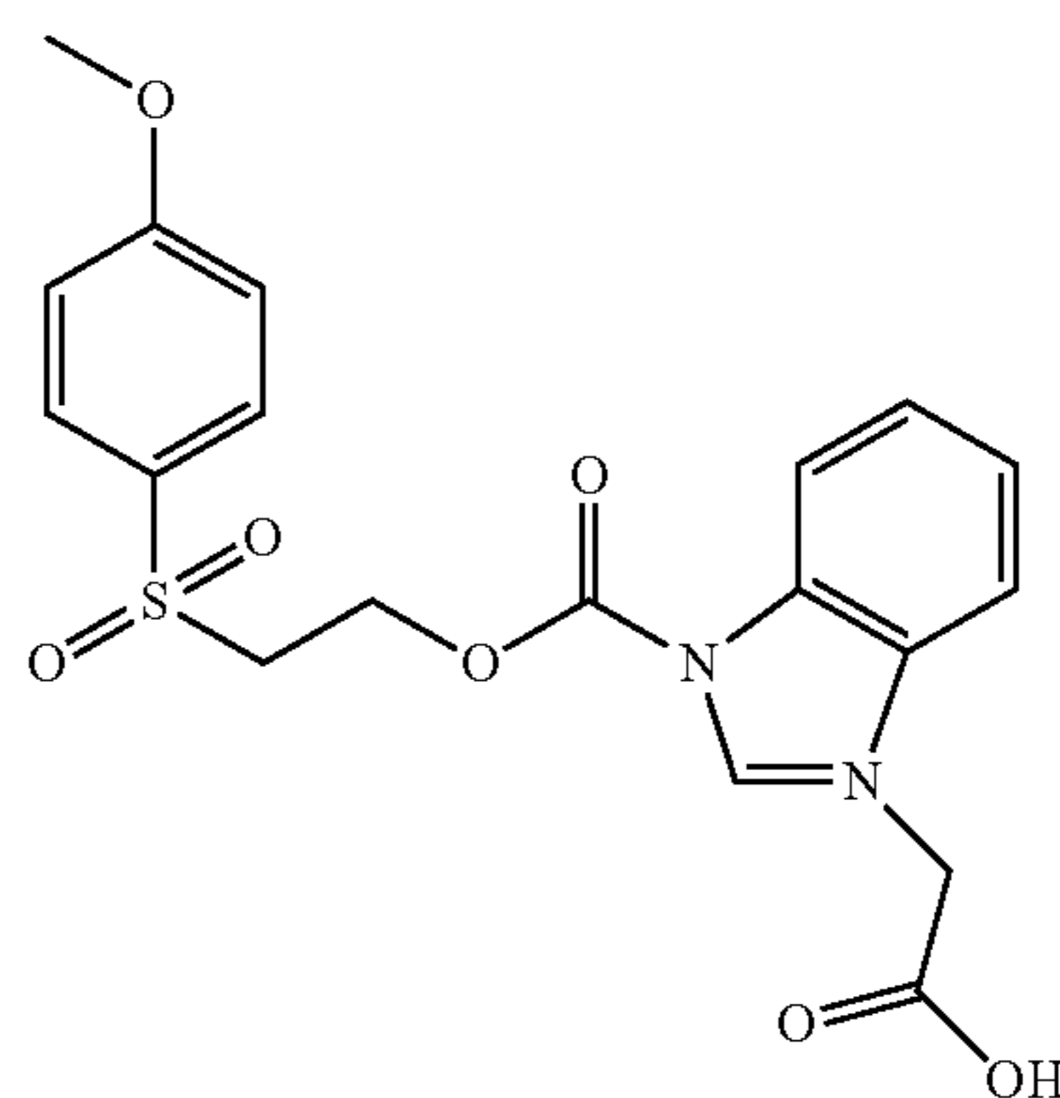
Structural Formula (4)
