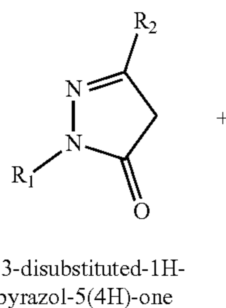
Scheme 2 General pathway to prepare Formula 2 related compounds
