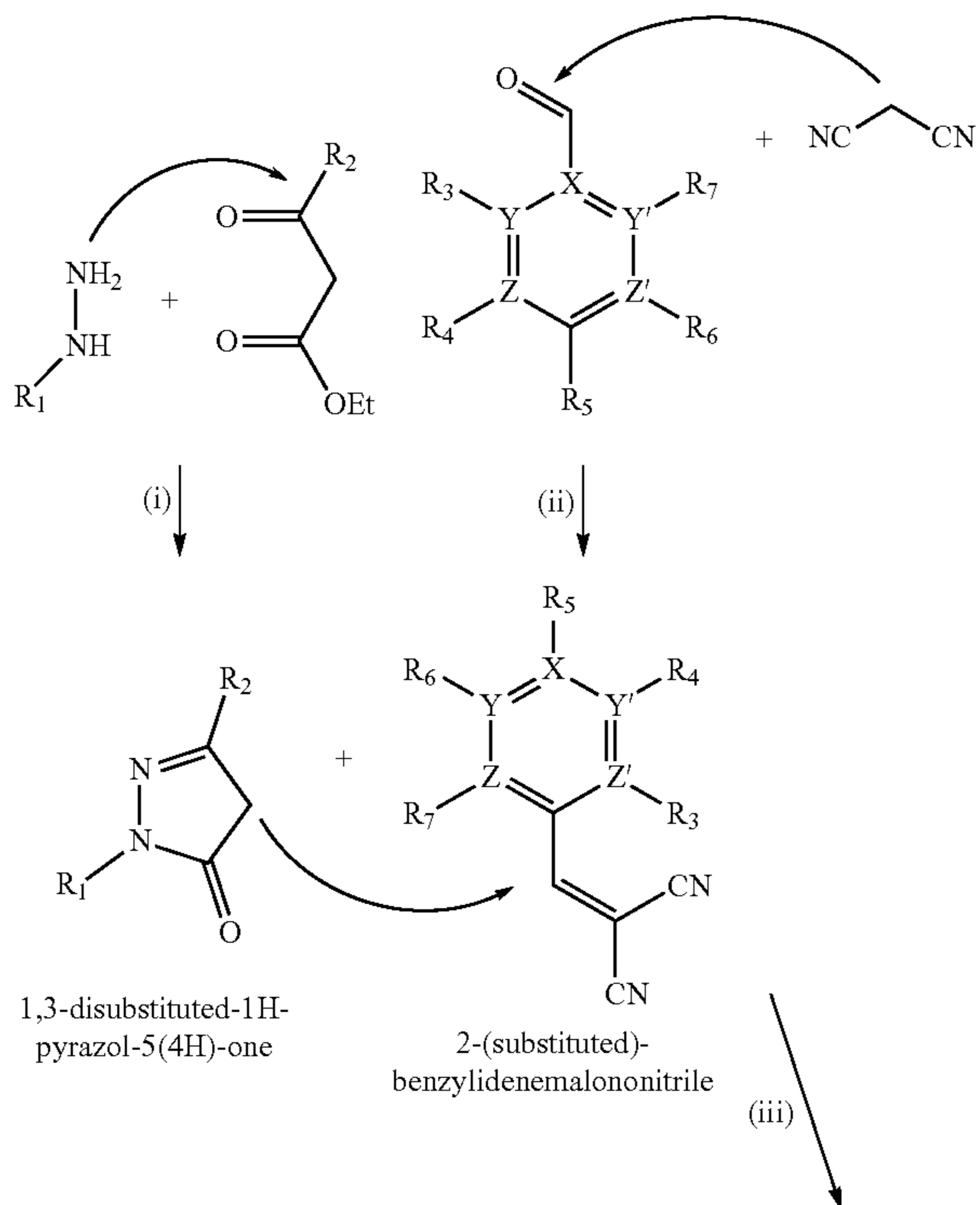
Scheme 1 General pathway to prepare Formula 1 related compounds
