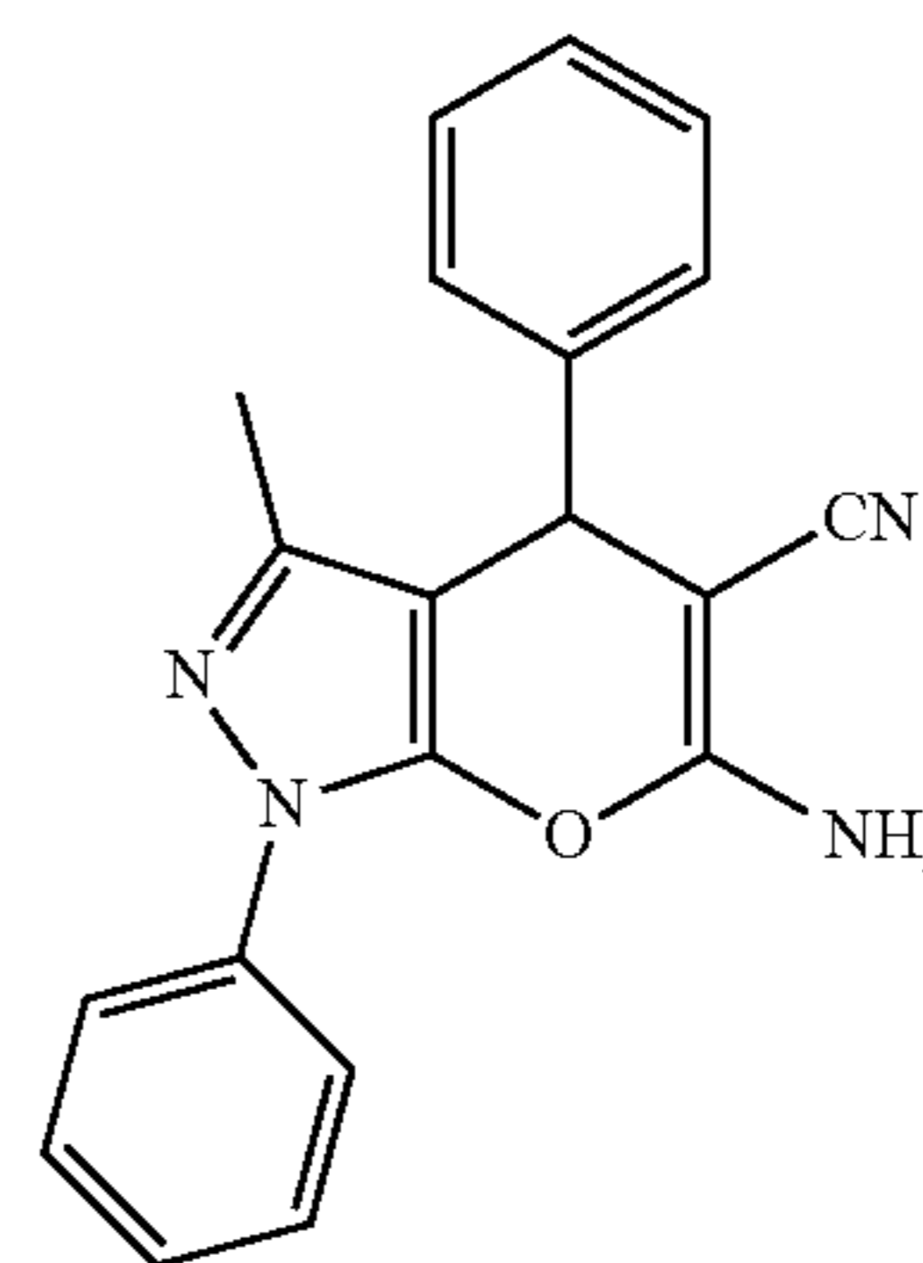
Chemical Formula: C 20 H 16 N 4 O Molecular Weight: 328.37
