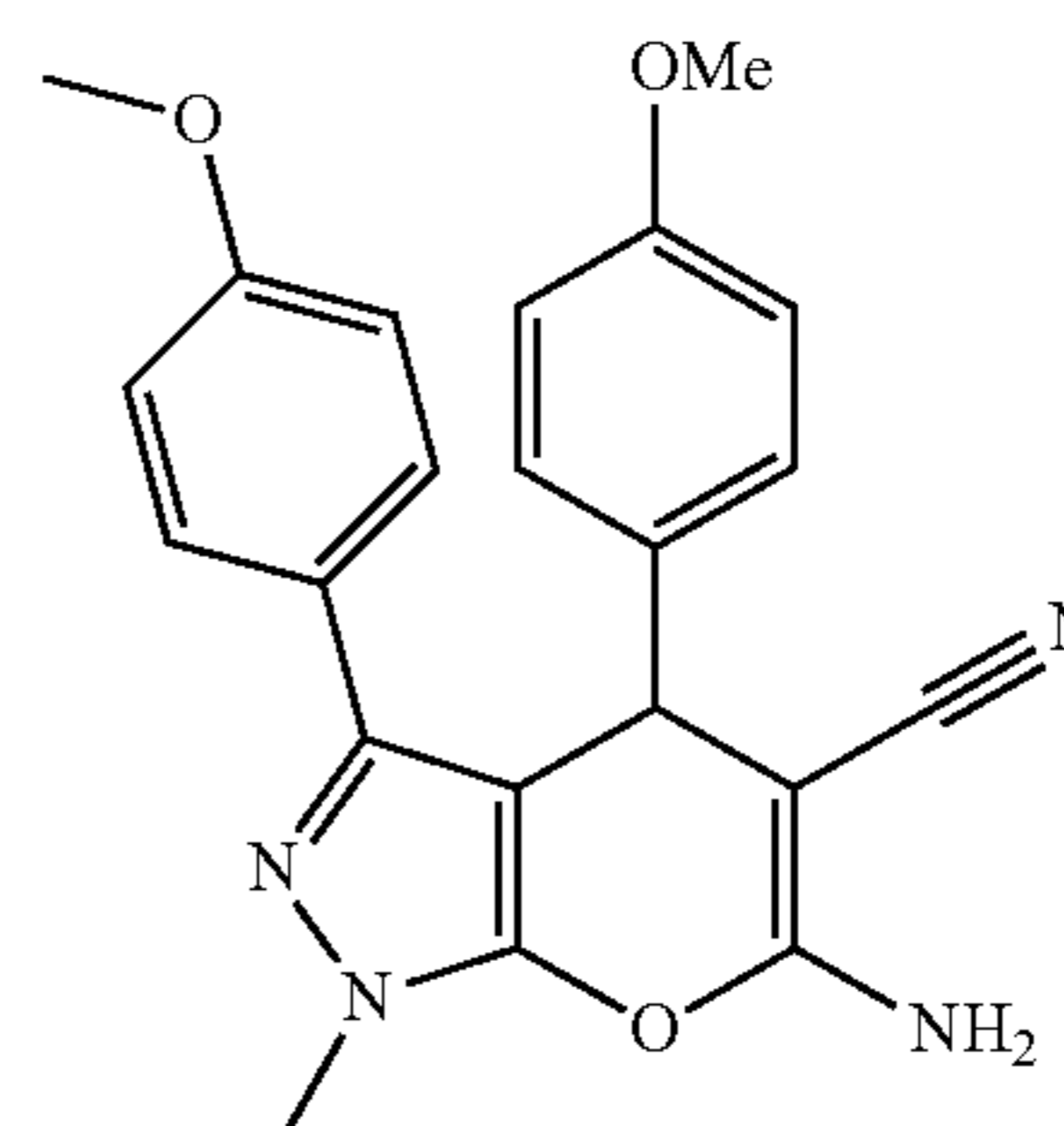
Chemical Formula: C_{22}H_{20}N_4O_3 Molecular Weight: 388.42
