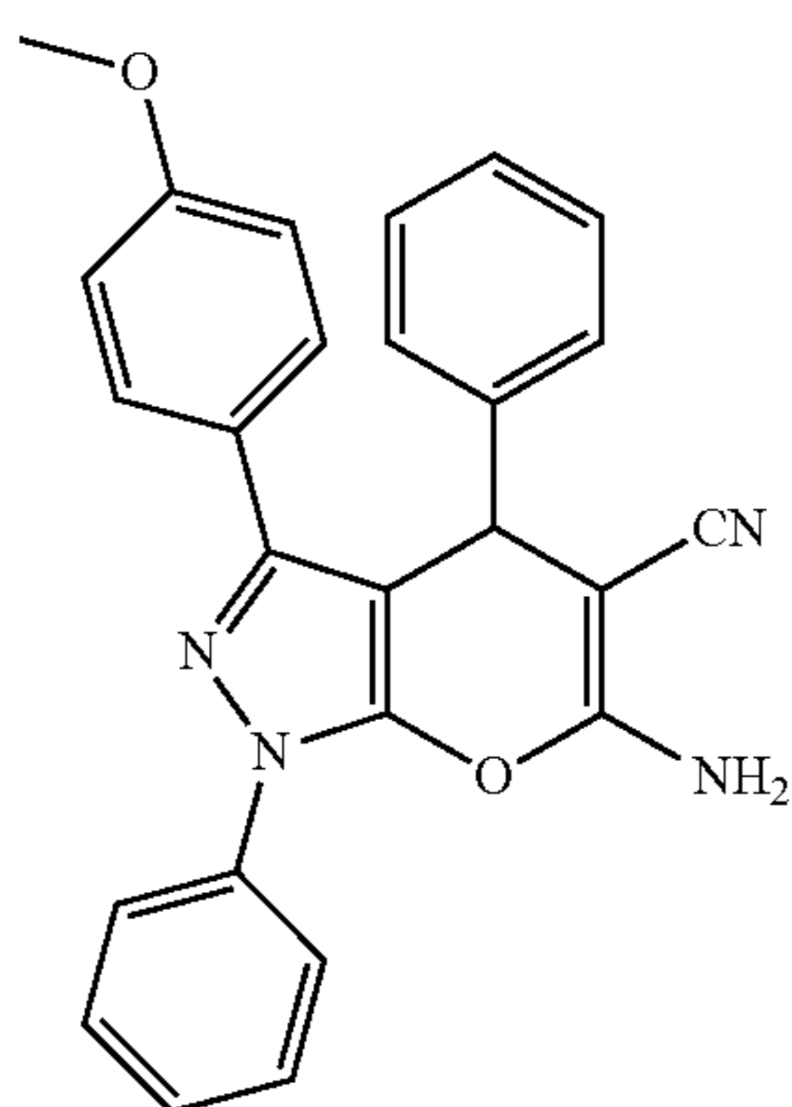
Chemical Formula: C_{26}H_{20}N_4O_2 Molecular Weight: 420.46
