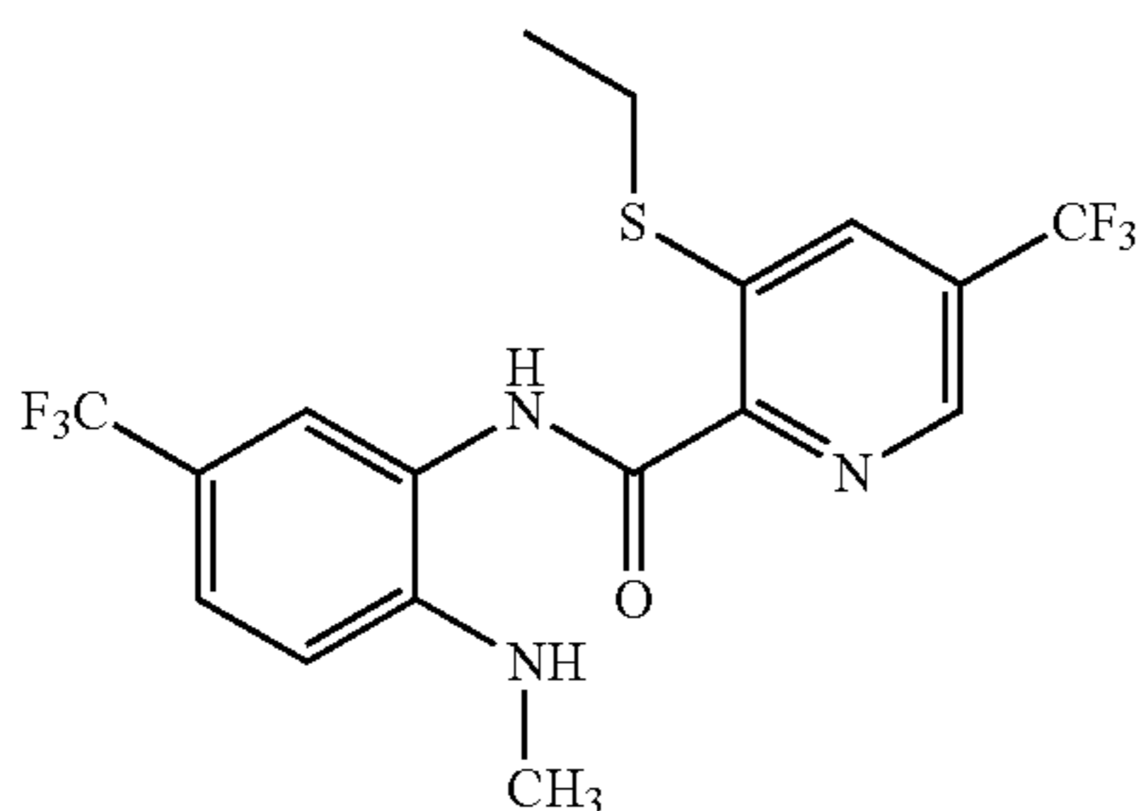
Intermediate Compound (M3-32)
