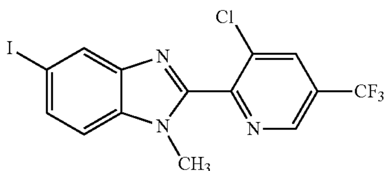
Intermediate Compound (M6-41)
