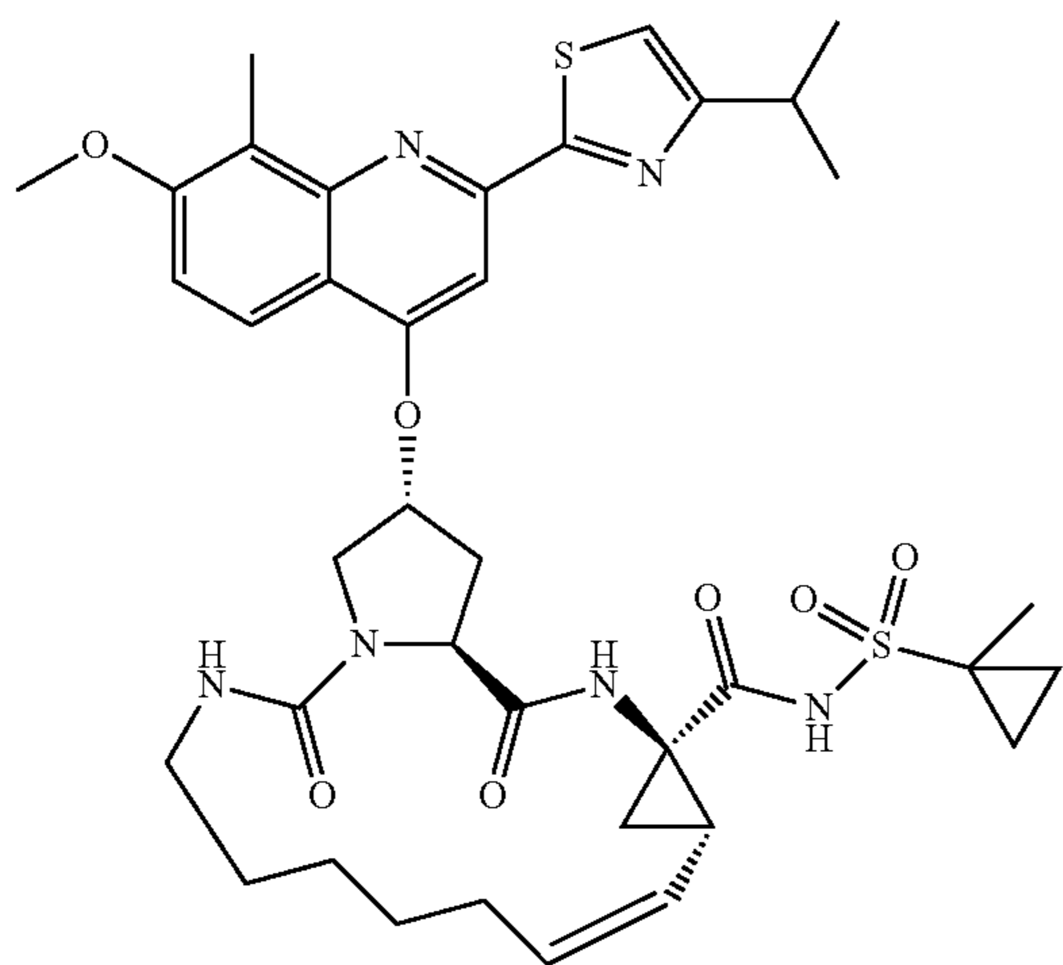
1-Methyl-cyclopropanesulfonic acid {18-[2-(4-isopropyl-thiazol-2-yl)-7-methoxy-8-methyl-quinolin-4-yloxy]-2,15-dioxo-3,14,16-triaza-tricyclo [14.3.0.0*4,6*]nonadec-7-ene-4-carbonyl}-amide (140)
