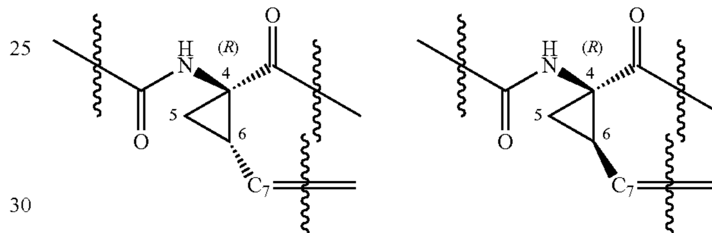
C7 syn to carbonyl
