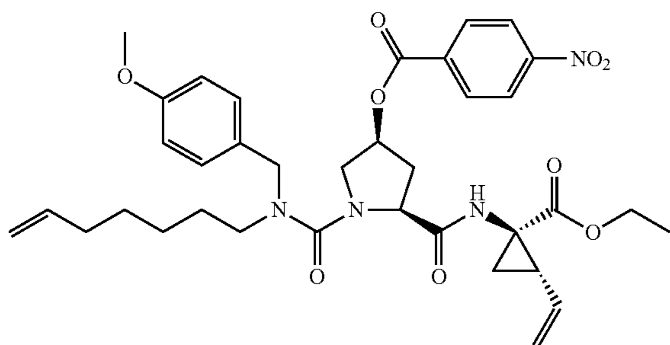
4-Nitro-benzoic acid 5-(1-ethoxycarbonyl-2-vinyl-cyclopropylcarbamoyl)-1-[hept-6-enyl-(4-methoxy-benzyl)-carbamoyl]-pyrrolidin-3-yl ester (135)
