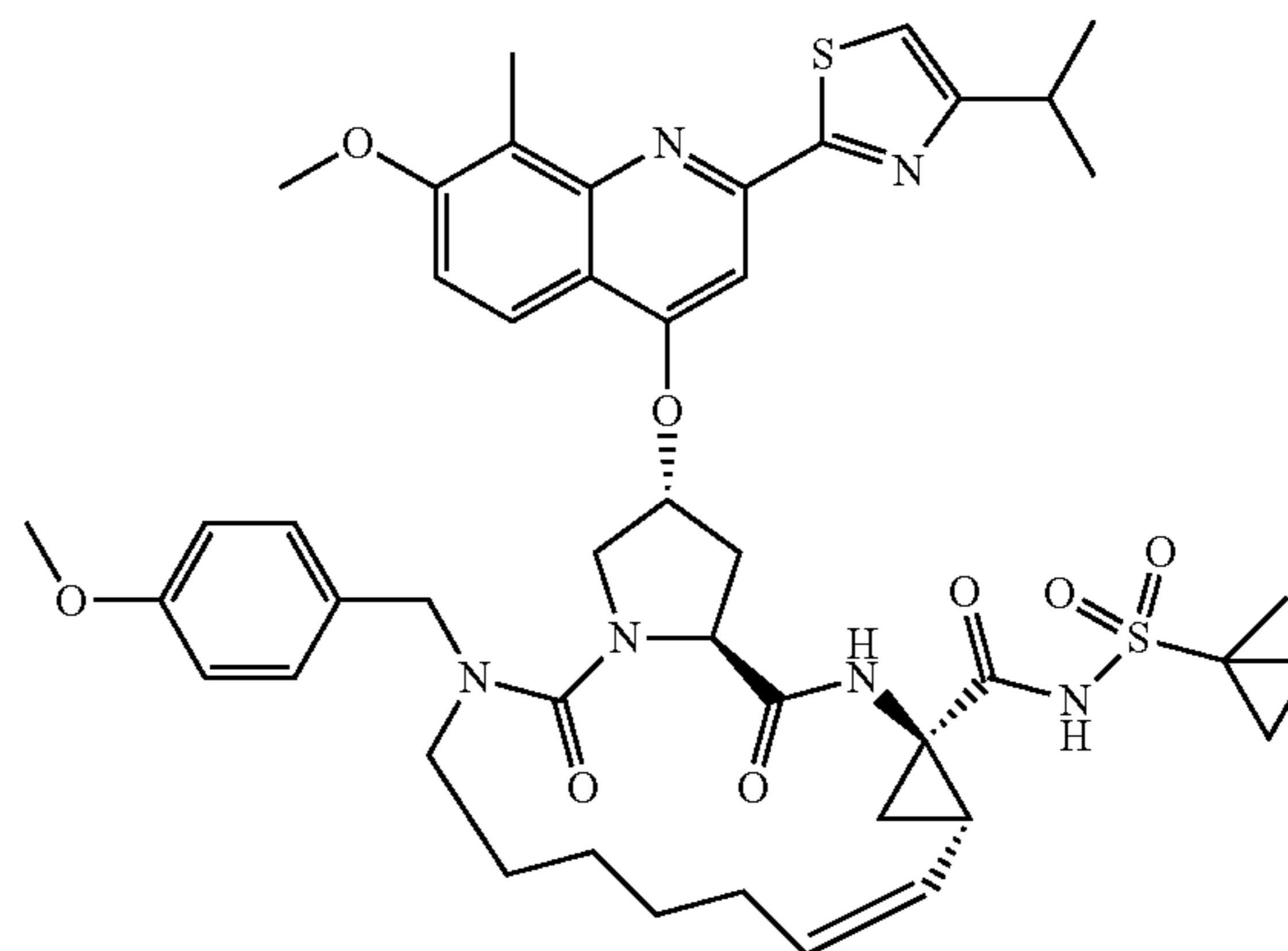
1-Methyl-cyclopropanesulfonic acid [18-[2-(4-isopropyl-thiazol-2-yl)-7-methoxy-8-methyl-quinolin-4-yloxy]-14-(4-methoxy-benzyl)-2,15-dioxo-3,14,16-triaza-tricyclo-[14.3.0.0*4,6*]nonadec-7-ene-4-carbonyl]-amide (139)
