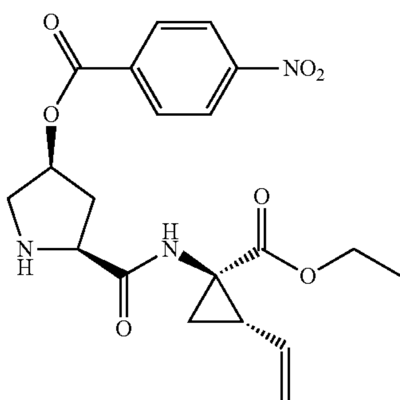
4-Nitro-benzoic acid 5-(1-ethoxycarbonyl-2-vinyl-cyclopropylcarbamoyl)-pyrrolidin-3-yl ester (134)
