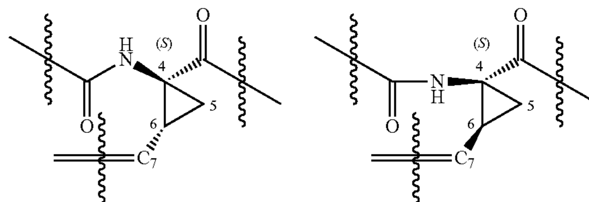
C7 syn to carbonyl
