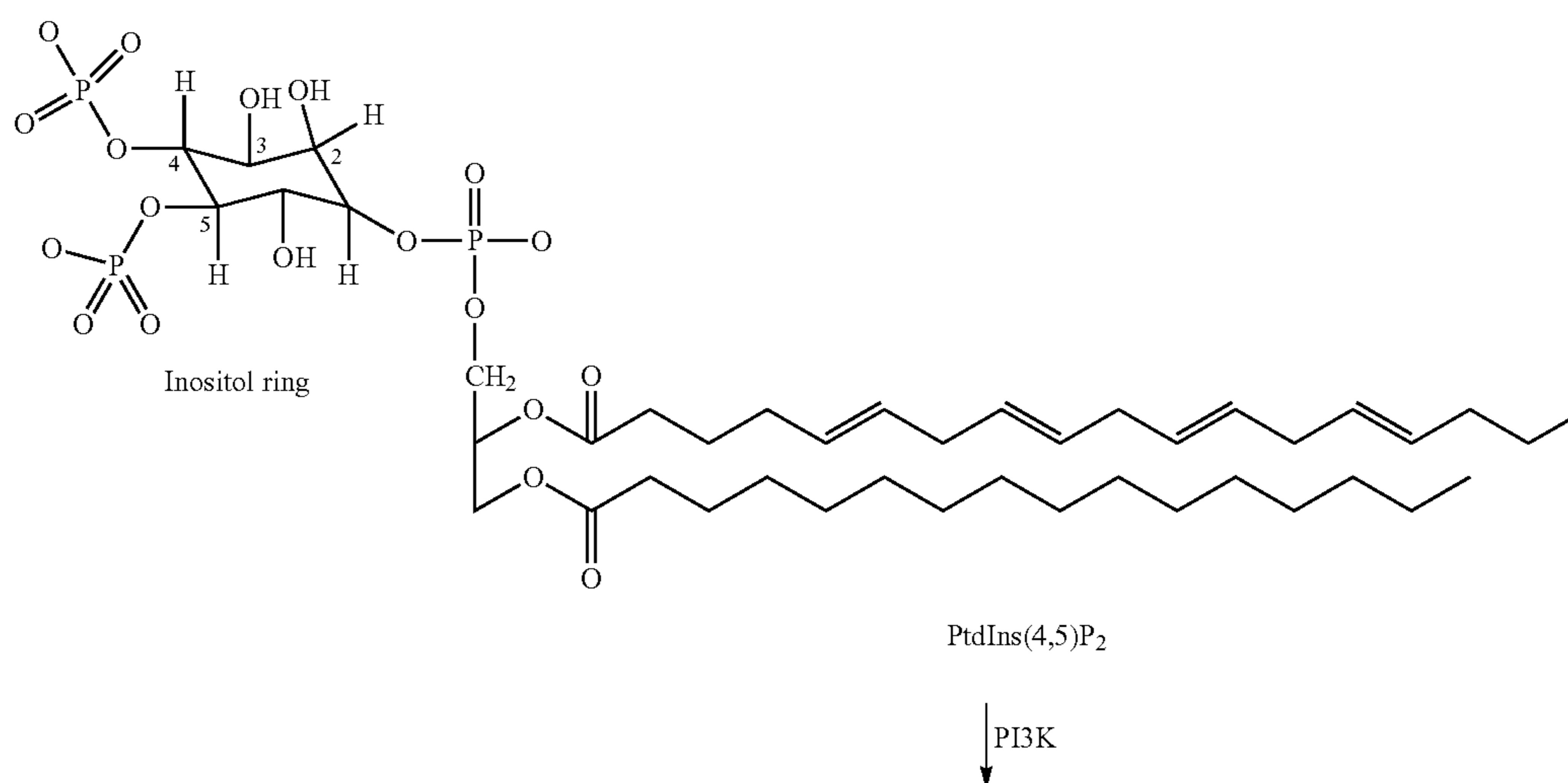
Scheme A: Conversion of PI(4,5)P 2 to PI(3,4,5)P 3
