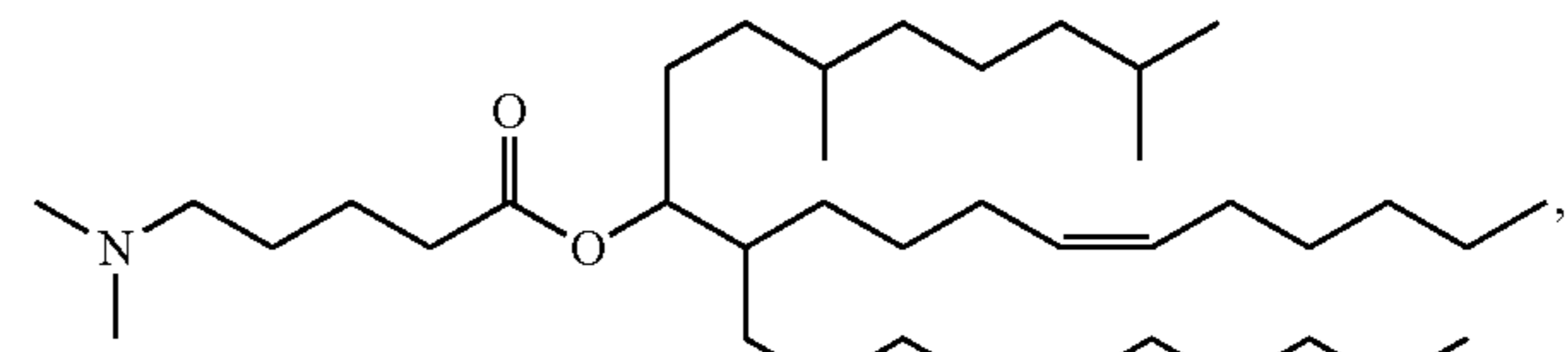
Compound 76
