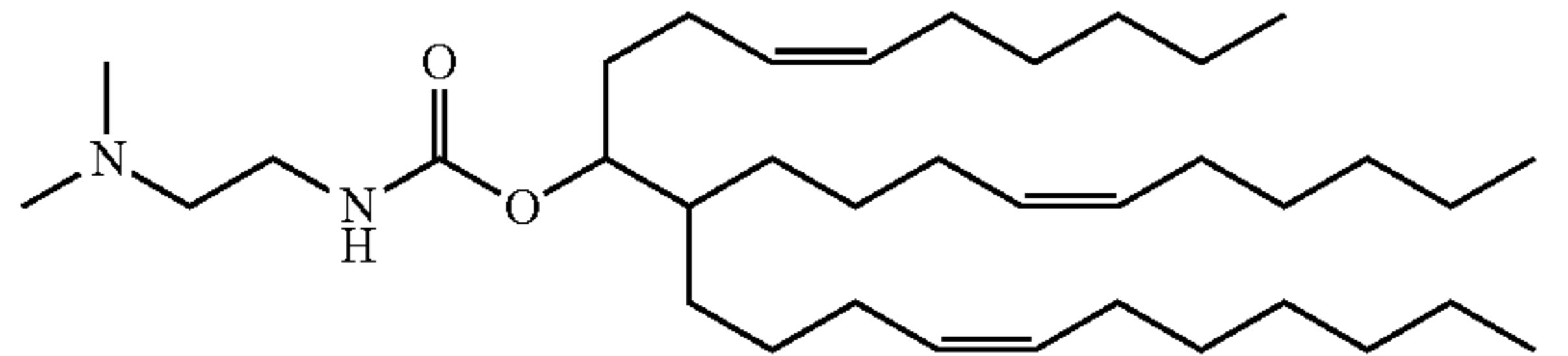
Compound 27
