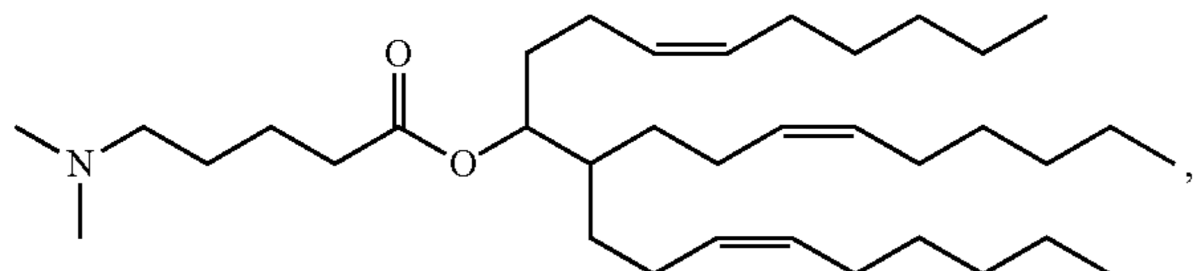
Compound 42
