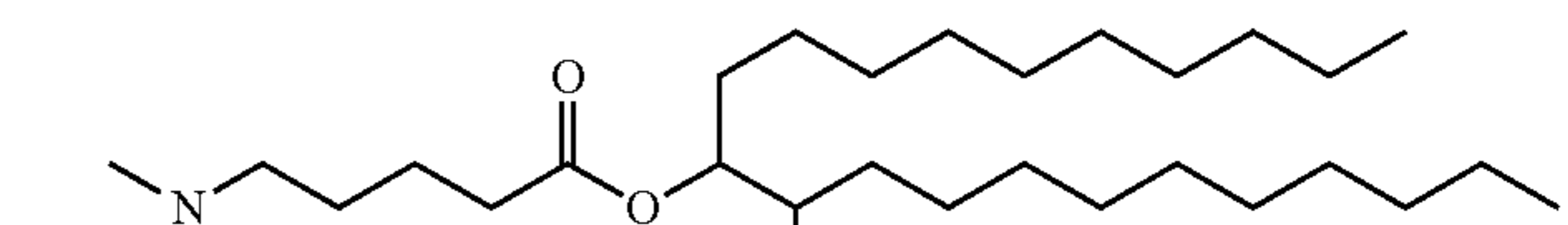
Compound 14
