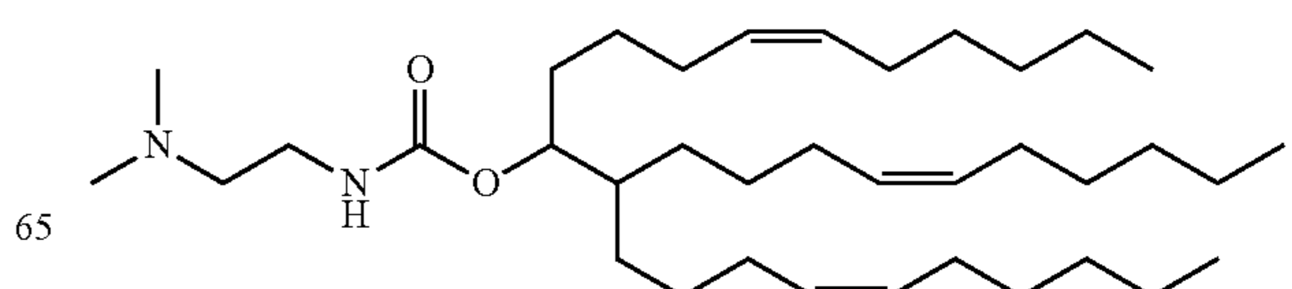
Compound 25
