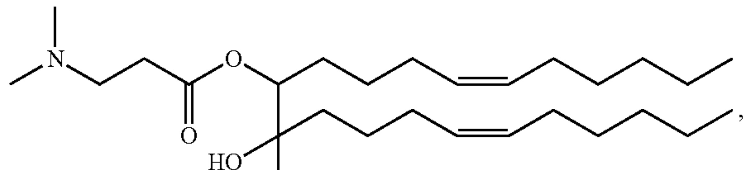
Compound 31
