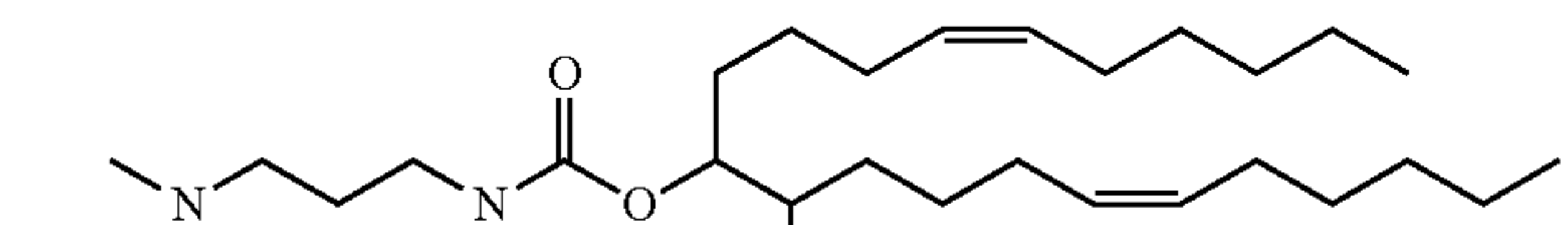
Compound 23
