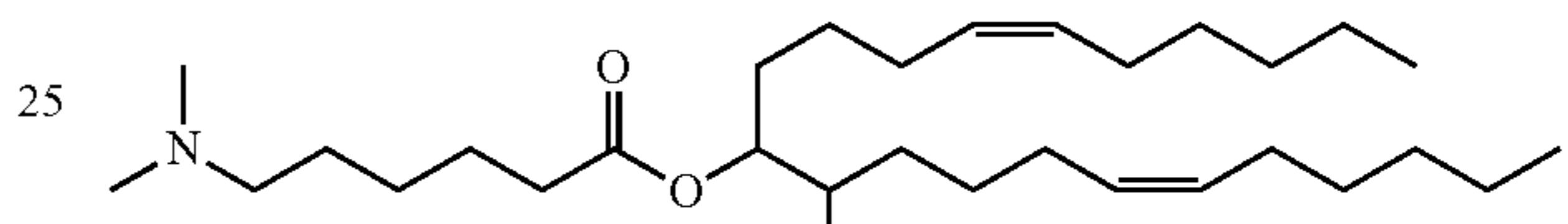
Compound 11
