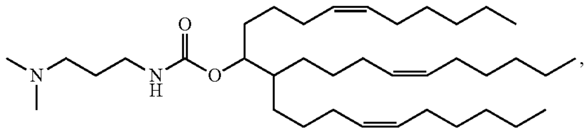
Compound 25
