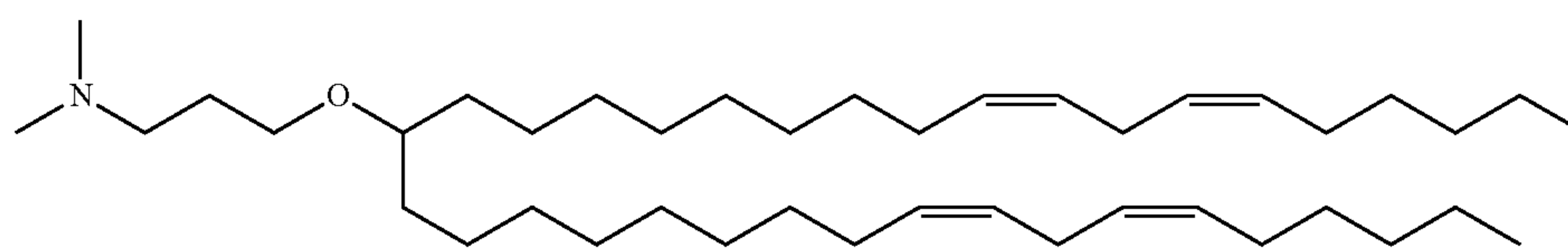
DLin-MP-DMA
