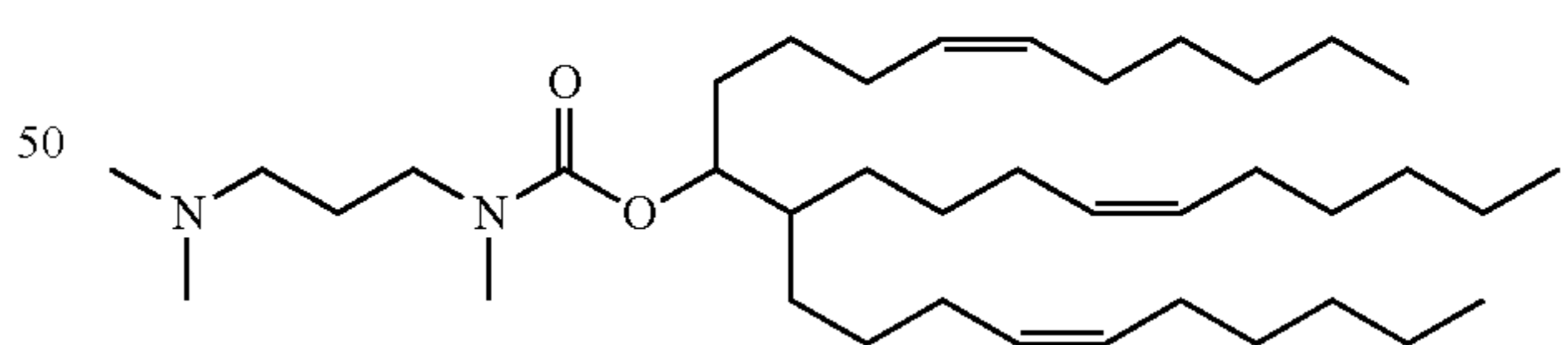
Compound 24
