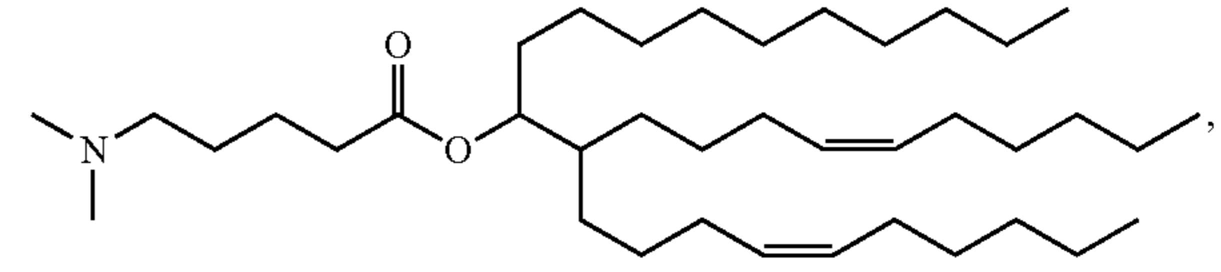
Compound 62
