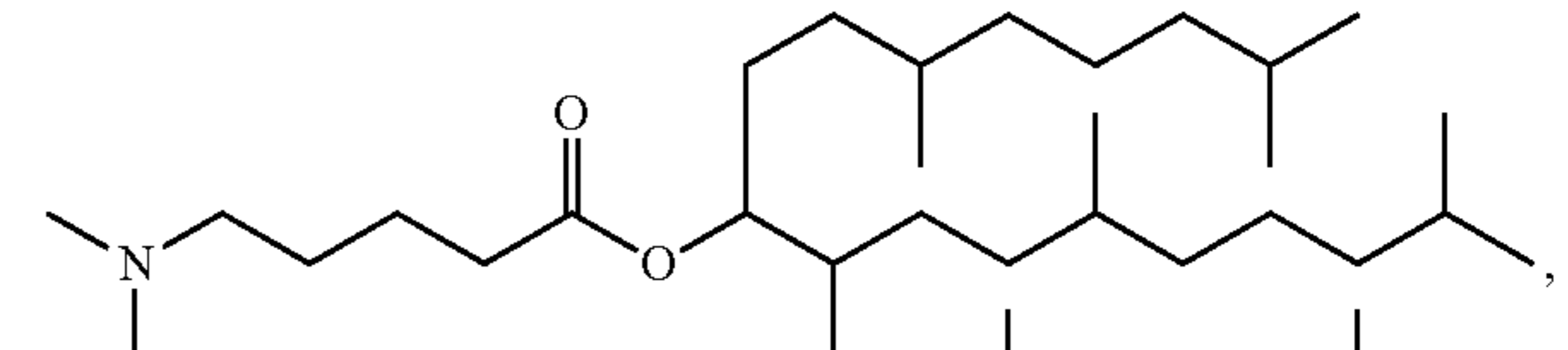
Compound 71
