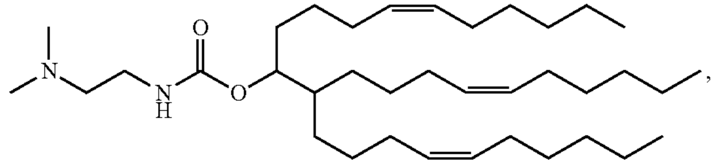
Compound 26
