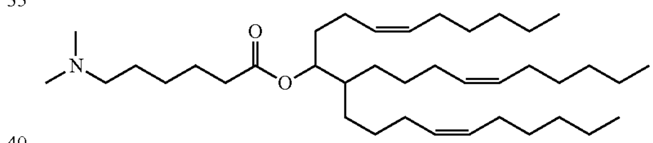
Compound 22
