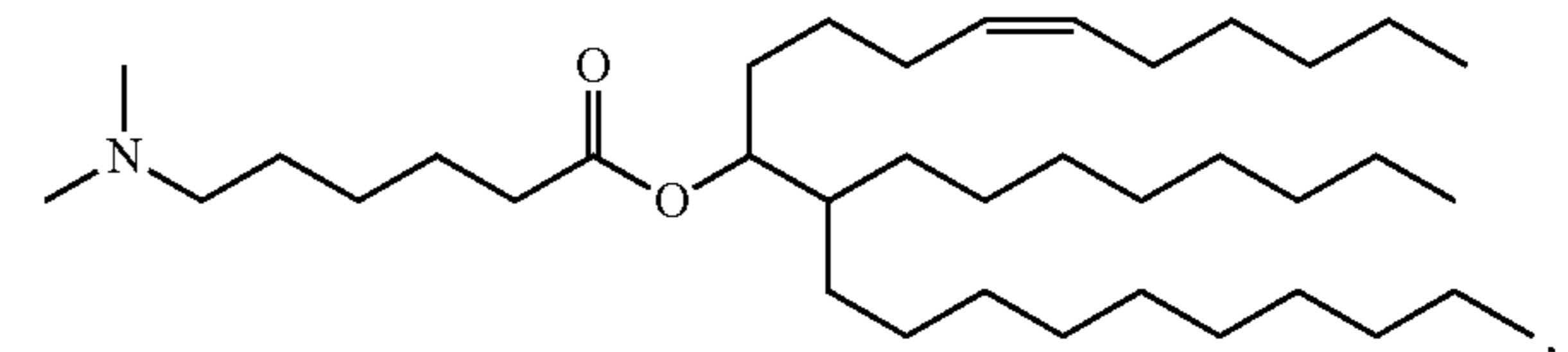
Compound 89
