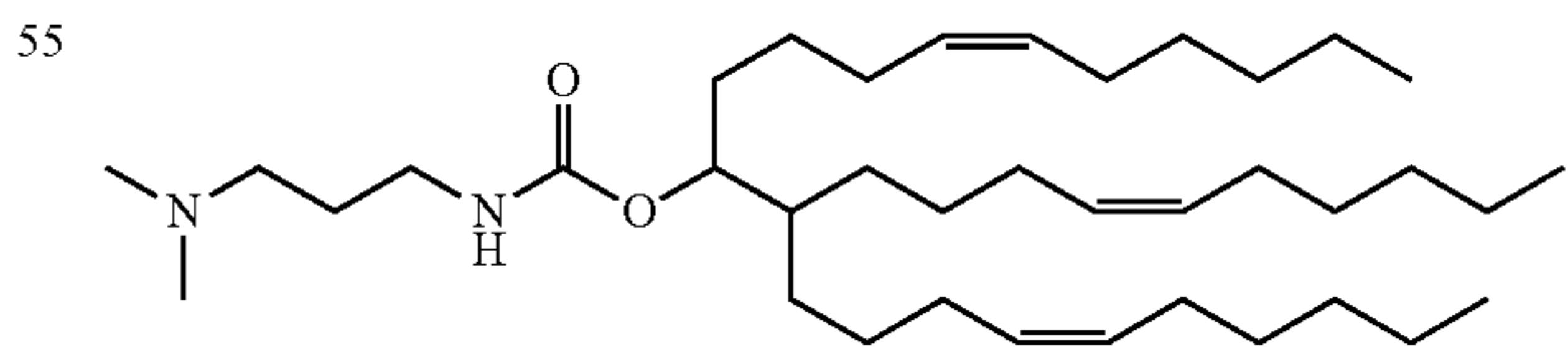
Compound 25
