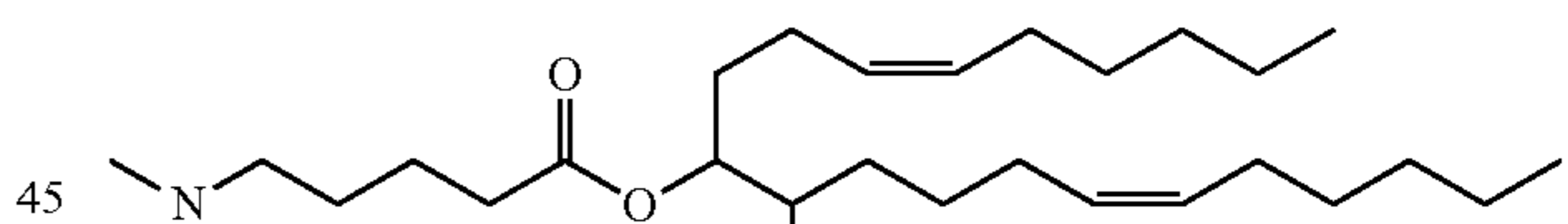
Compound 19
