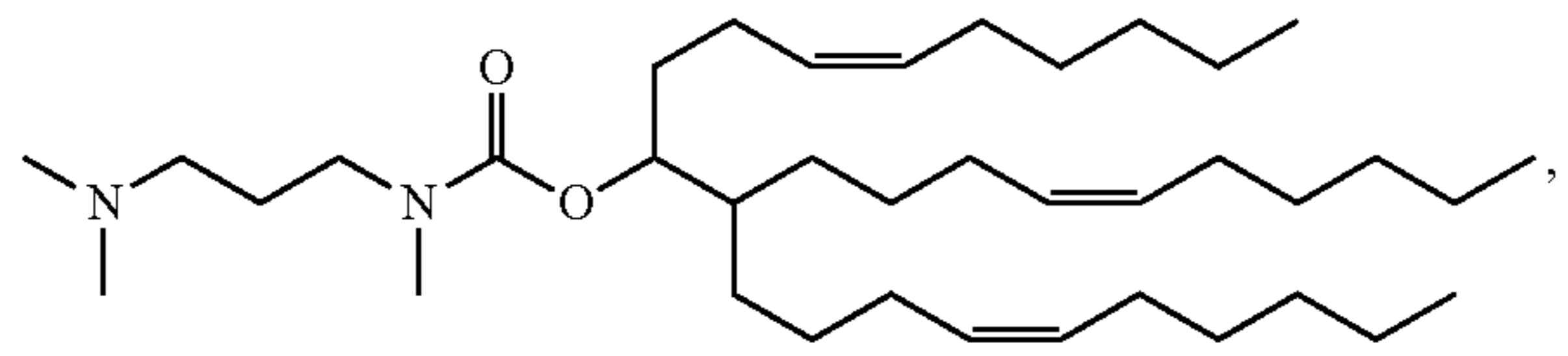
Compound 30
