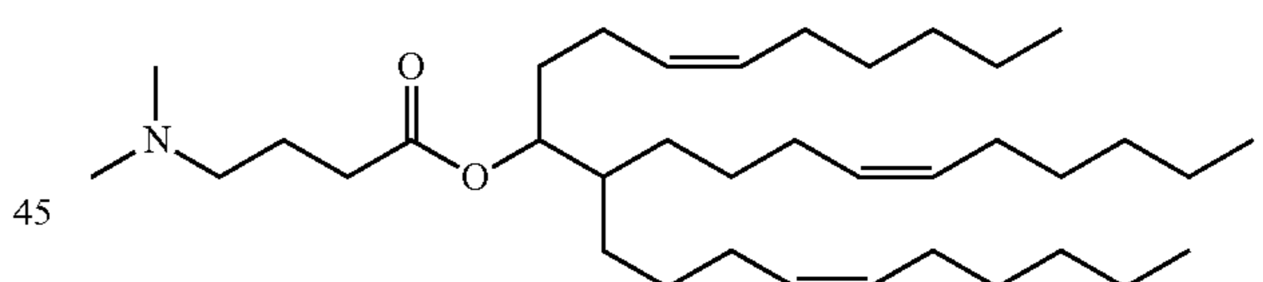
Compound 23
