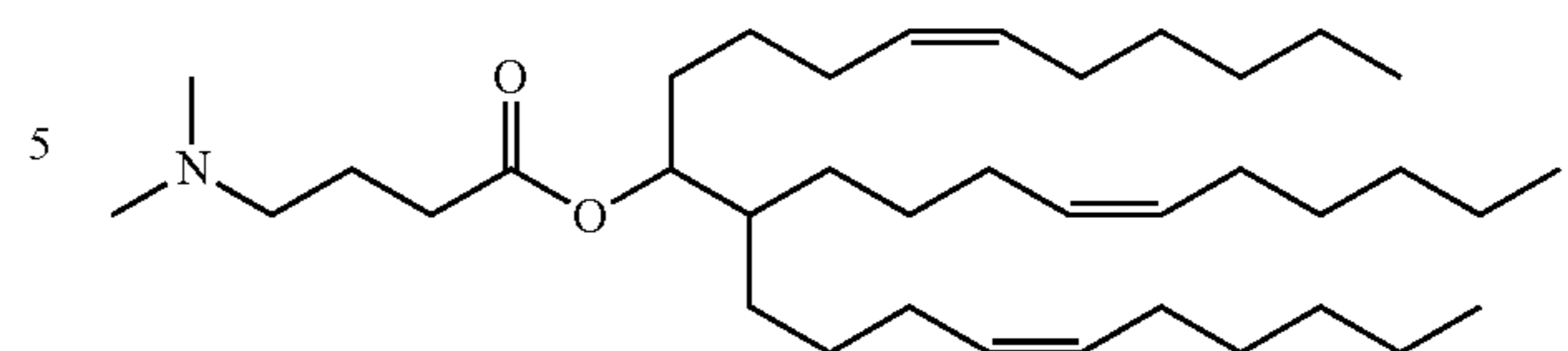
Compound 11
