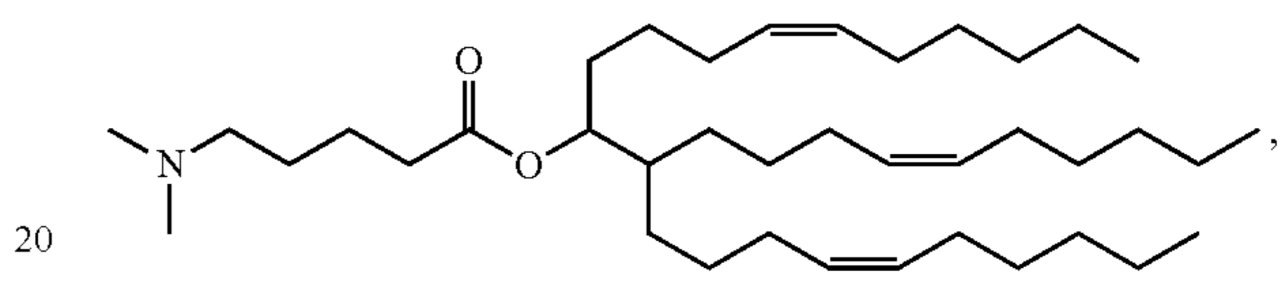
Compound 14
