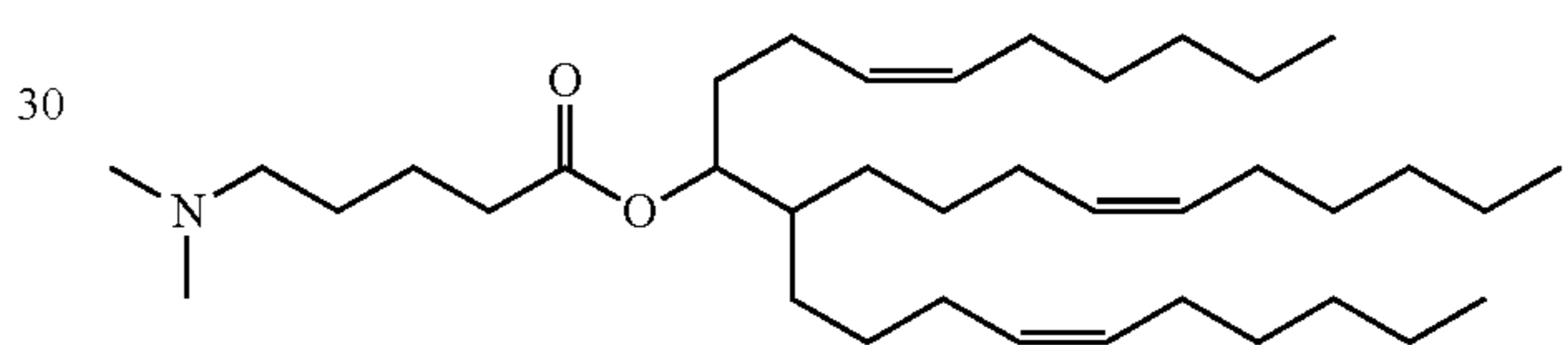
Compound 21
