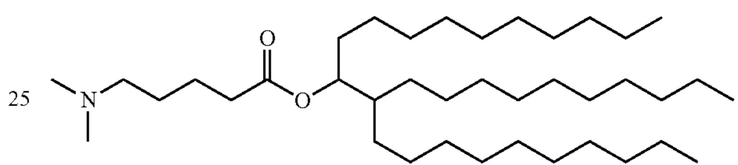
Compound 19
