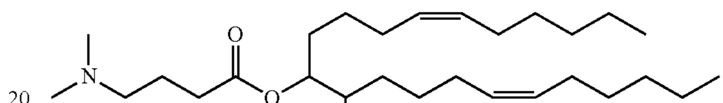
Compound 9
