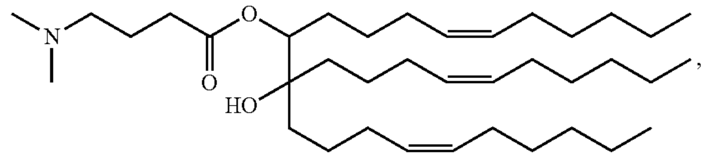
Compound 31
