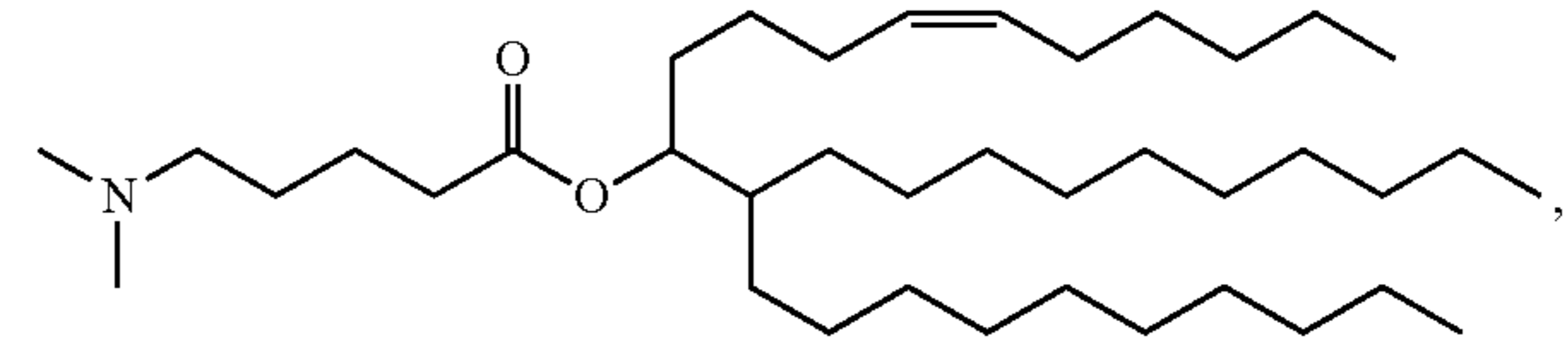
Compound 53
