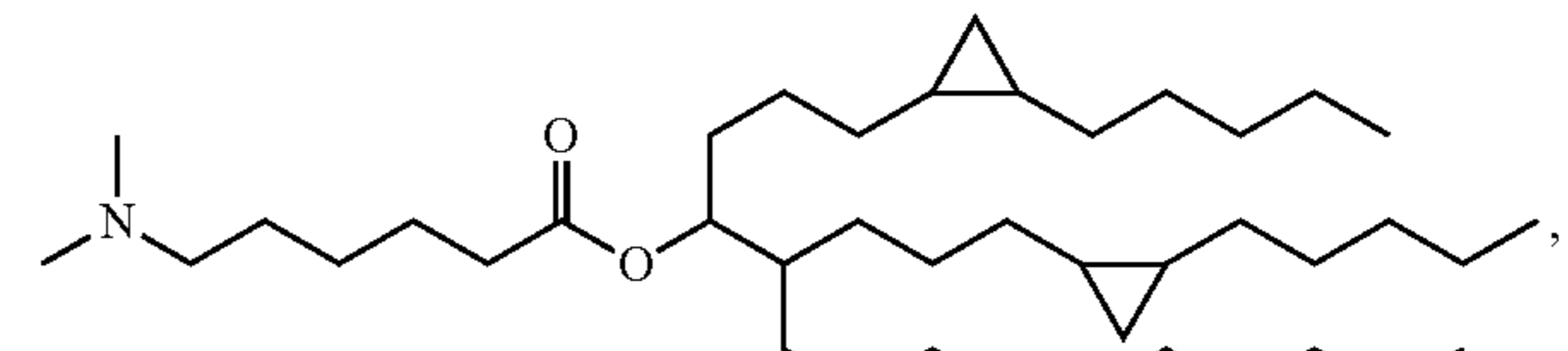
Compound 79
