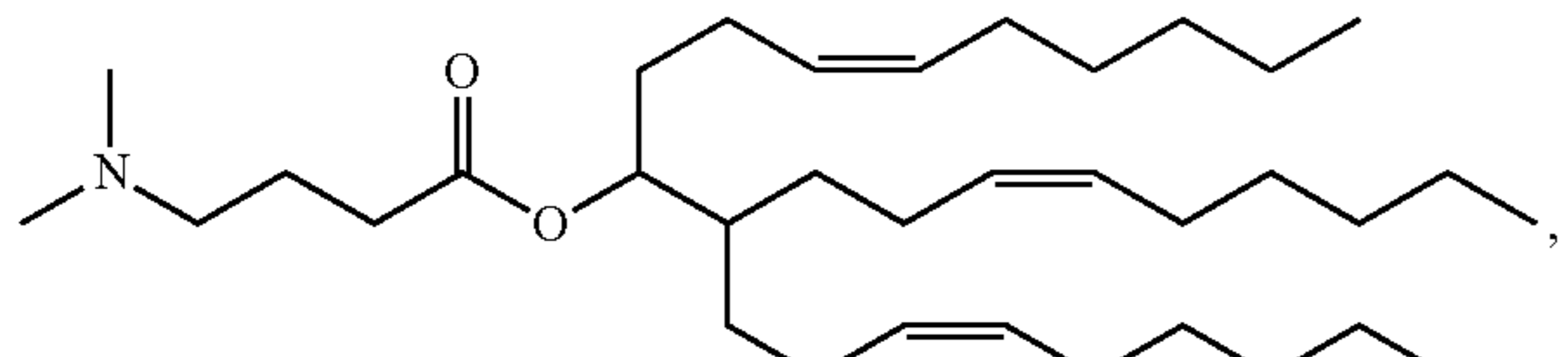
Compound 42
