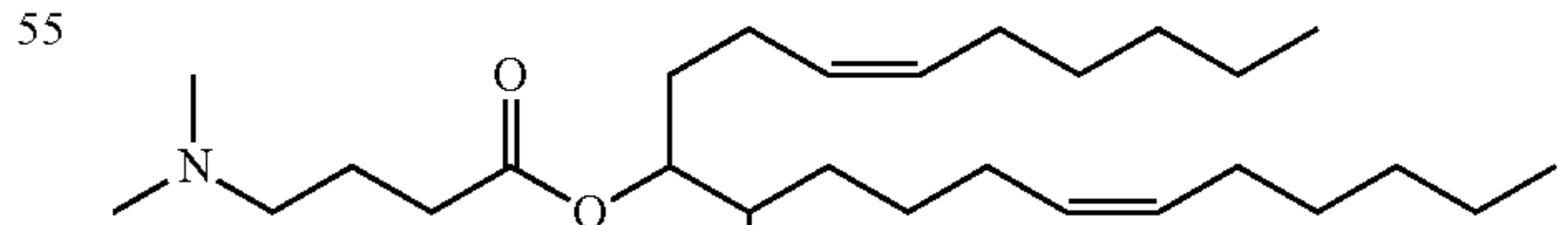
Compound 22
