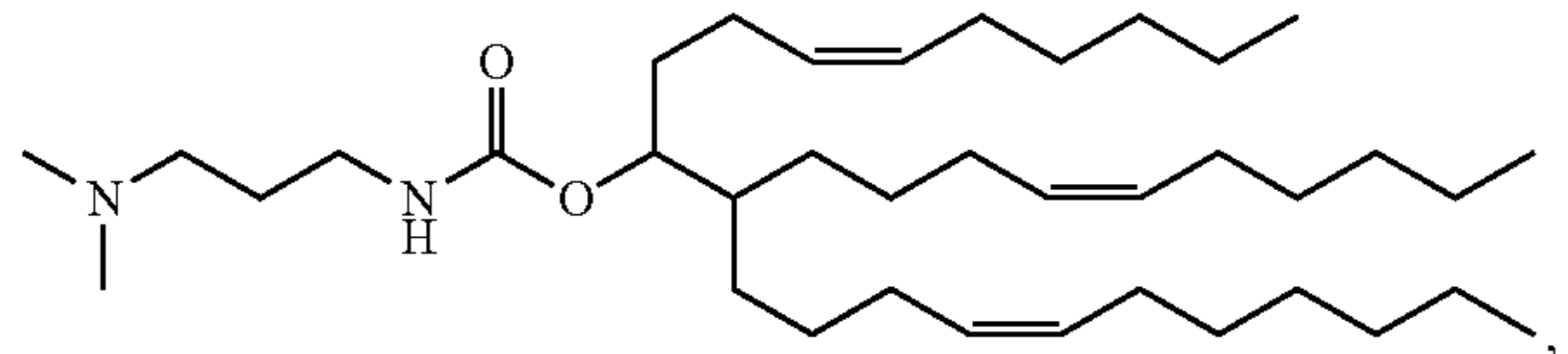
Compound 28
