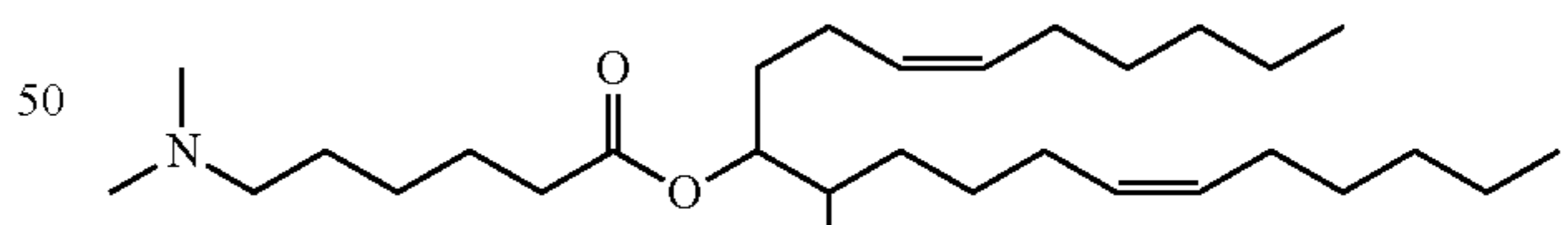
Compound 21
