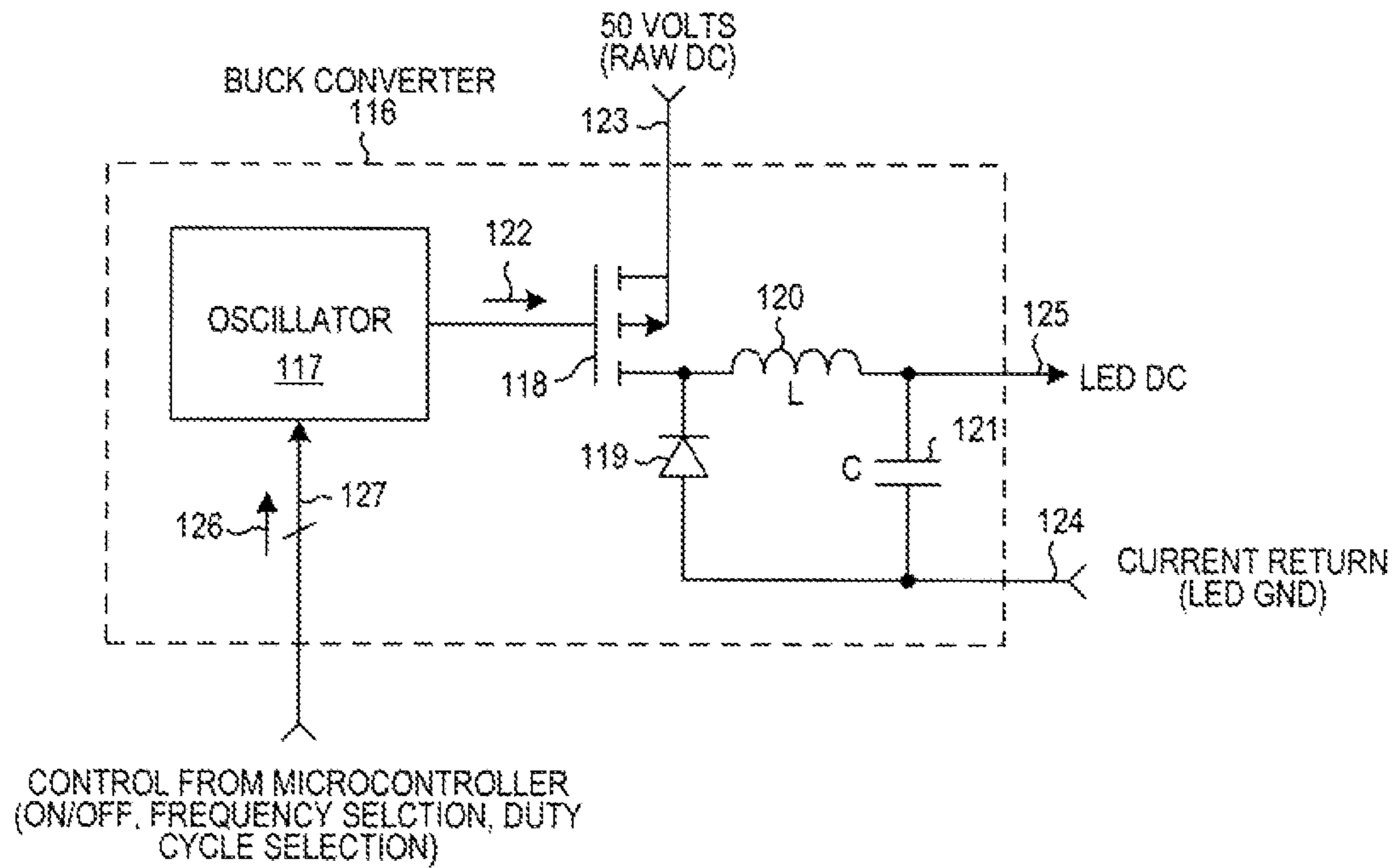
BUCK CONVERTER
