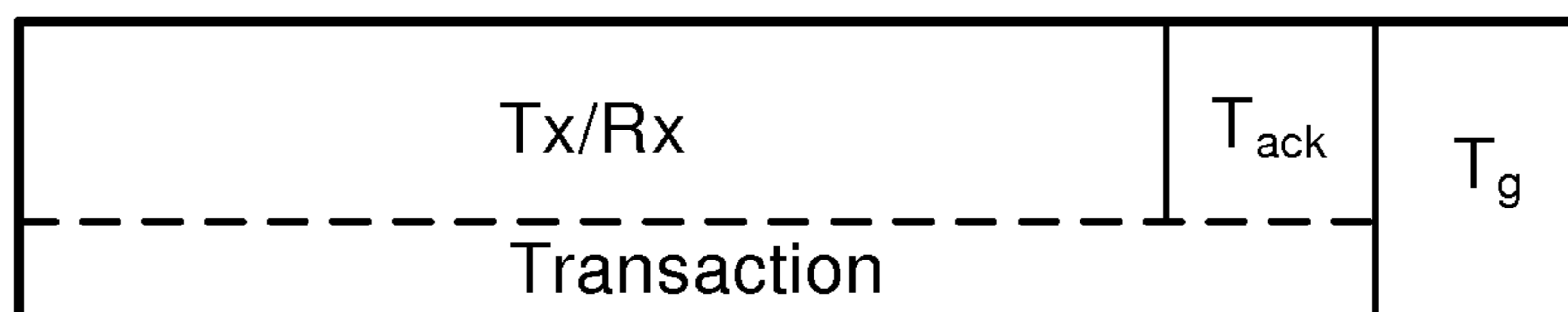
FIG. 1 Application Timeslot Format, single transaction
