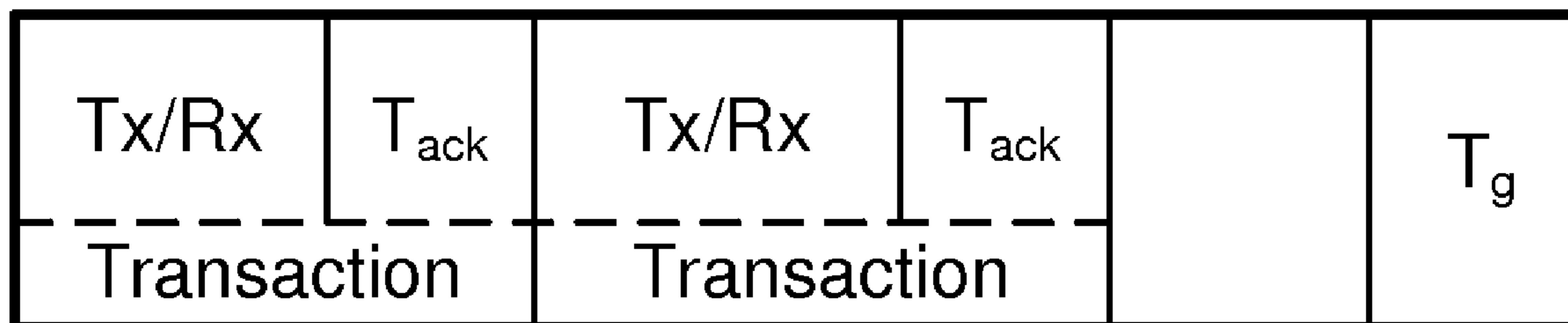
Application Timeslot Format, multiple transactions
