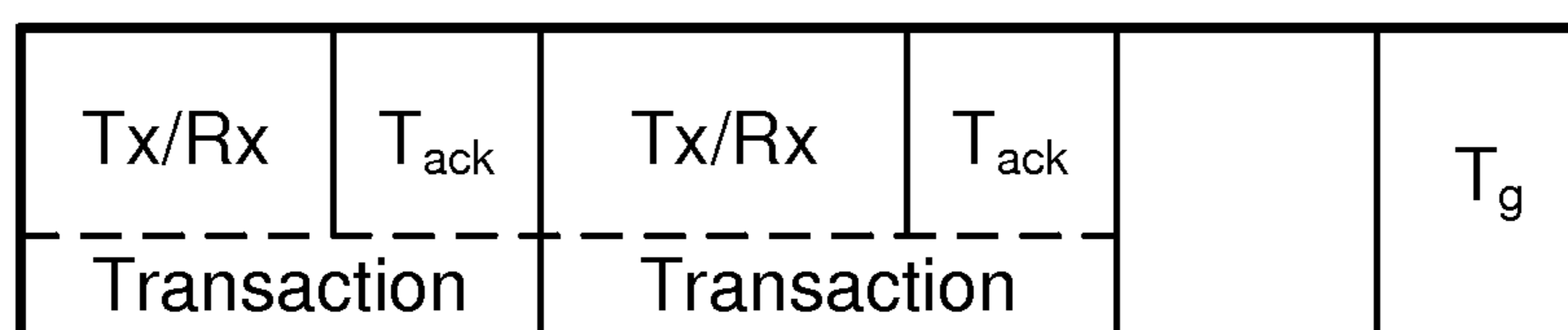
FIG. 2 Application Timeslot Format, multiple transactions
