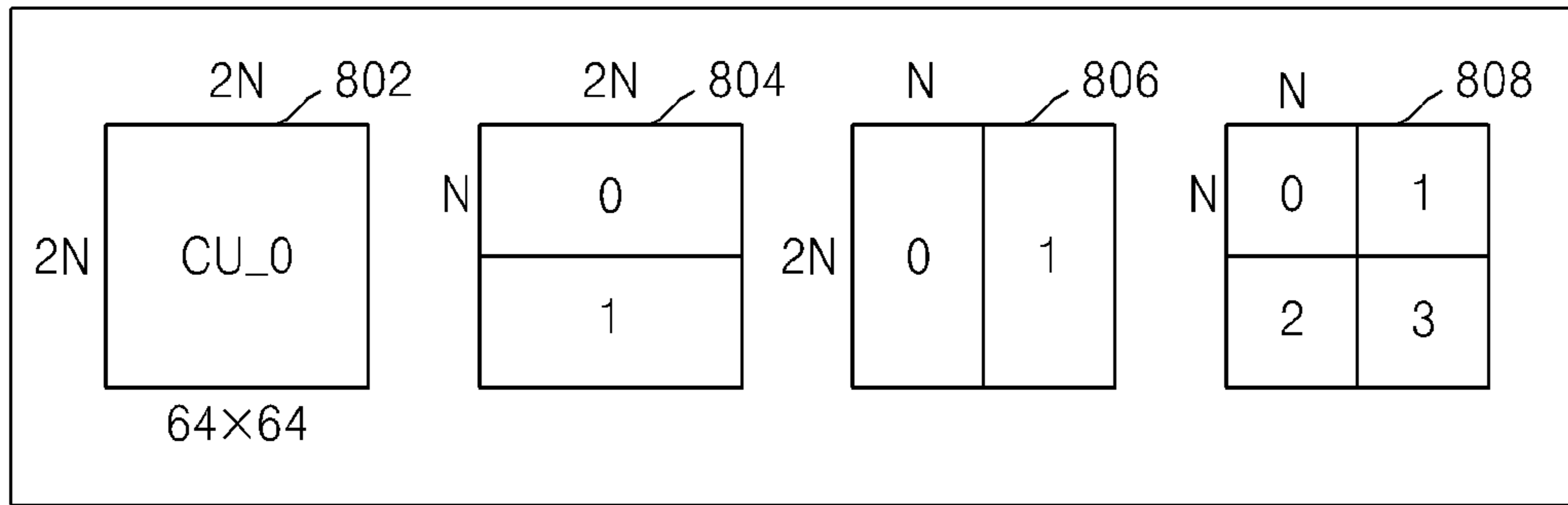
'PARTITION TYPE'-INFORMATION (800)
