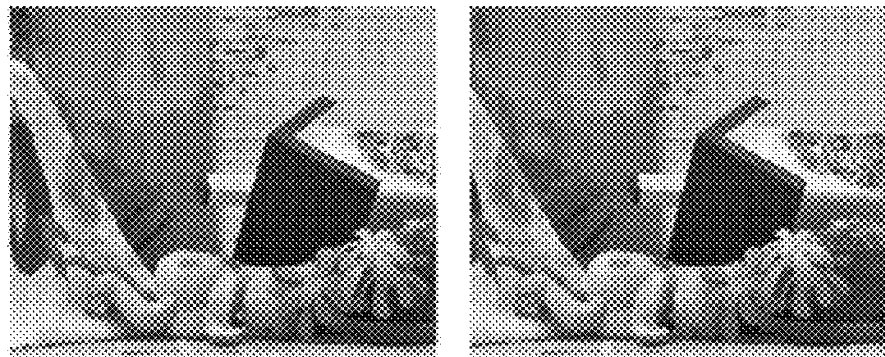
Stereo Completion
