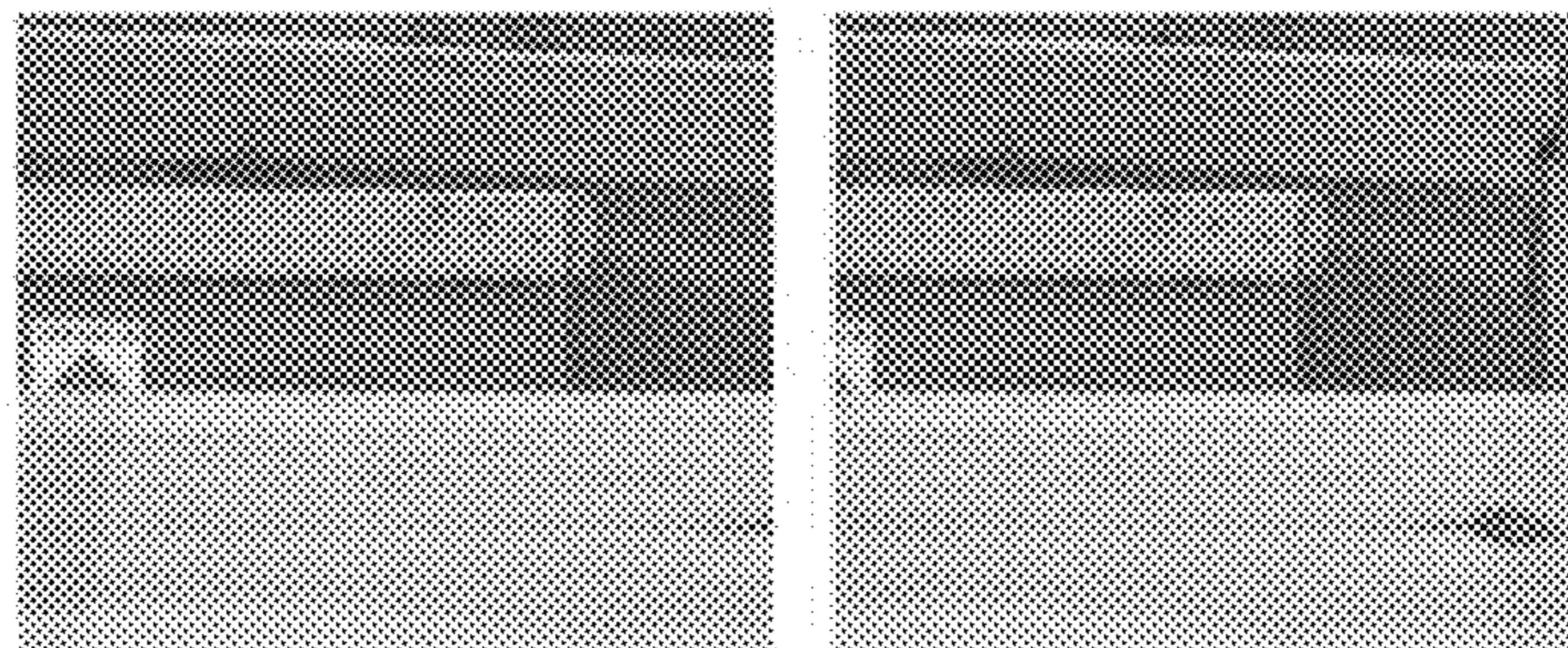
Stereo Completion
