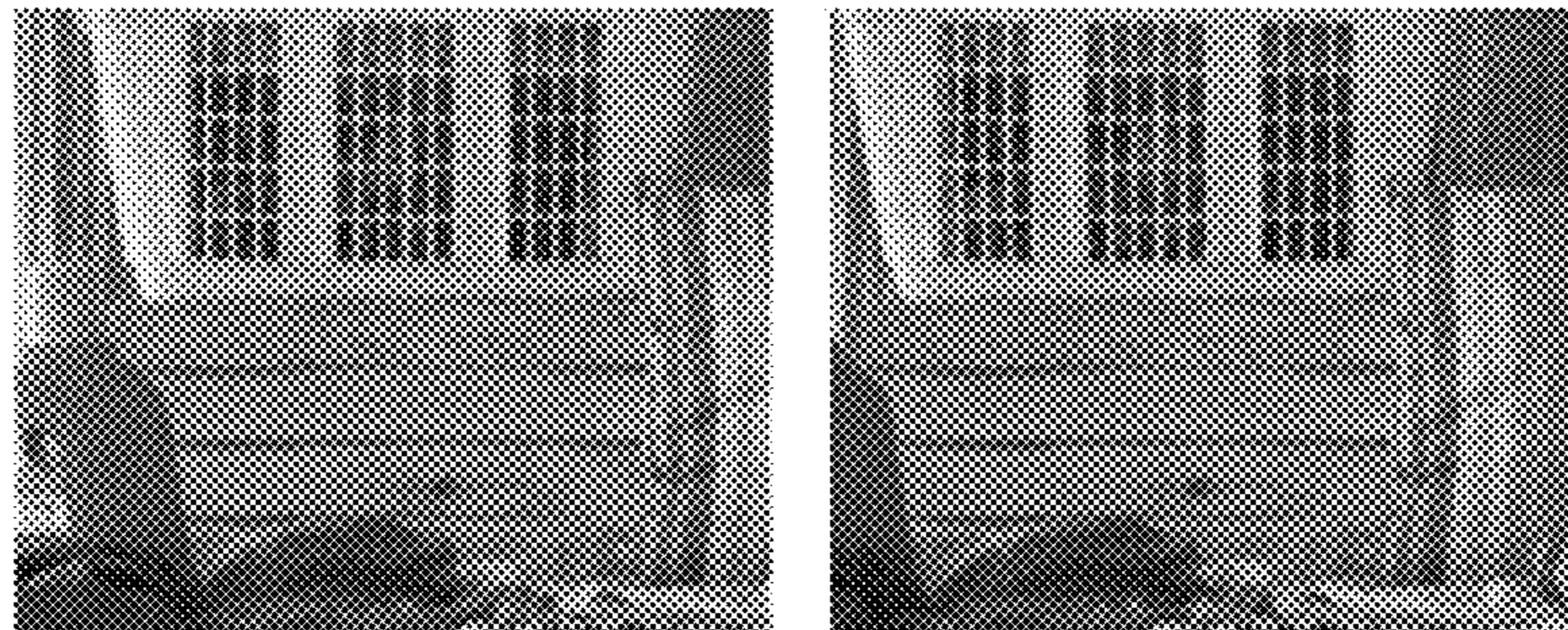
Stereo Completion
