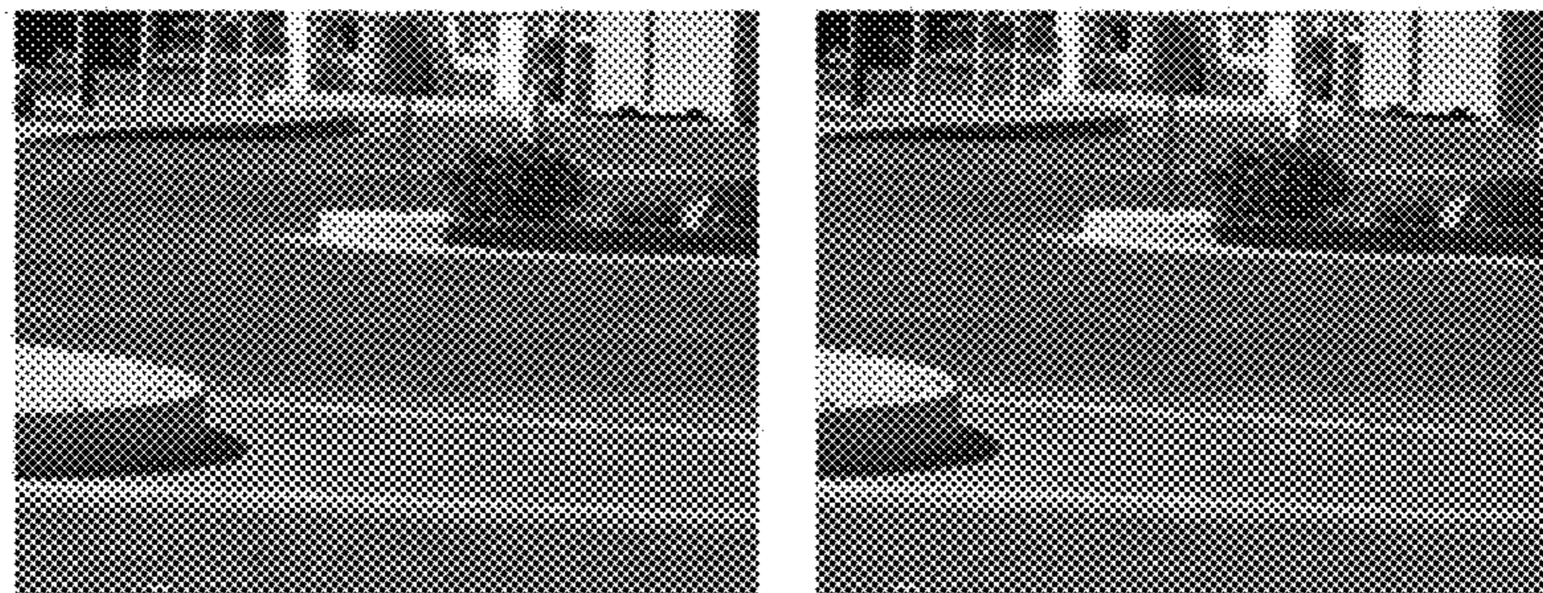
Stereo Completion
