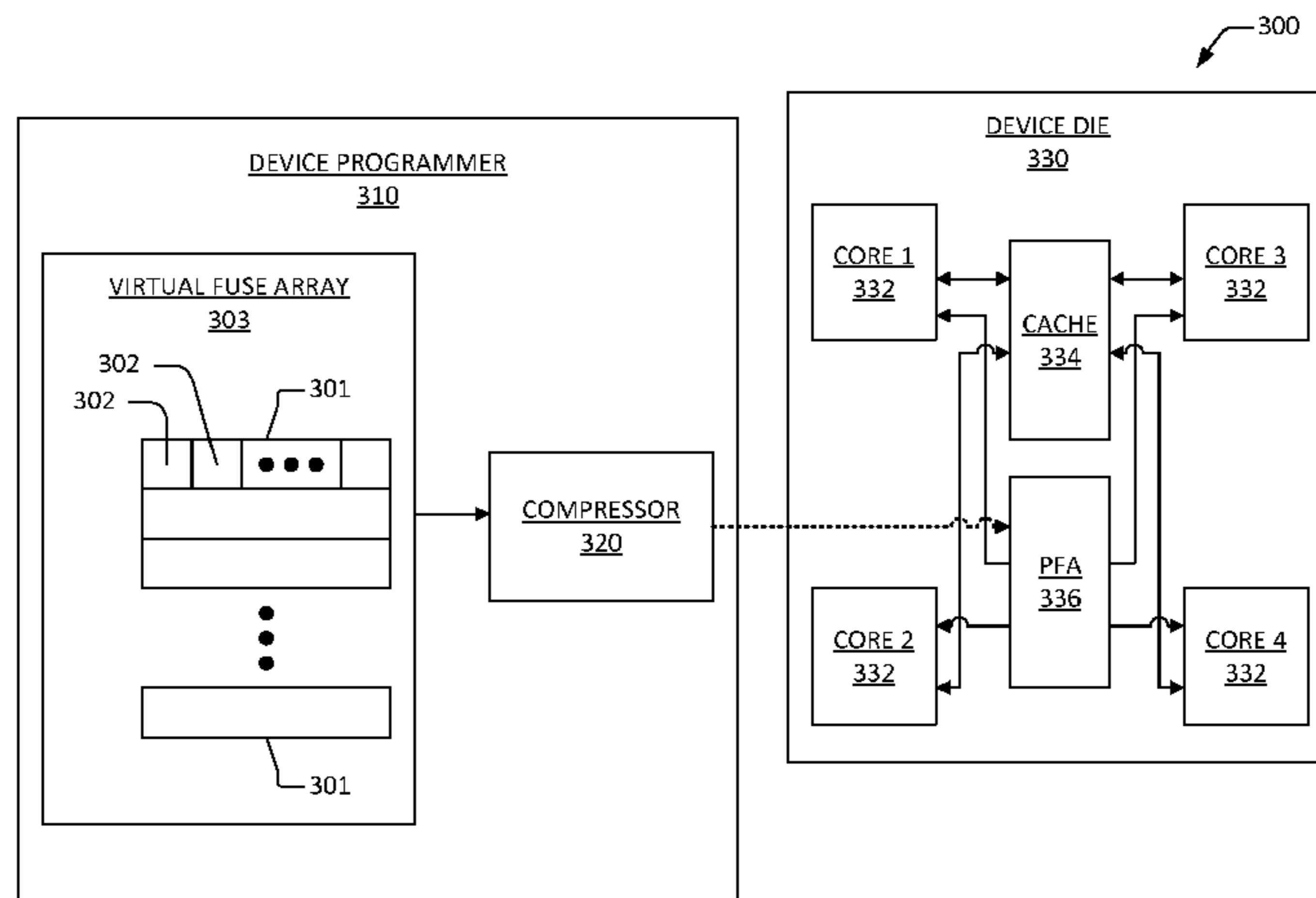
MICROPROCESSOR FUSE ARRAY COMPRESSION SYSTEM
