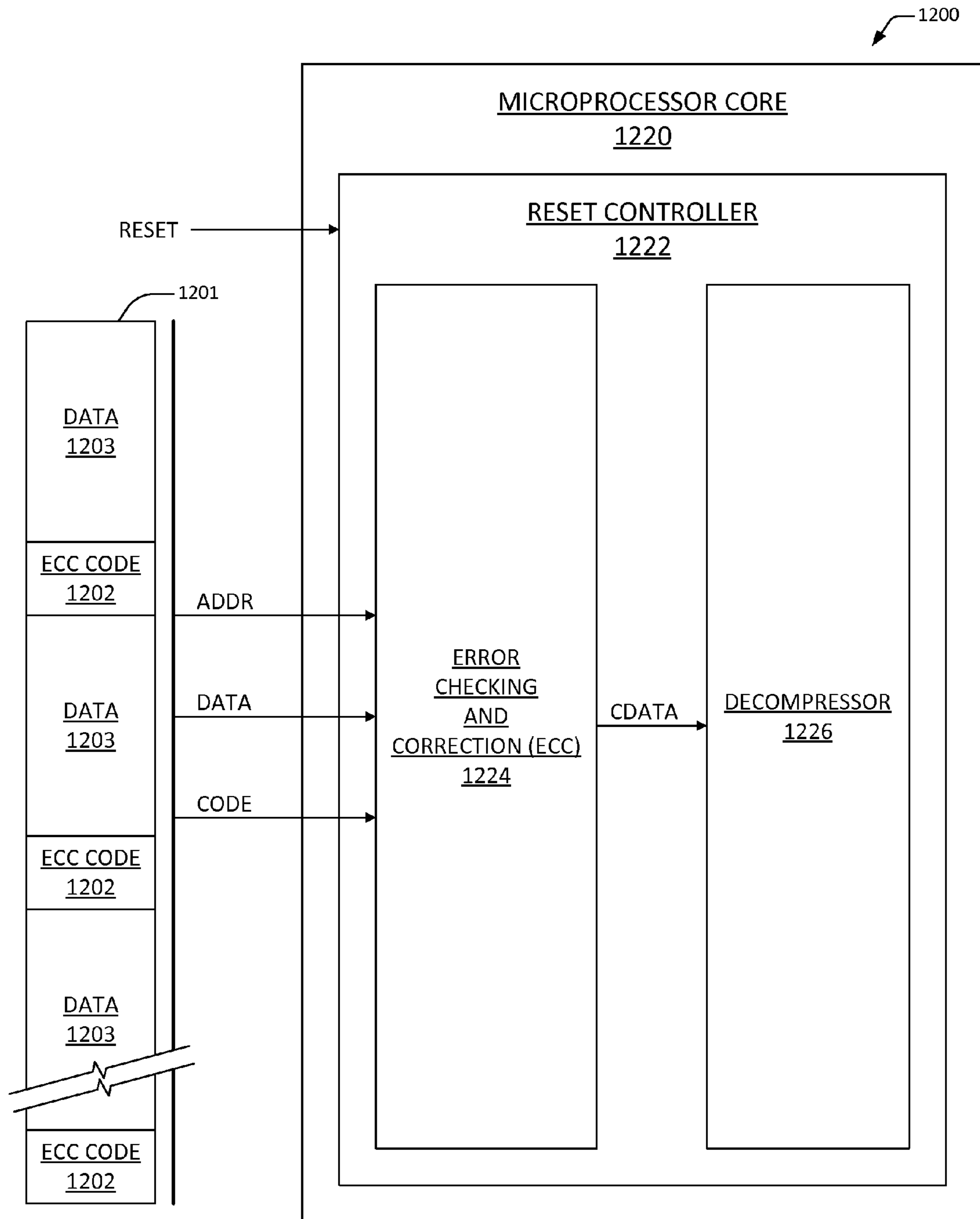
ERROR CHECKING AND CORRECTION (ECC) MECHNISM
