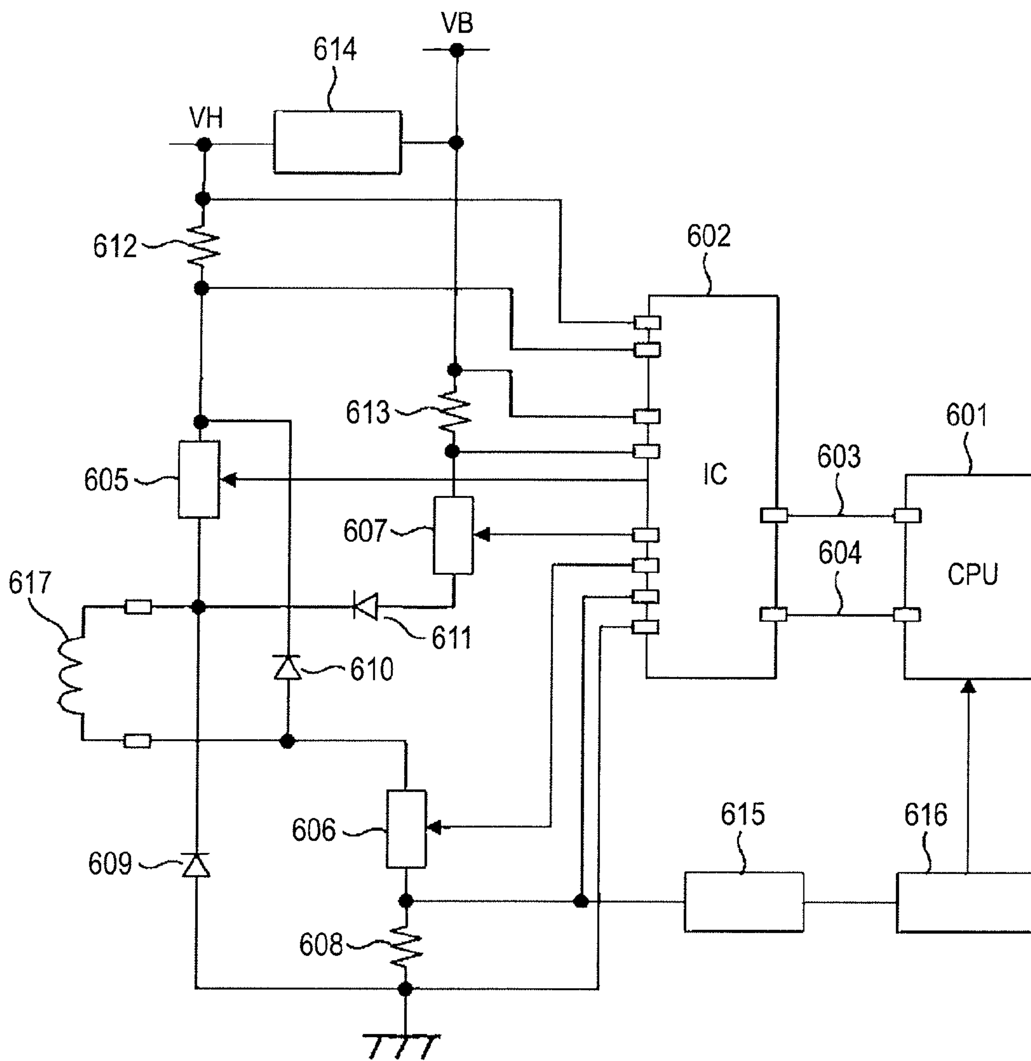
DRIVER CIRCUIT CONFIGURATION FOR DETECTING VALVE OPENING TIMING
