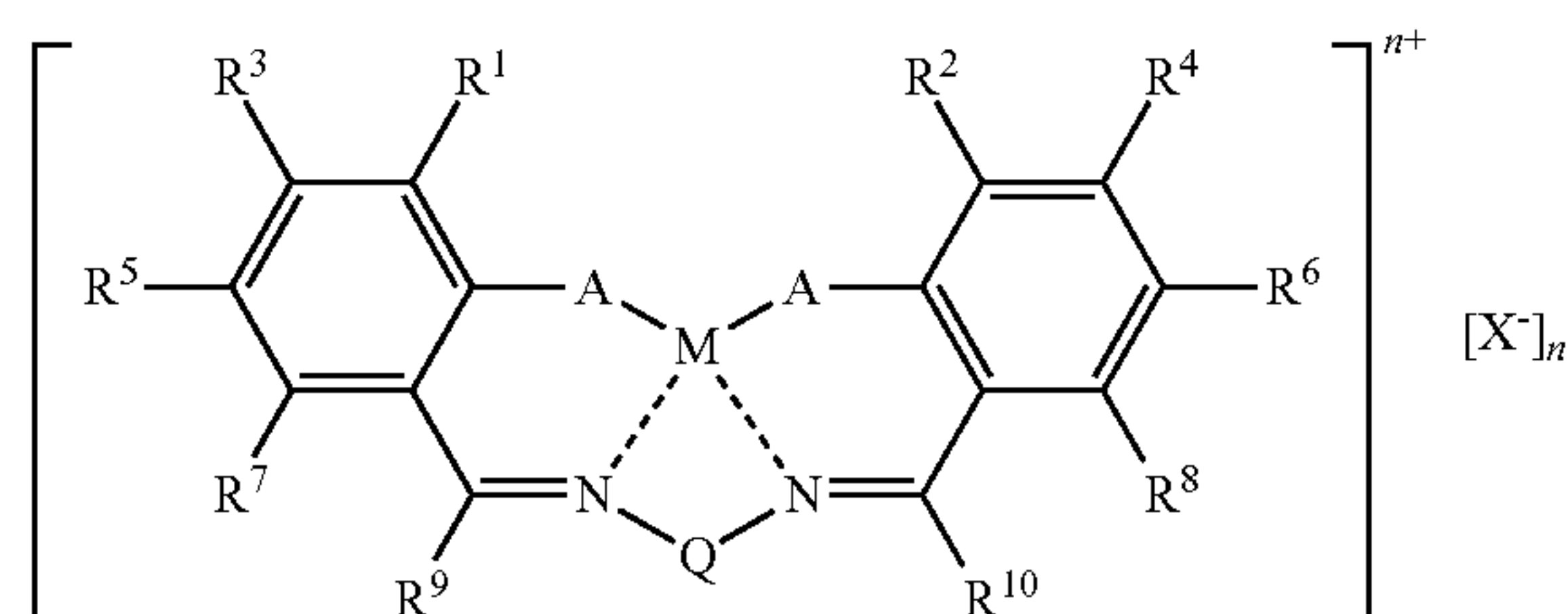
[Chemical Formula 2]
