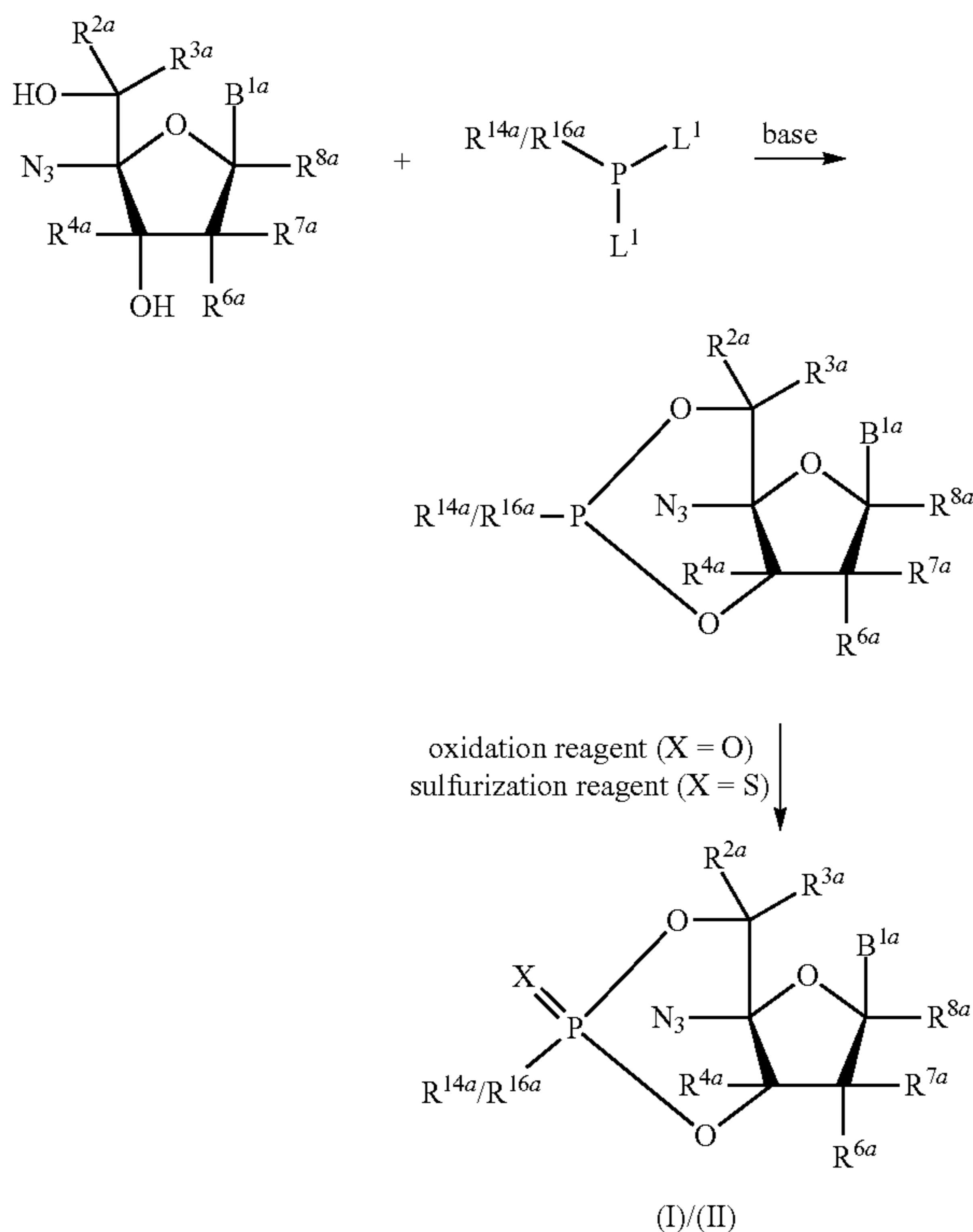
Scheme 4:
