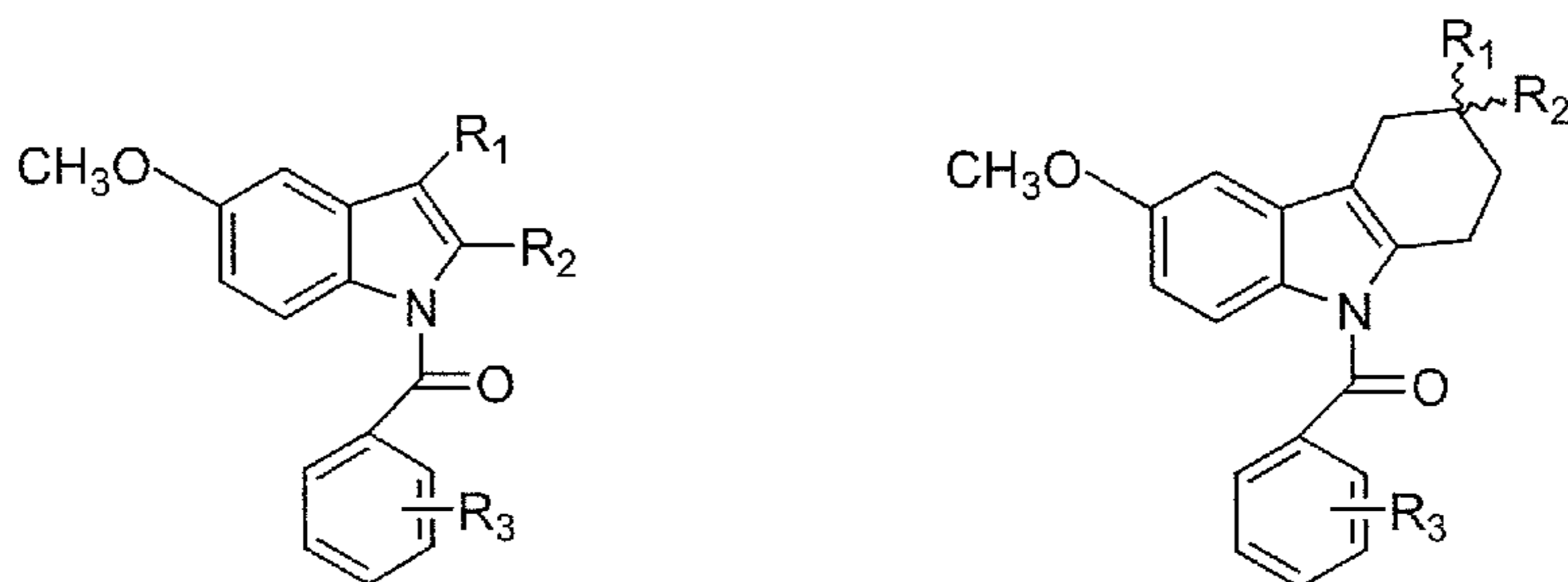
Compound 4, 5 Series
