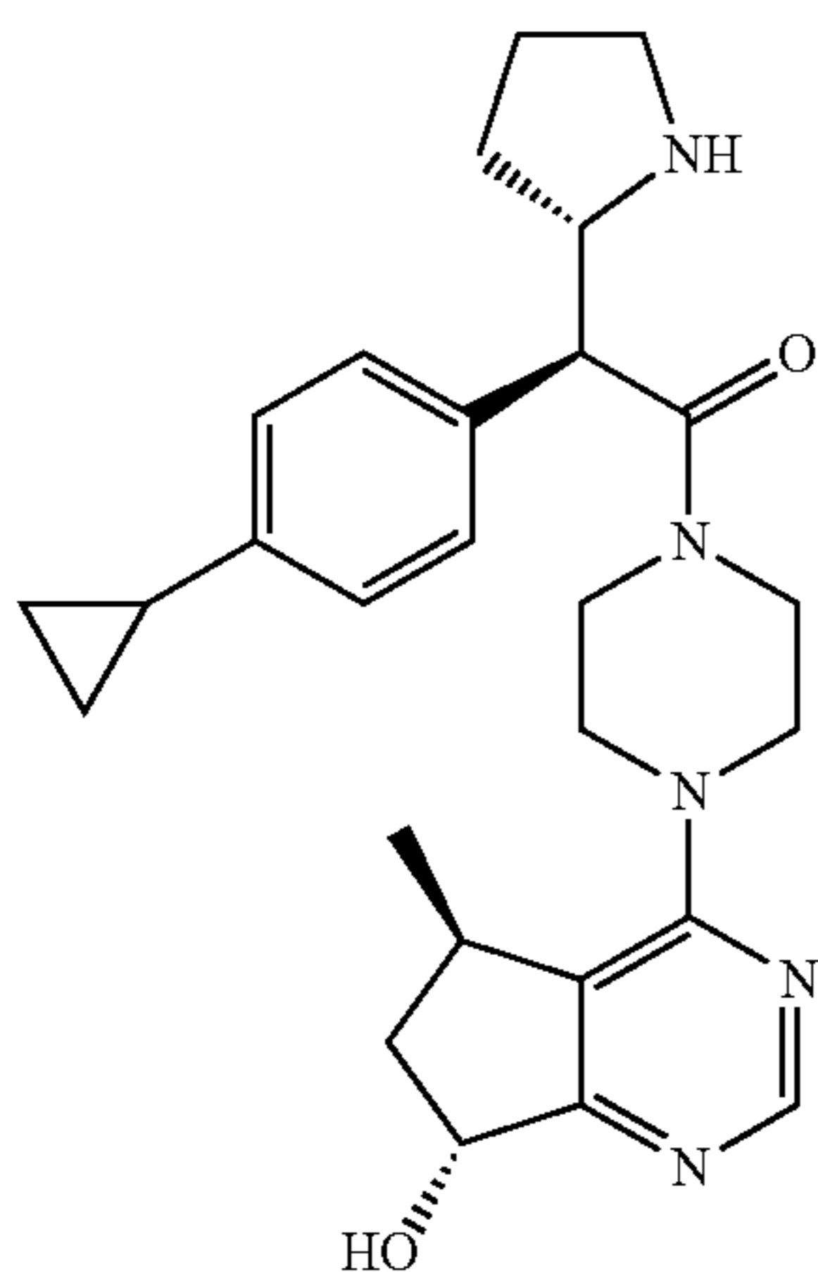
(S)-2-(4-cyclopropylphenyl)-1-(4-((5R,7R)-7-hydroxy-5-methyl-6,7-dihydro-5H-cyclopenta[d]pyrimidin-4-yl)piperazin-1-yl)-2-((S)-pyrrolidin-2-yl)ethanone
