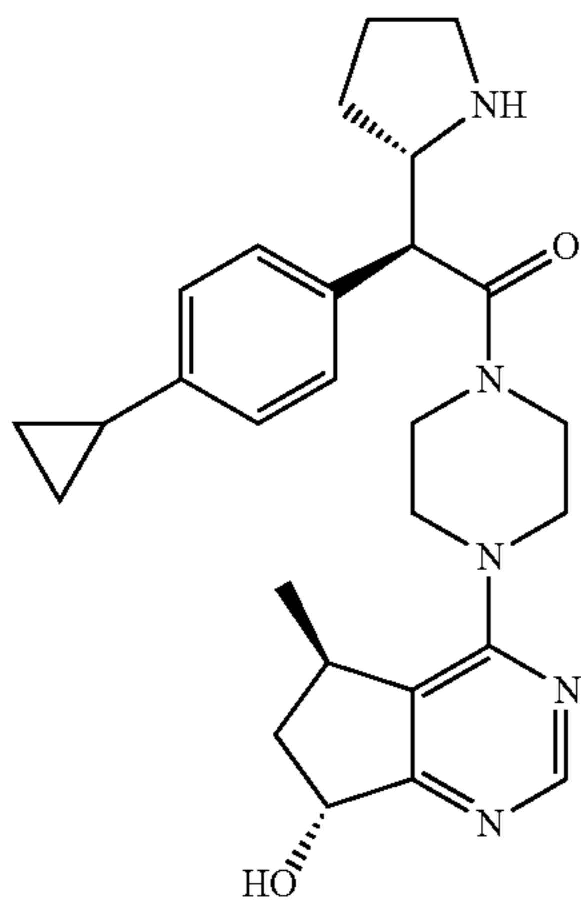
(S)-2-(4-cyclopropylphenyl)-1-(4-((5R,7R)-7-hydroxy-5-methyl-6,7-dihydro-5H-cyclopenta[d]pyrimidin-4-yl)piperazin-1-yl)-2-((S)-pyrrolidin-2-yl)ethanone
