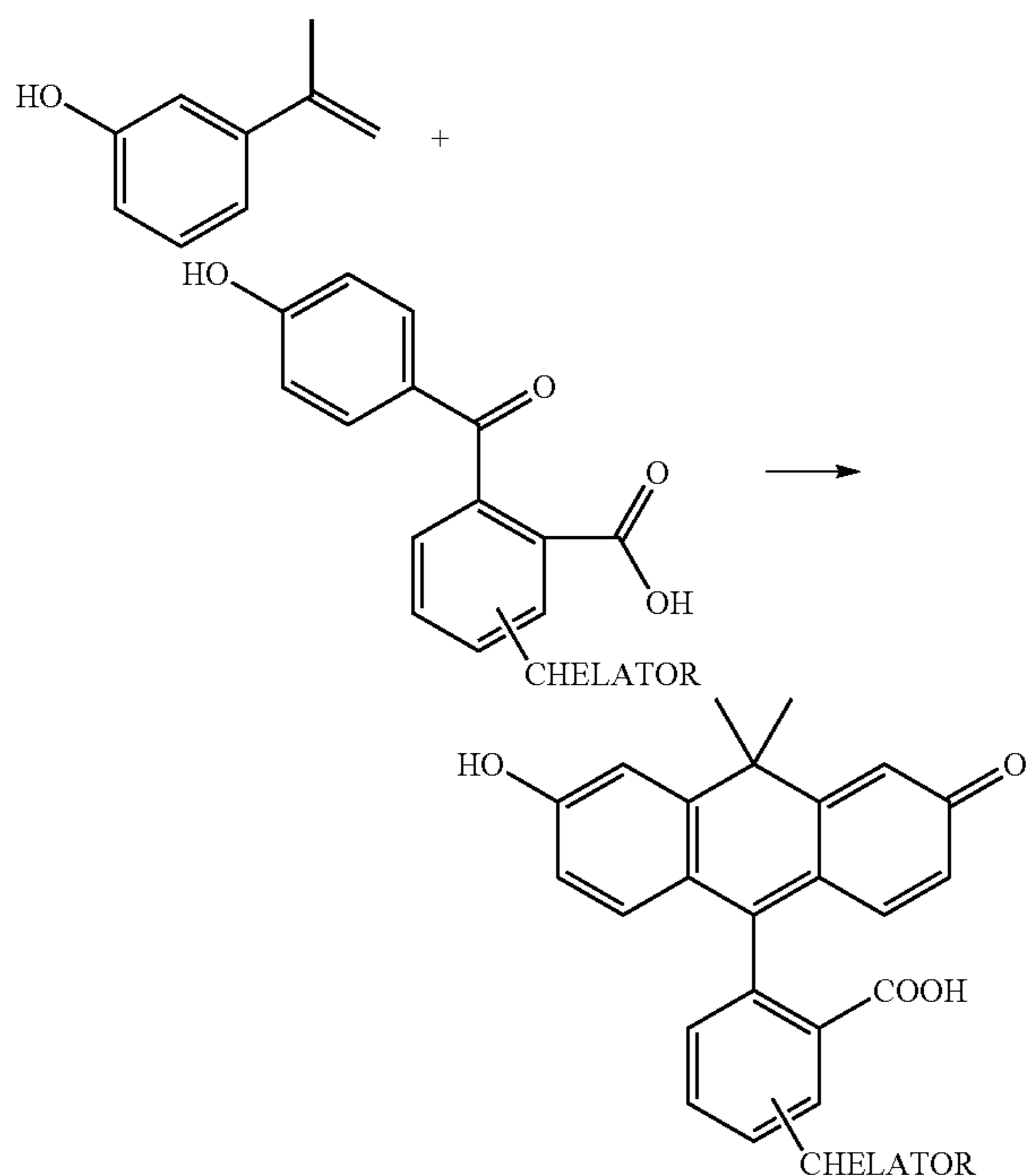
Scheme 4 (For clarity all the substituents are not shown)
