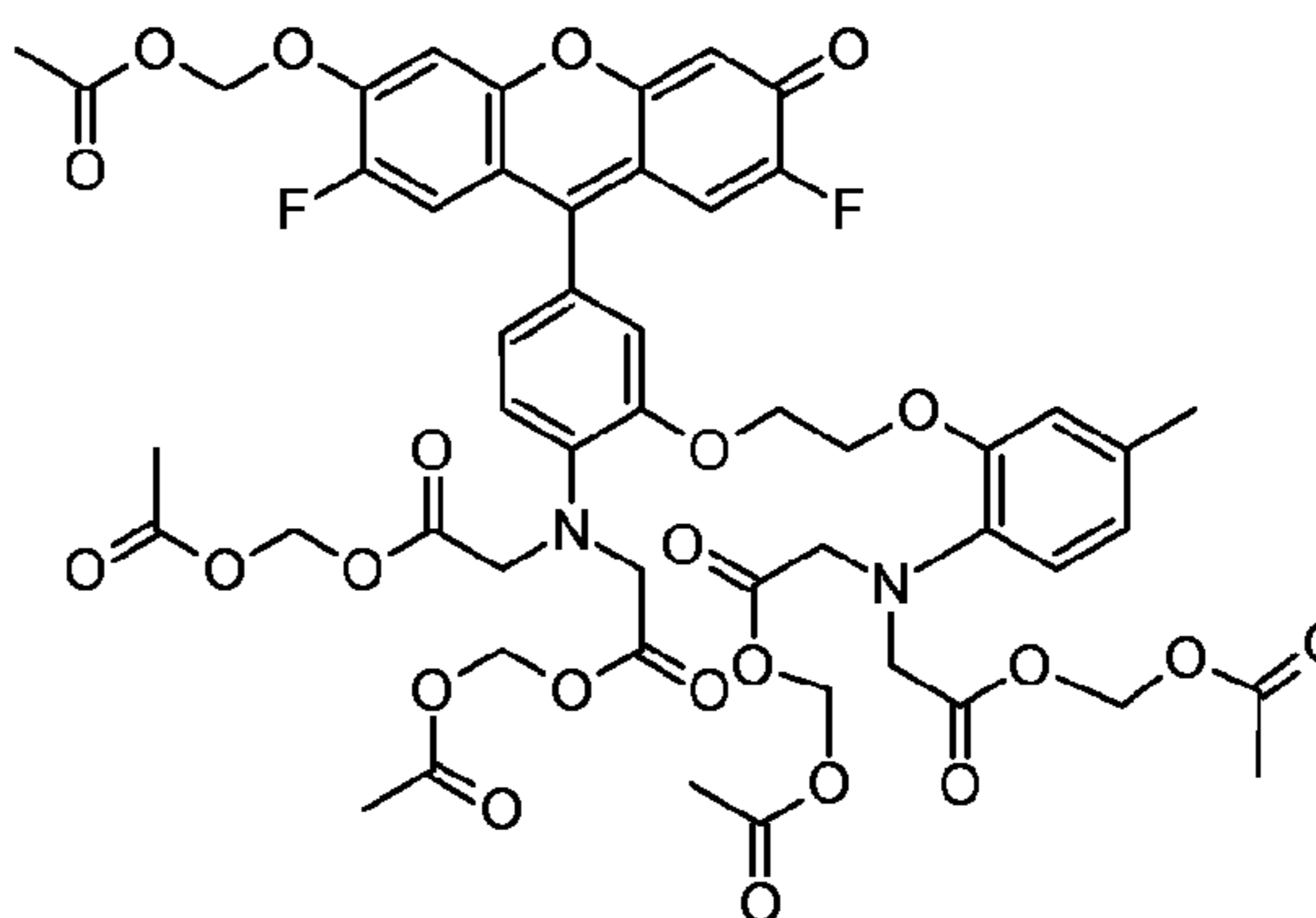
Fluo-4 AM
