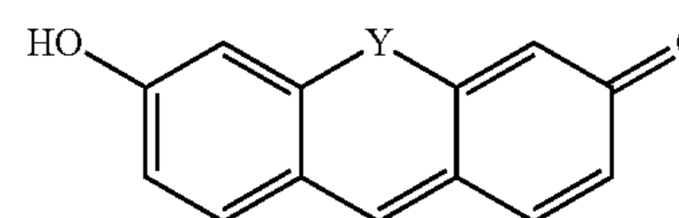
Fluorescein
