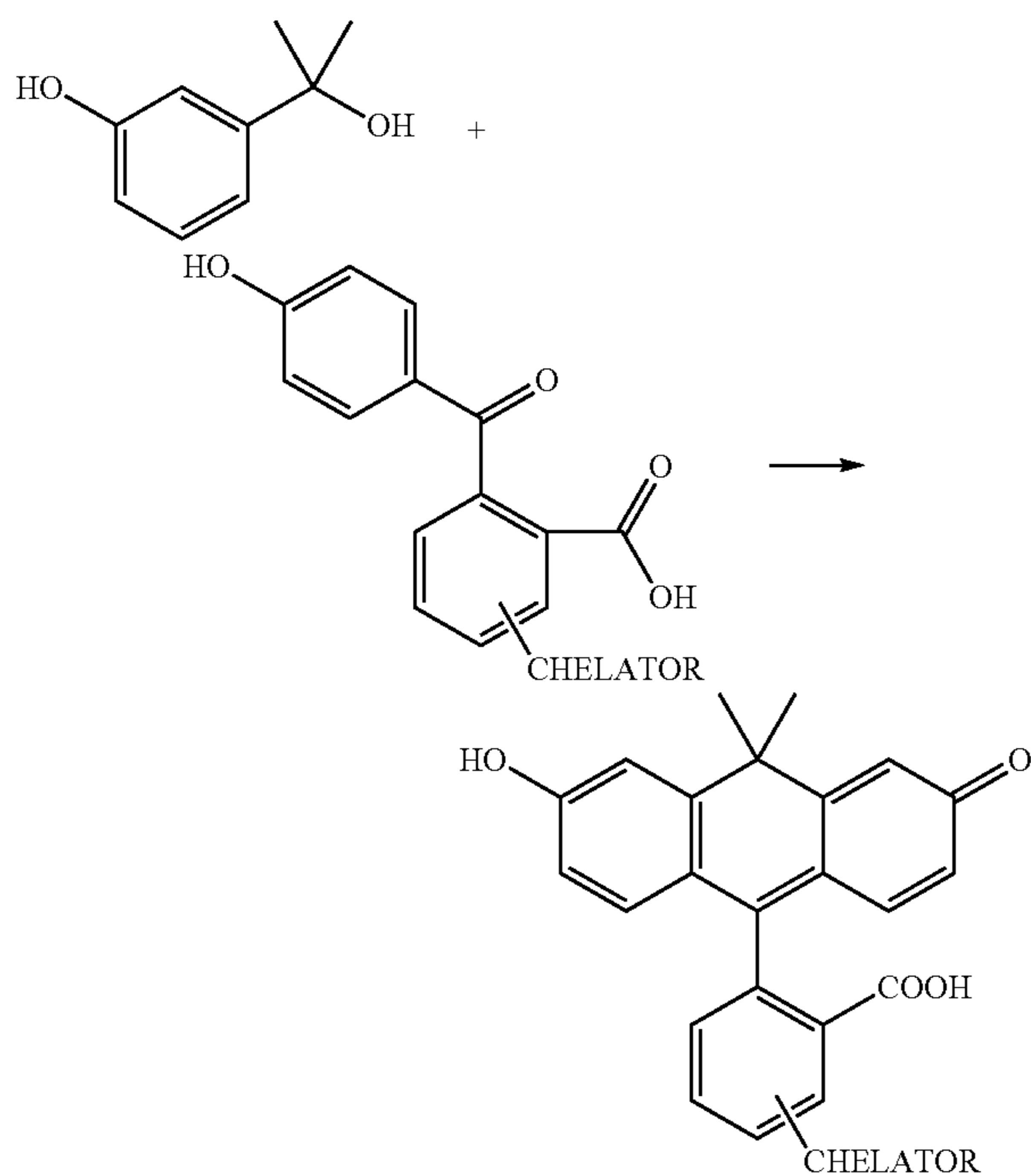
Scheme 3 (For clarity all the substituents are not shown)
