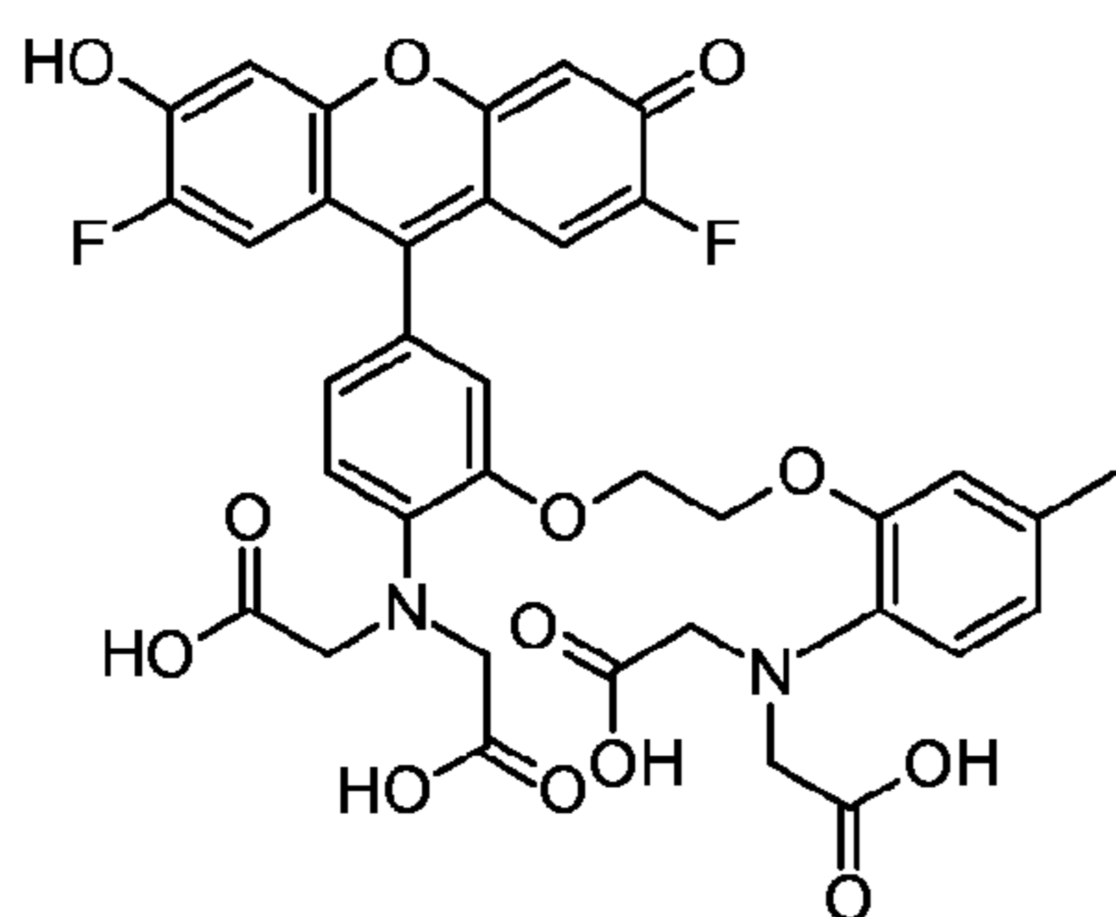
Fluo-4
