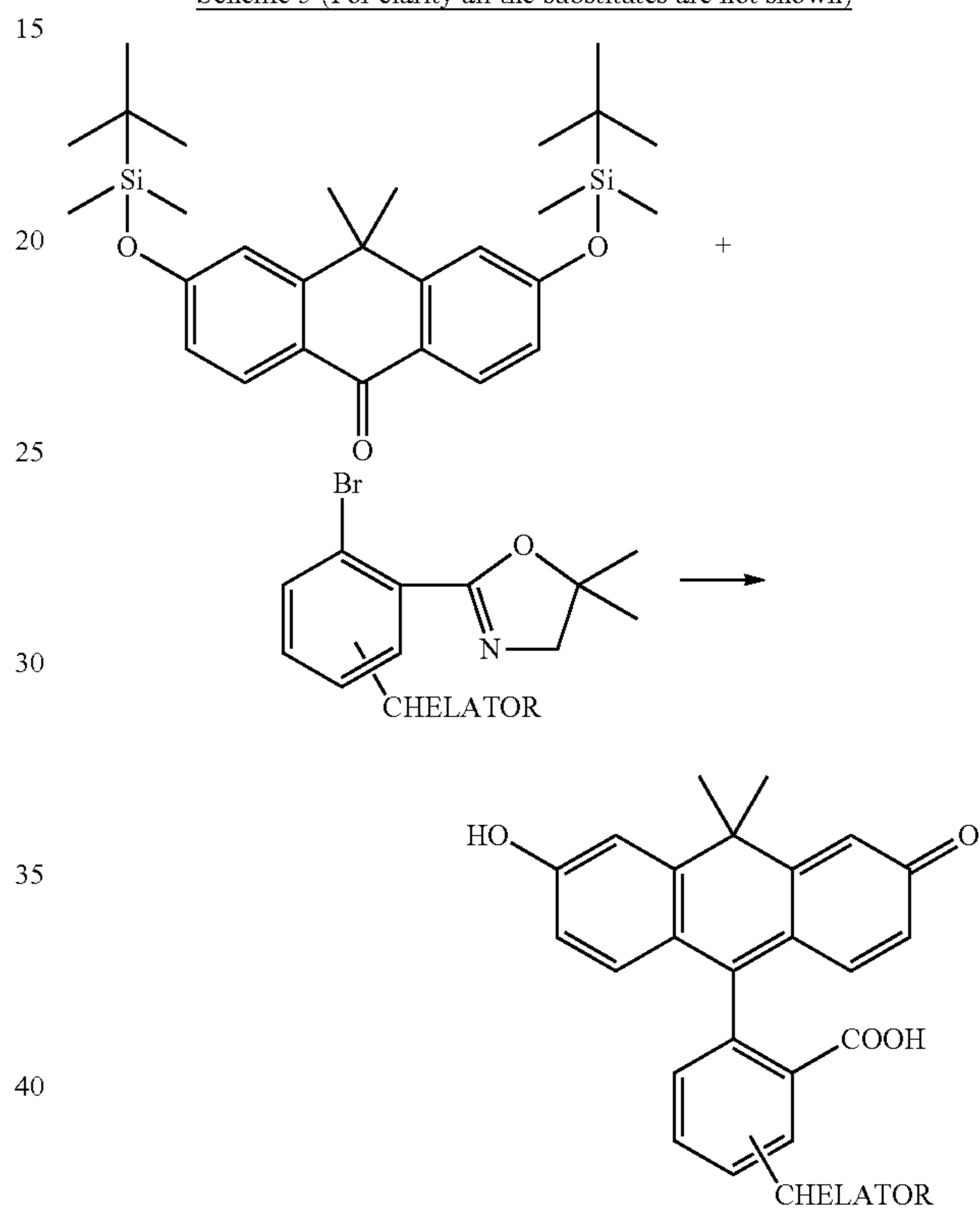
Scheme 5 (For clarity all the substituents are not shown)
