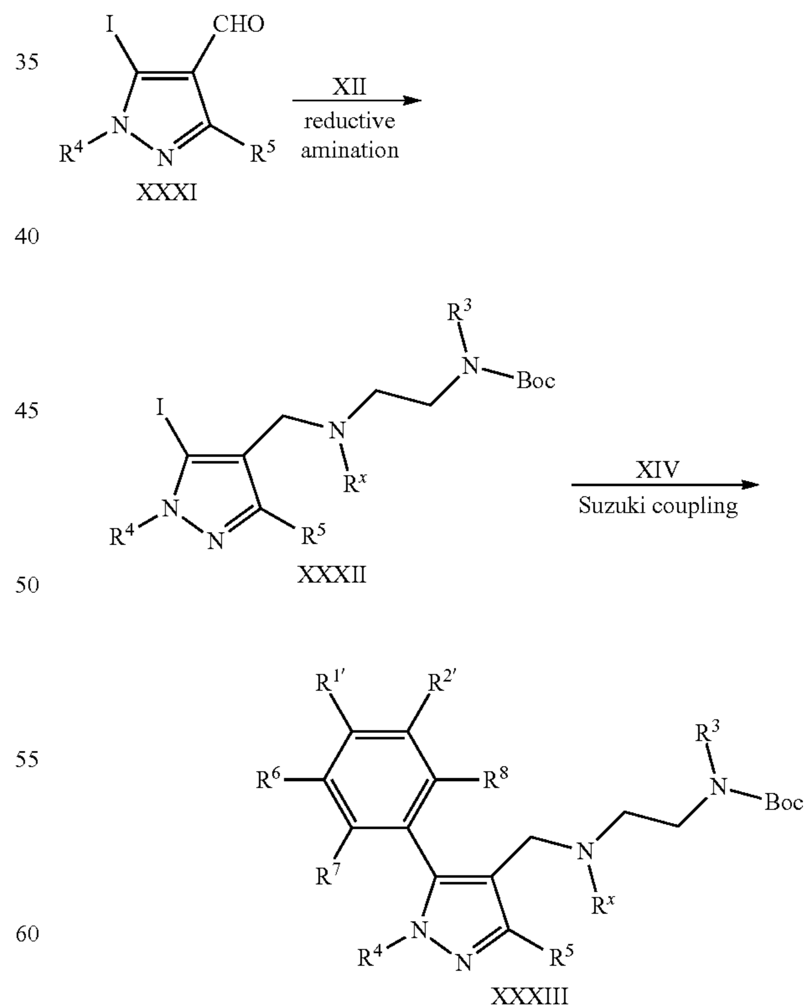
Scheme 5
