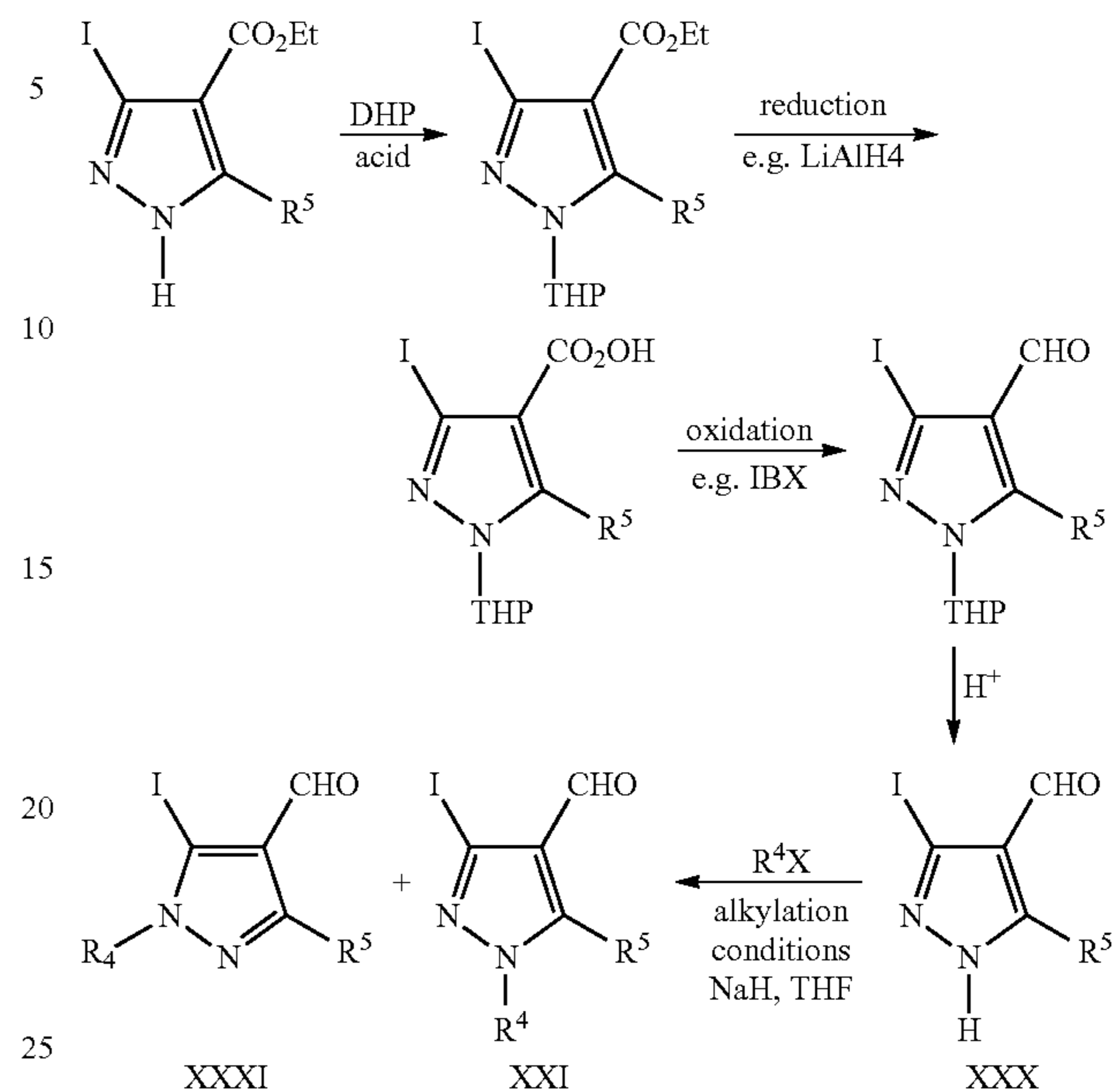
Scheme 4
