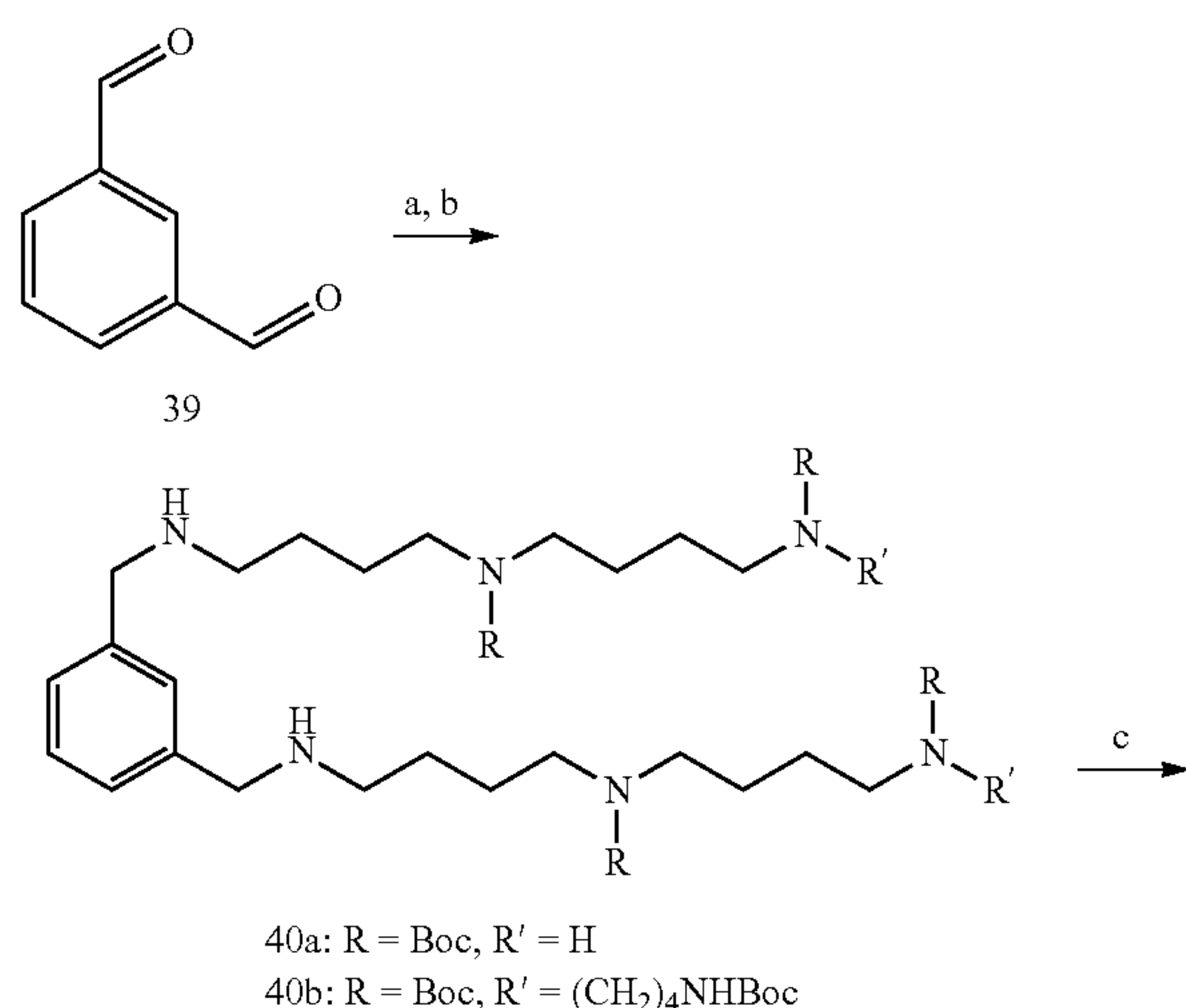
Scheme 2. a Synthesis of 34a and 34b
