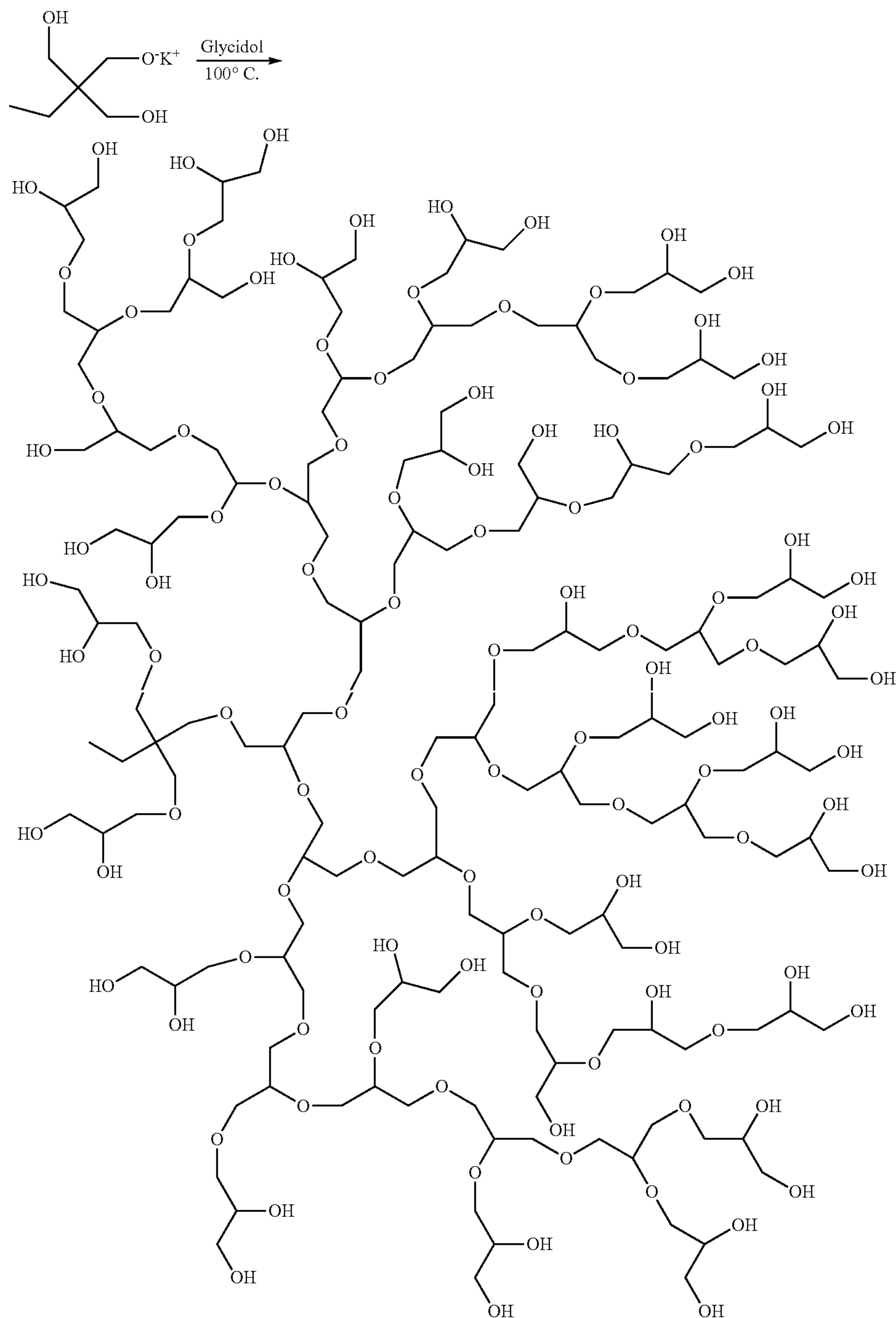
Scheme I. Synthesis of hyperbranched polyglycerol
