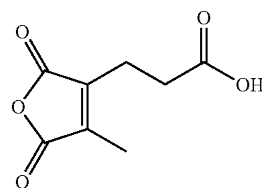
2-propionic-3-methylmaleic anhydride
