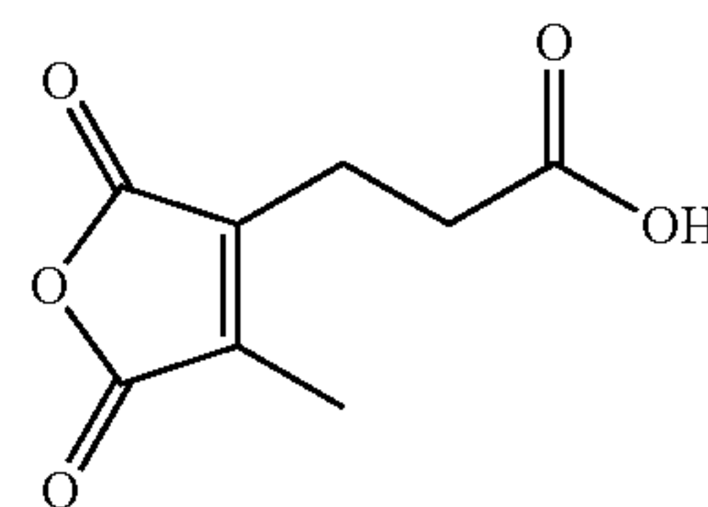
2-propionic-3-methylmaleic anhydride
