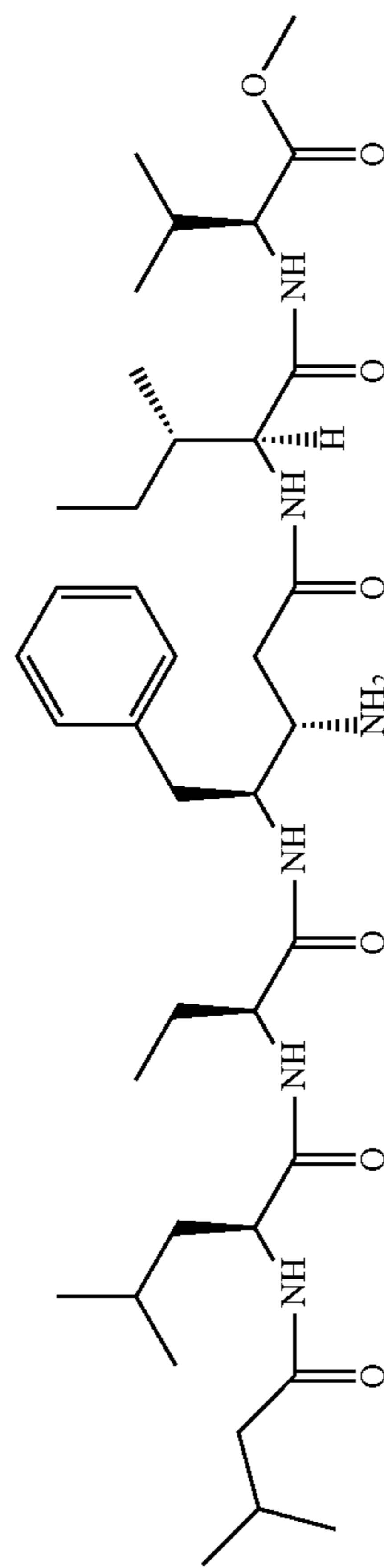
Methyl (S)-2-((2S,3S)-2-((3S,4S)-3-amino-4-[(S)-4-methyl-2-(3-methylbutyrylamino)pentanoylamino]-5-phenylpentanoylamino)-3-methylbutyrate
