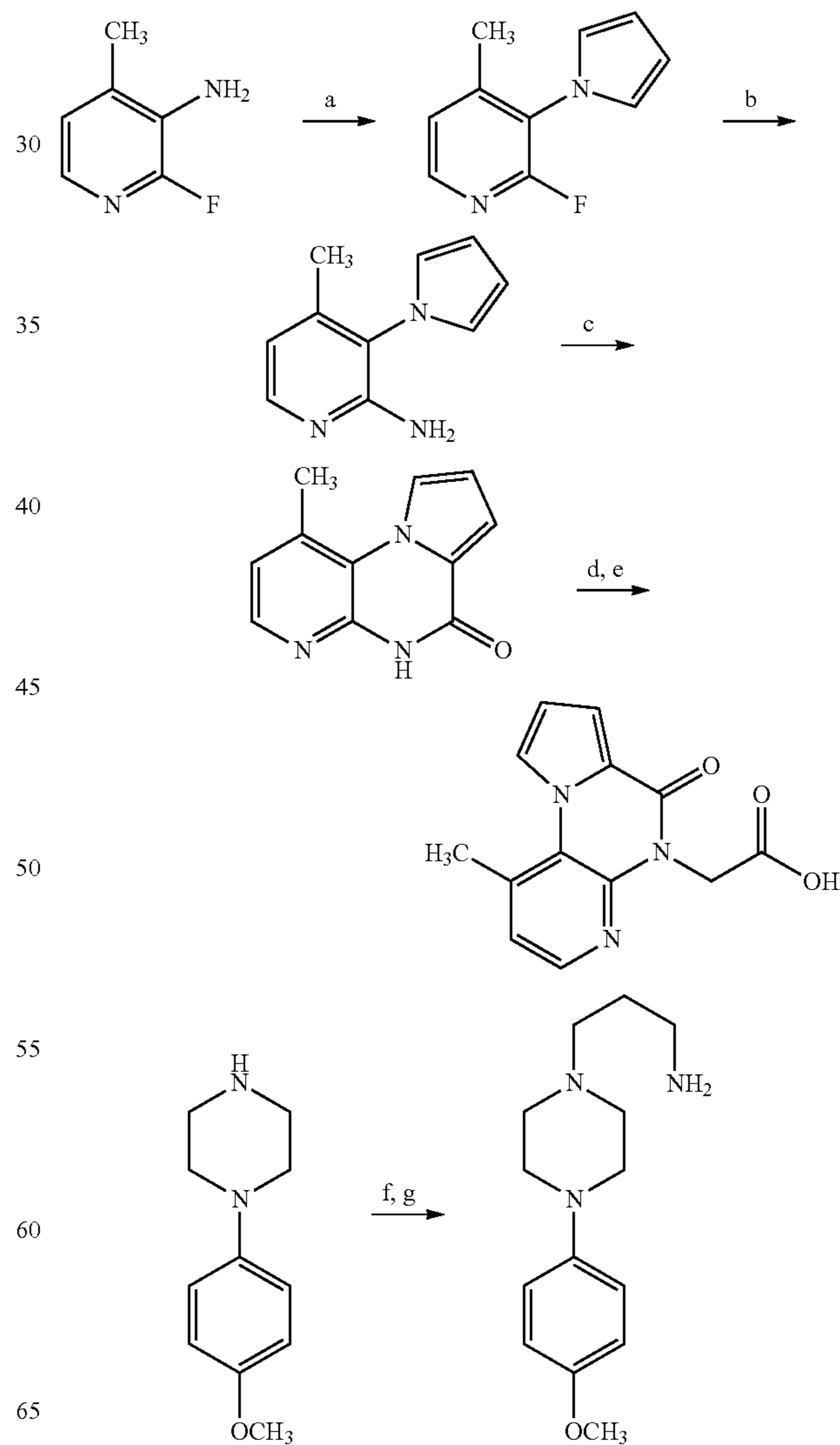
SCHEME 1
