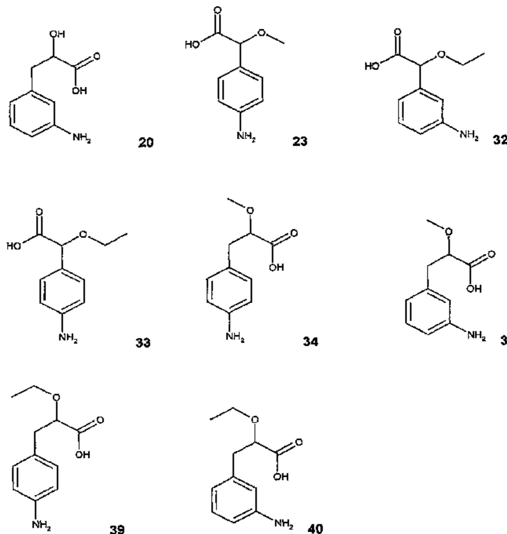
Structure of compounds 20, 23, 32, 33, 34, 35, 39, 40
