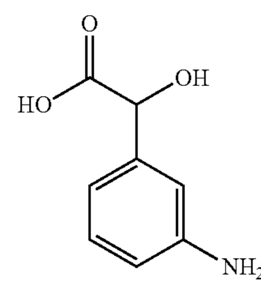
(R,S) 2-hydroxy-2-(3-aminophenyl)acetic acid
