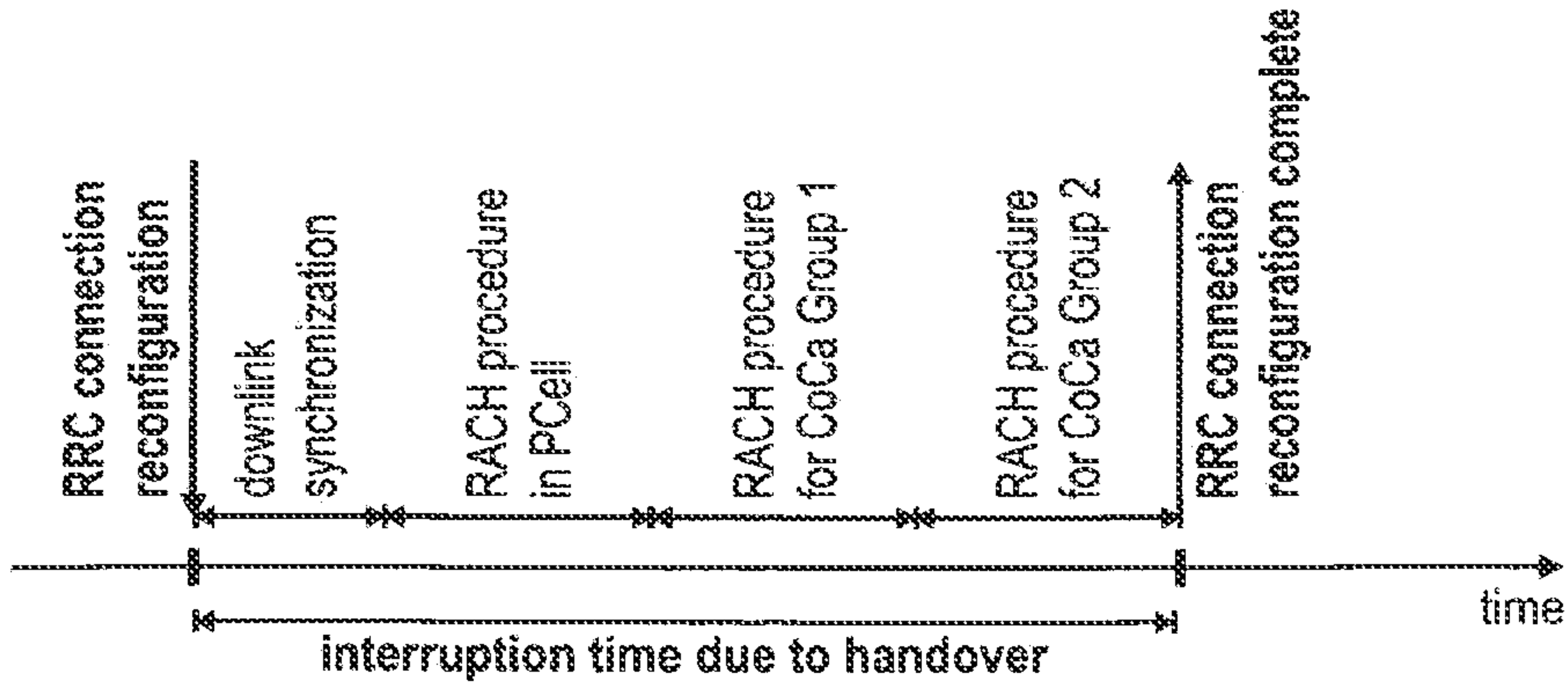
Fig. 10 (PRIOR ART)
