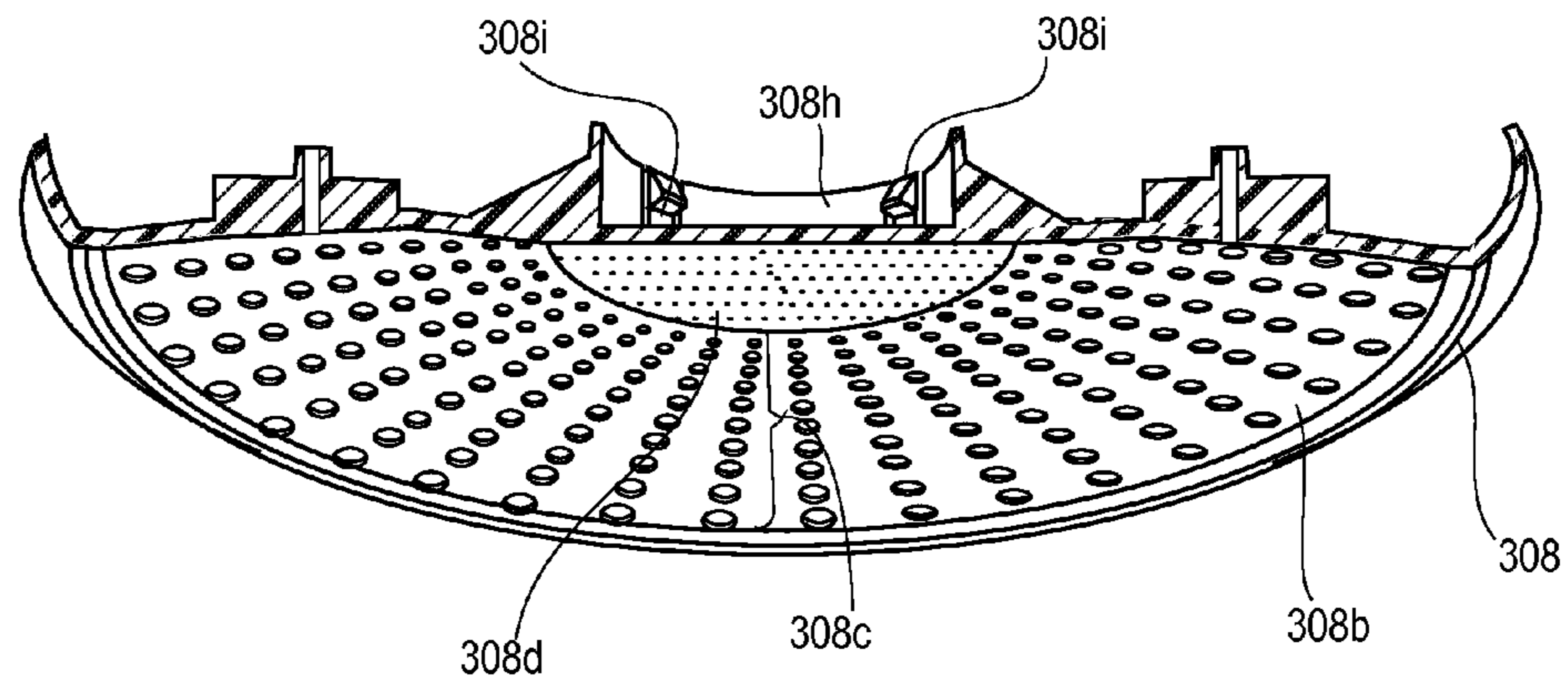
FIG. 3D
