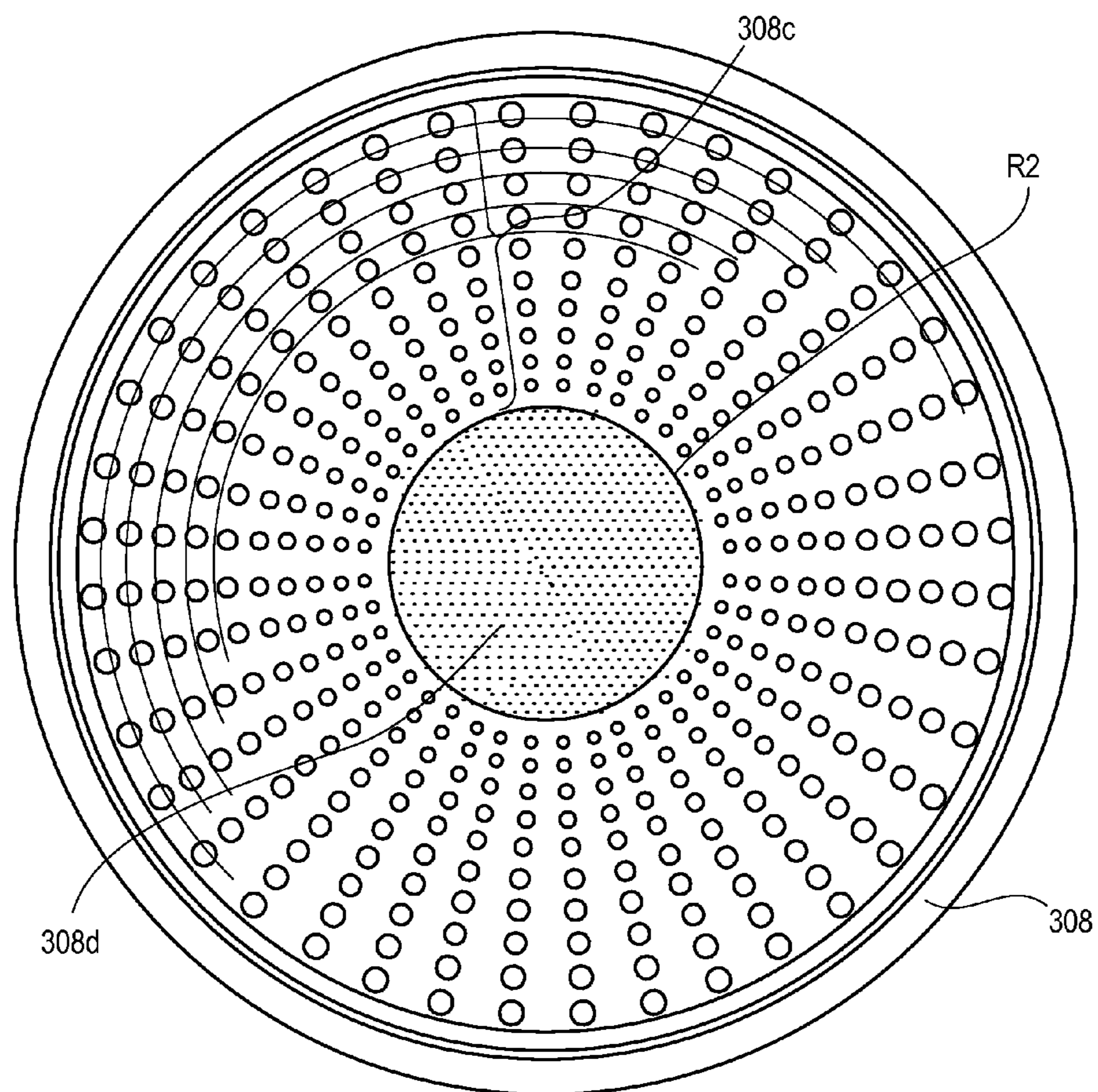
FIG. 3D
