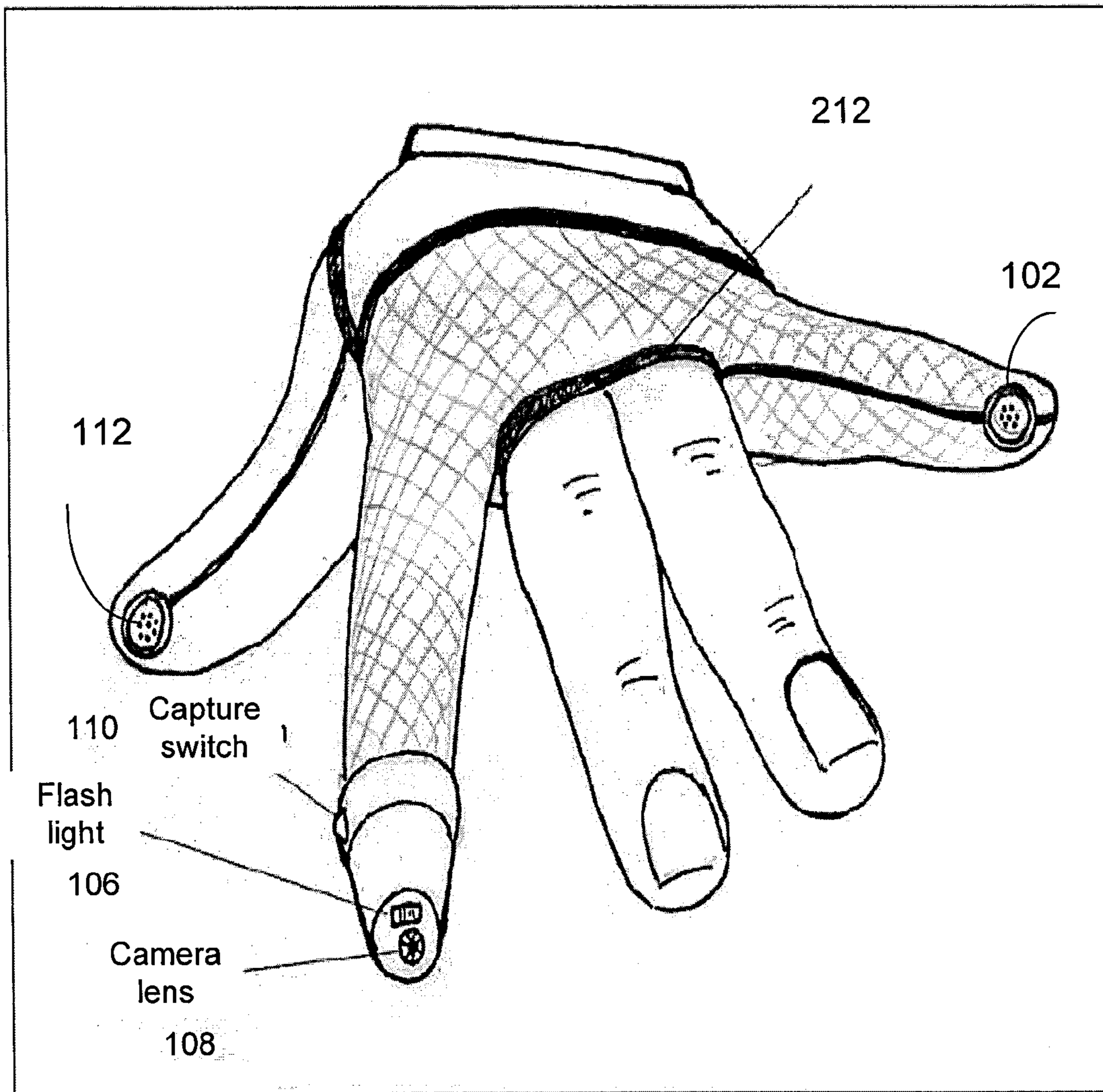
GLOVE TOP VIEW
