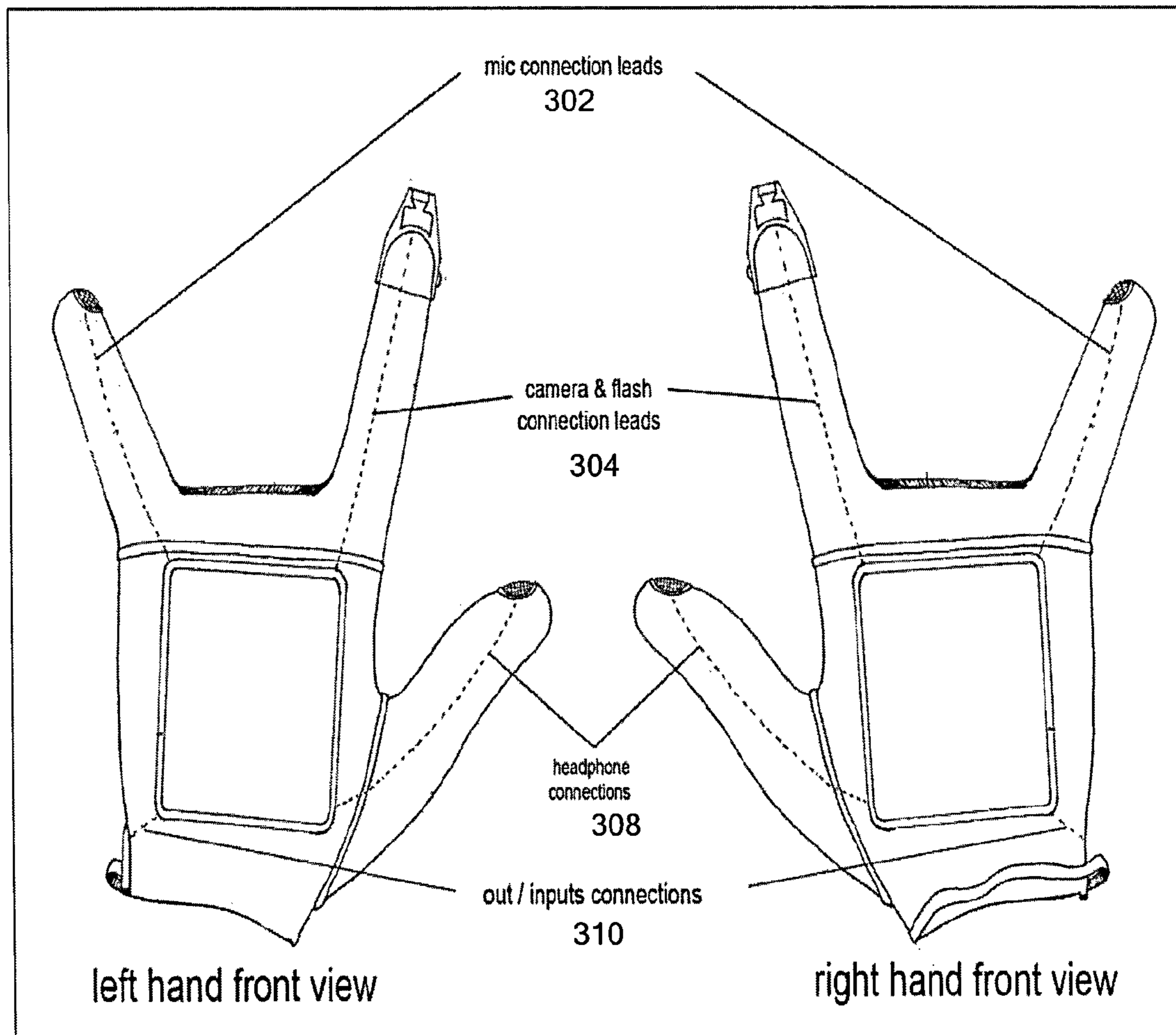
GLOVE FRONT VIEWS AND CONNECTIONS
